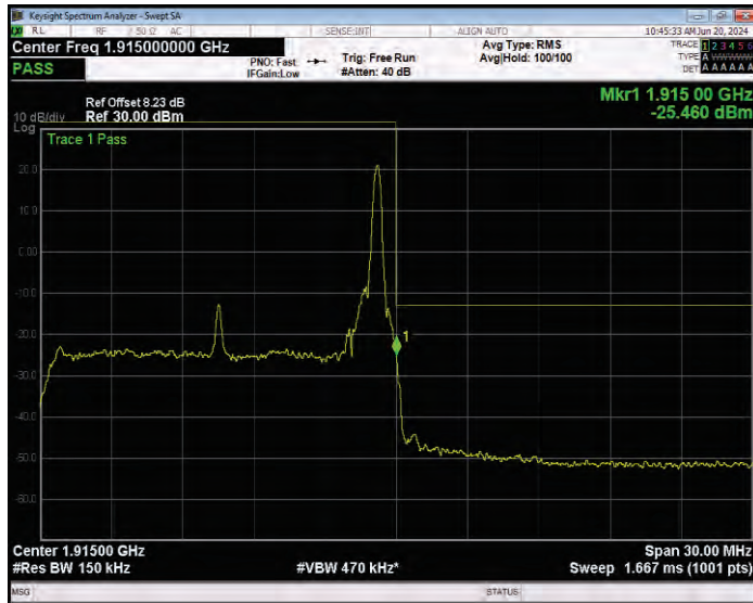
Band25 QPSK BW=15MHz Channel=26615 RB Size=75 Position=#0 Normal
