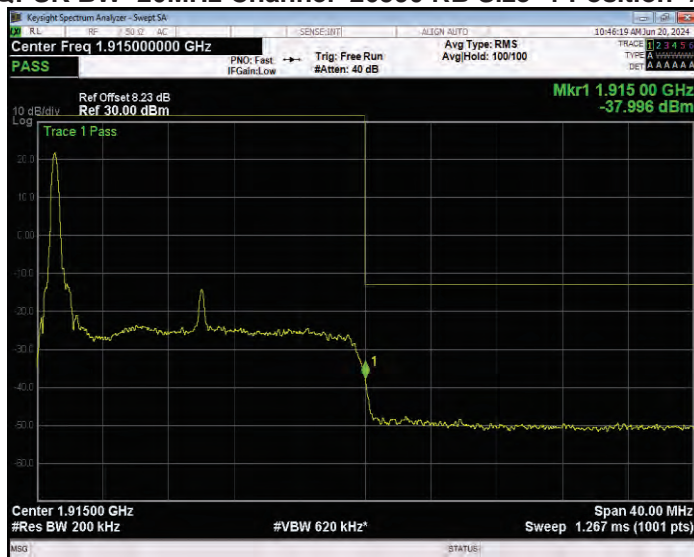
Band25 QPSK BW=20MHz Channel=26590 RB Size=1 Position=#Max Normal
