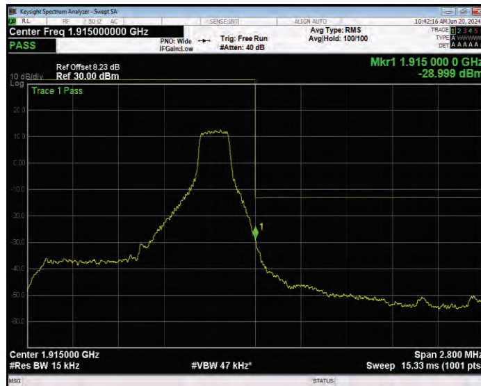
Band25 QPSK BW=1.4MHz Channel=26683 RB Size=6 Position=#0 Normal
