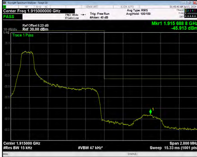
Band25 QPSK BW=1.4MHz Channel=26683 RB Size=1 Position=#Max Extended
