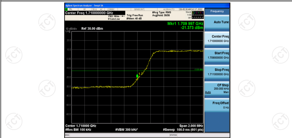
Band66-5MHz-16QAM-132647-25RB#0
