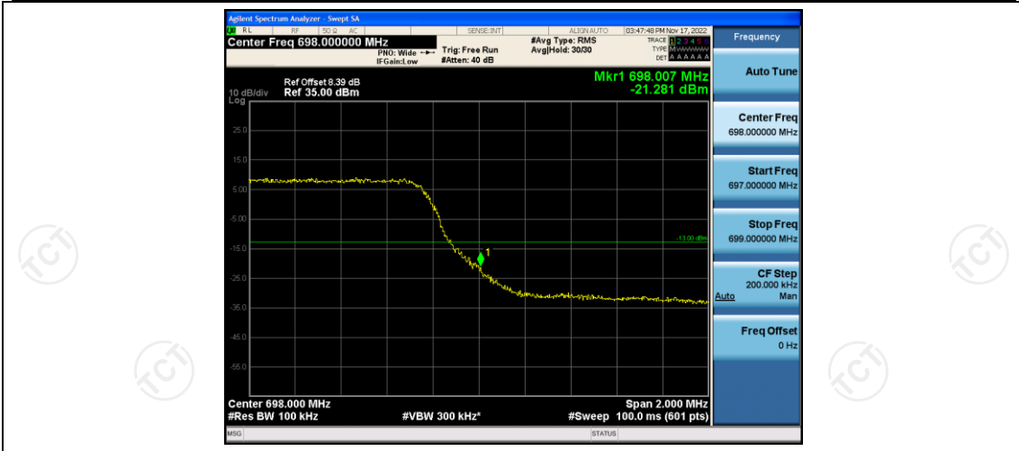
Band71-5MHz-16QAM-133147-25RB#0
