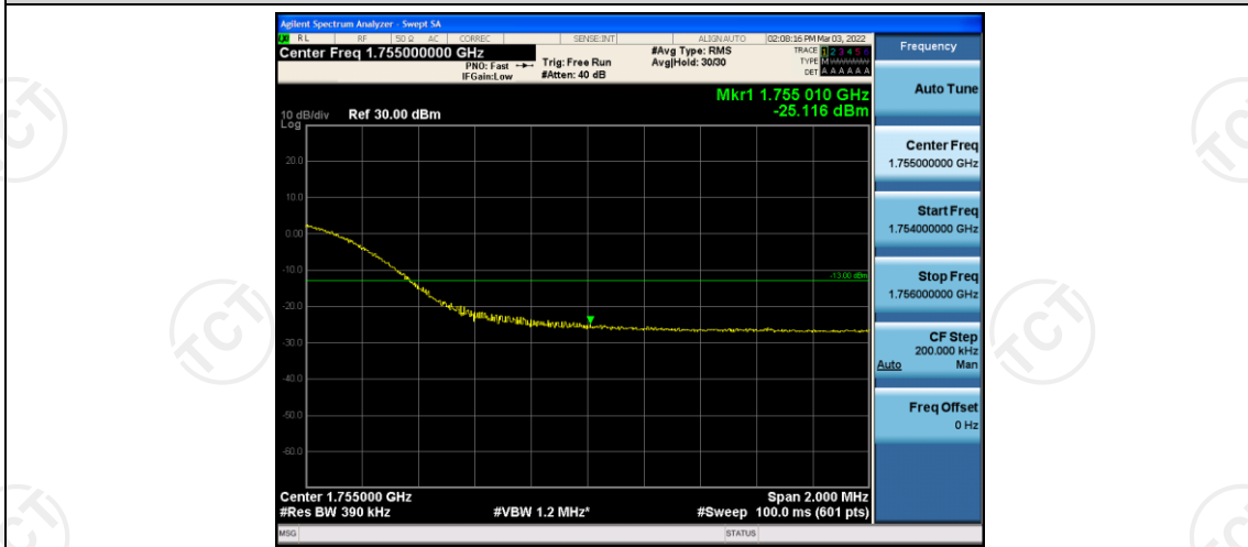
Band4-20MHz-16QAM-20300-100RB#0
