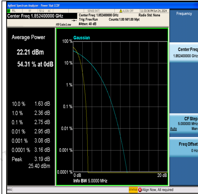
Band2-9262-PASS
