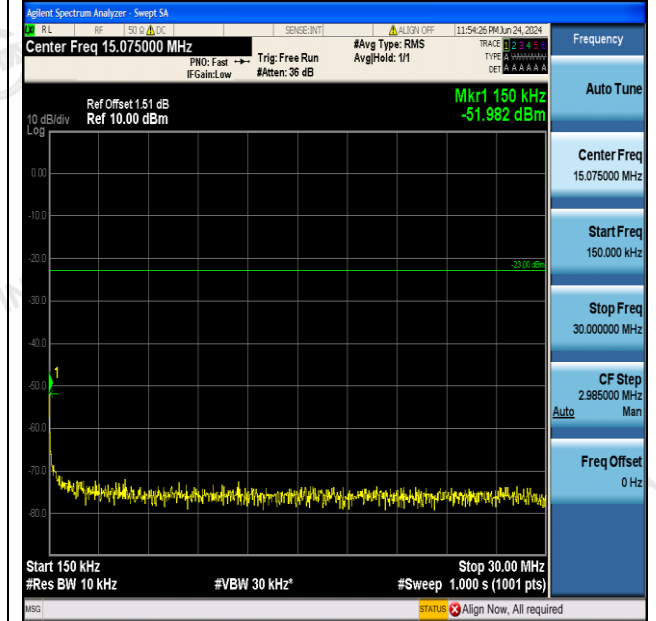
Band5-4233-0.15~30MHz-PASS
