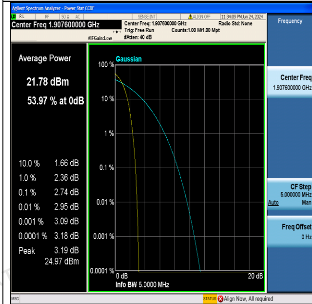
Band2-9538-PASS
