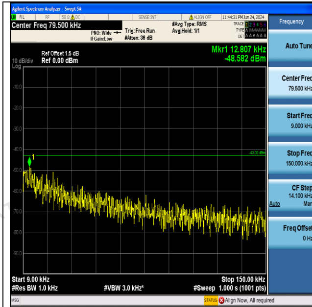
Band2-9262-0.009~0.15MHz-PASS
