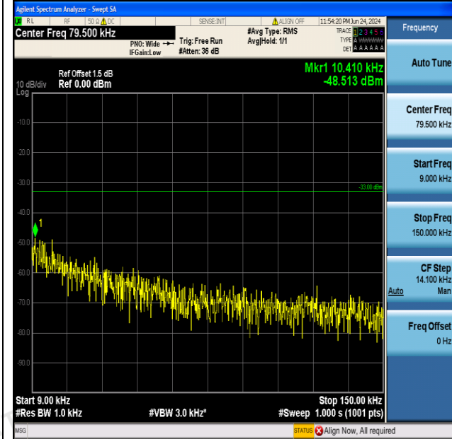
Band5-4233-0.009~0.15MHz-PASS
