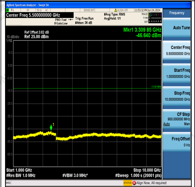
Band5-4132-1000~10000MHz-PASS
