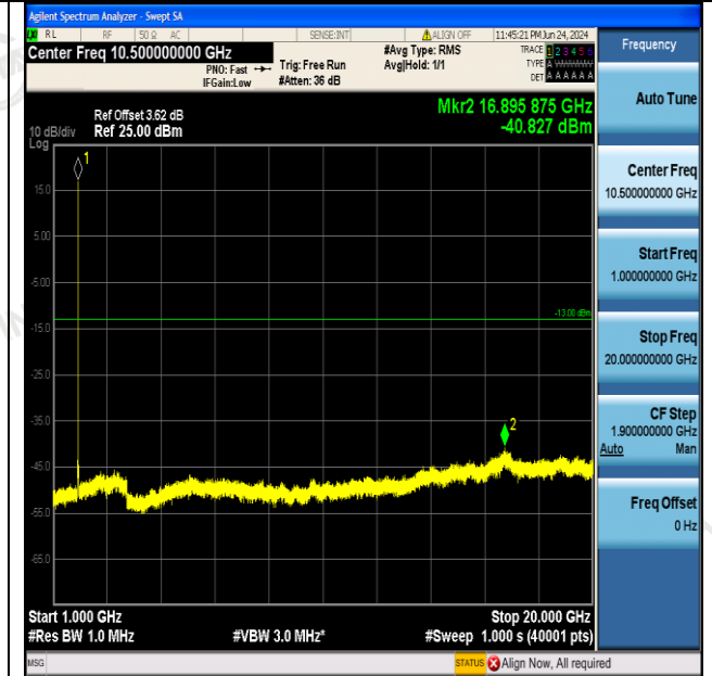
Band2-9400-1000~20000MHz-PASS
