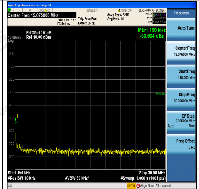
Band2-9538-0.15~30MHz-PASS
