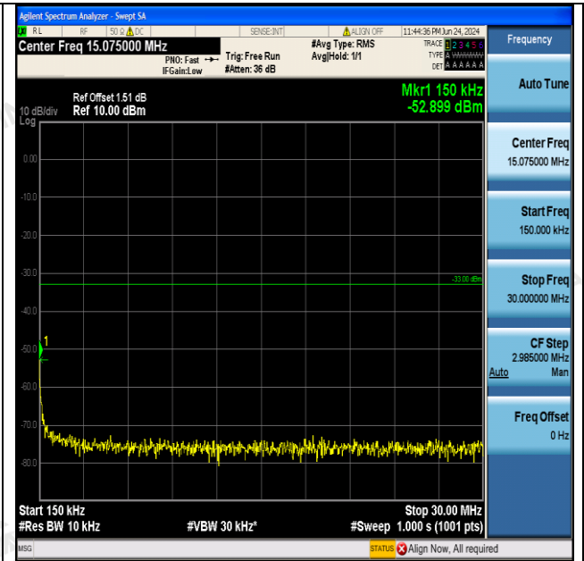
Band2-9262-0.15~30MHz-PASS
