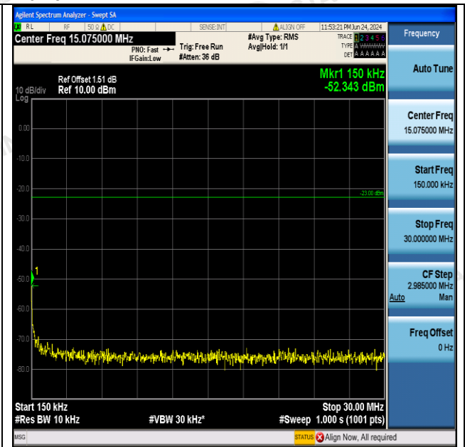
Band5-4132-0.15~30MHz-PASS
