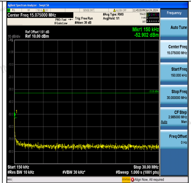
Band2-9400-0.15~30MHz-PASS
