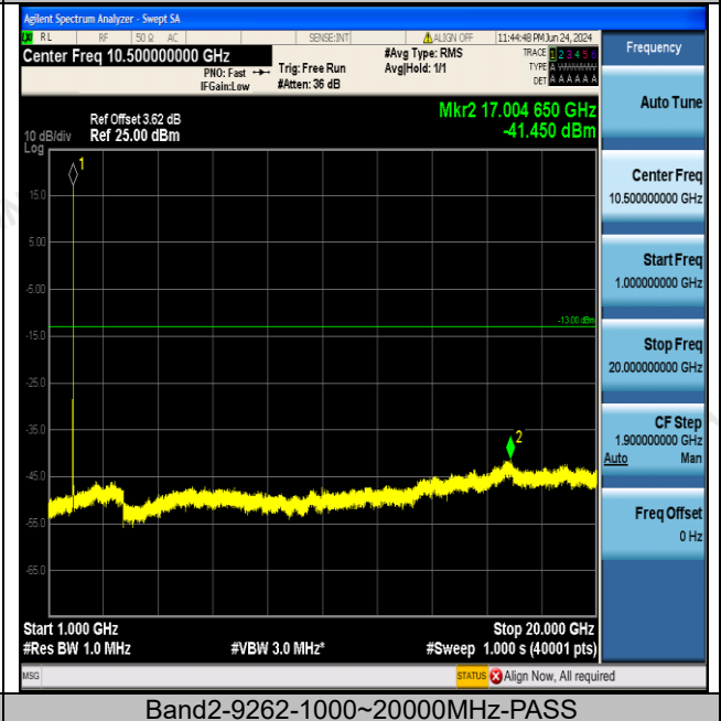
Band2-9262-1000~20000MHz-PASS
