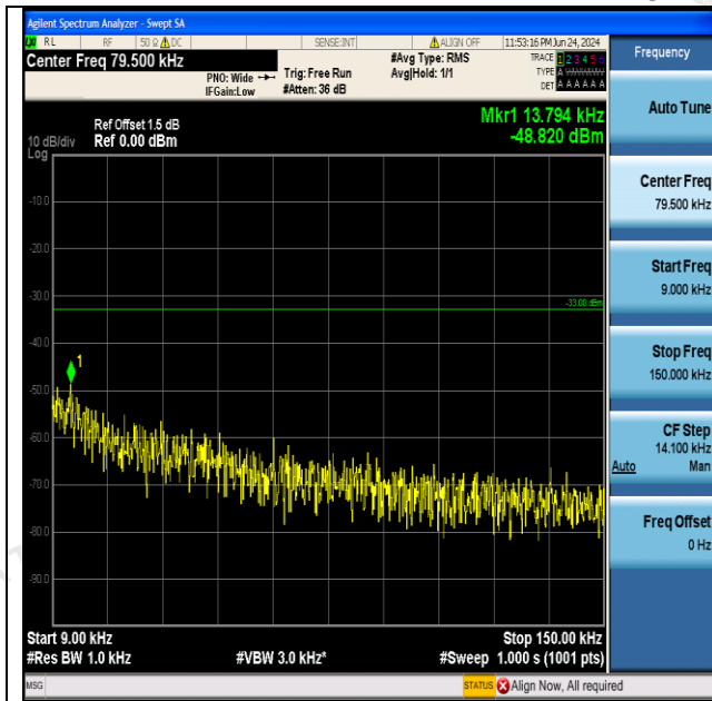
Band5-4132-0.009~0.15MHz-PASS
