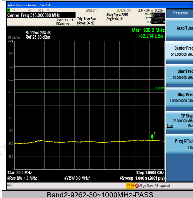
Band2-9262-30~1000MHz-PASS
