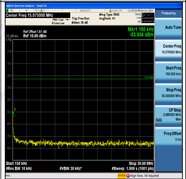
Band5-4182-0.15~30MHz-PASS
