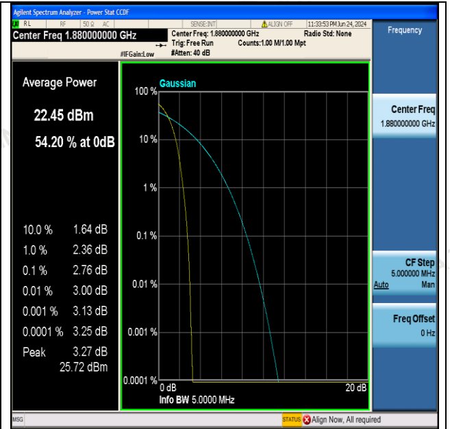
Band2-9400-PASS
