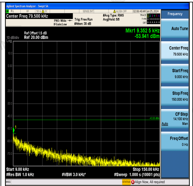
GPRS1900-512-0-0.009~0.15MHz-PASS
