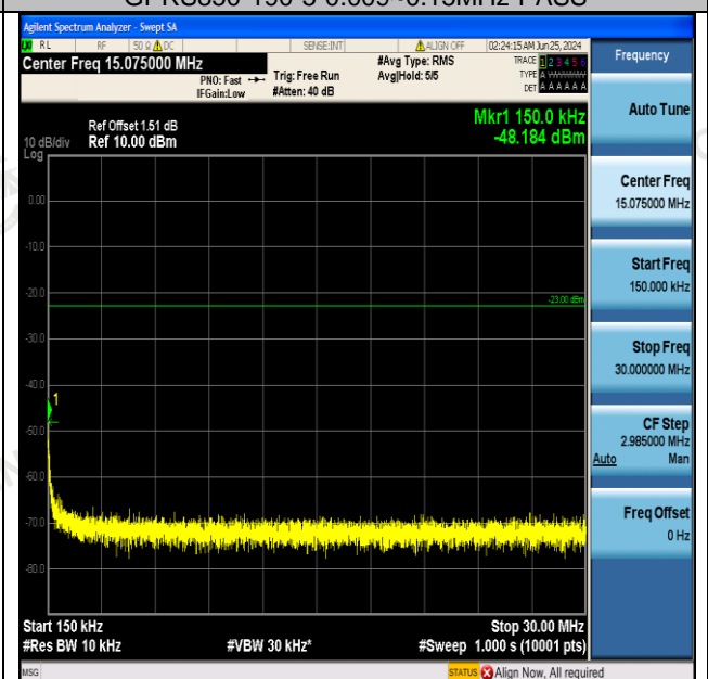
GPRS850-190-5-0.15~30MHz-PASS
