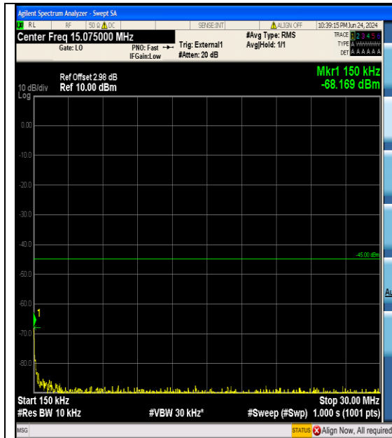
Band41_15MHz_16QAM_39725_75RB#0_0.15~30_0.15~30
