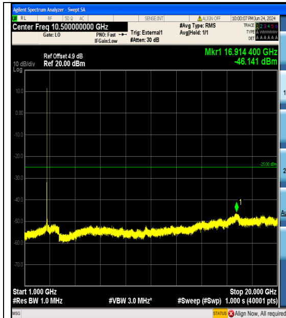
Band41_5MHz_16QAM_41565_25RB#0_1000~ 20000_1000~20000
