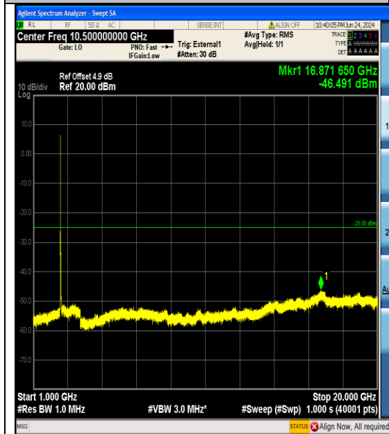
Band41_15MHz_16QAM_39725_75RB#0_1000~20000_1000~20000
