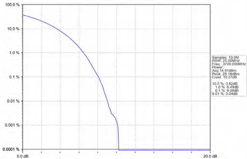
n78a 15kHz SISO NTN 40MHz CP-OFDM 64 QAM 3720MHz Outer Full
