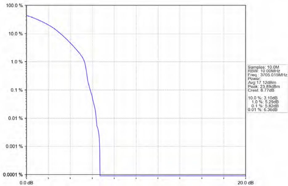
n78a 30kHz SISO NTN 10MHz DFT-s-OFDM 64 QAM 3705.015MHz Outer Full
