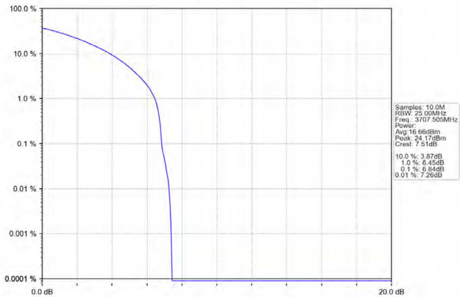
n78a 30kHz SISO NTN 15MHz CP-OFDM 64 QAM 3707.505MHz Outer Full
