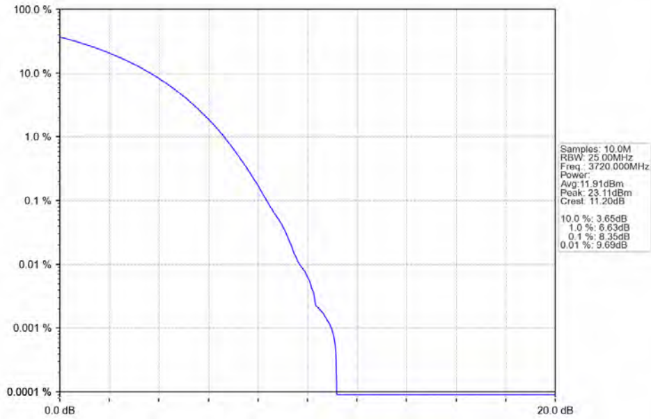
n78a 15kHz SISO NTN 40MHz CP-OFDM 256 QAM 3720MHz Outer Full
