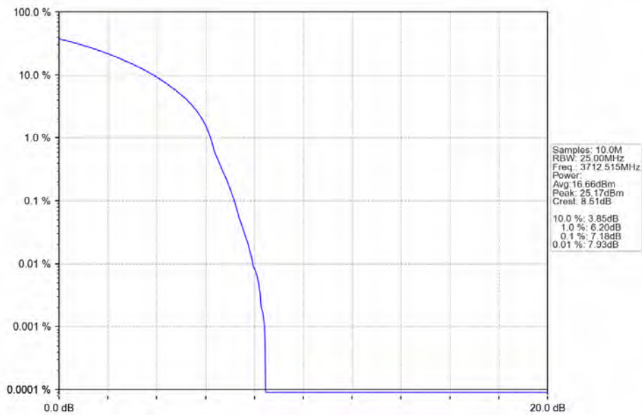
n78a 30kHz SISO NTN 25MHz CP-OFDM 64 QAM 3712.515MHz Outer Full
