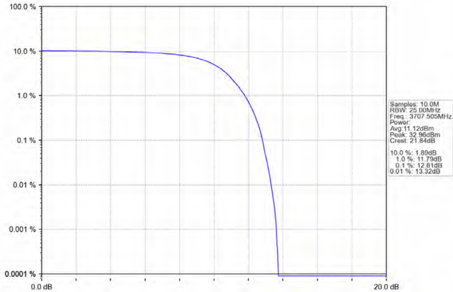
n78a_30kHz_SISO_NTNV_15MHz_DFT-s-OFDM_PI/2_BPSK_3707.505MHz_Outer_Full
