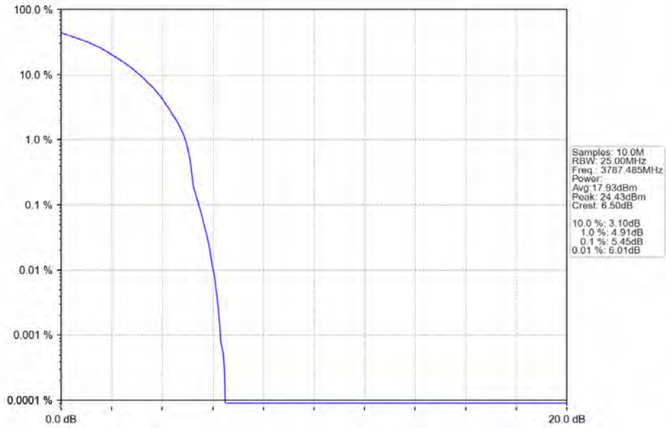
n78a 30kHz SISO NTN 25MHz DFT-s-OFDM 16 QAM 3787.485MHz Outer Full
