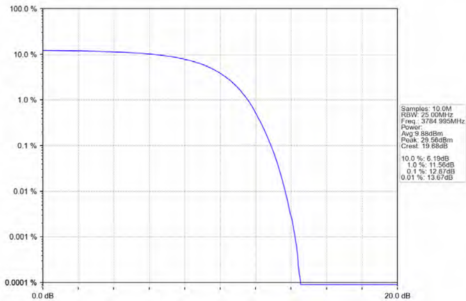
n78a 30kHz SISO NTN 30MHz DFT-s-OFDM QPSK 3784.995MHz Outer Full
