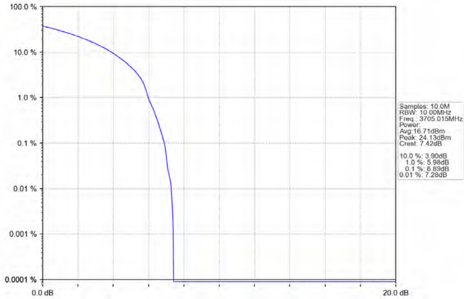
n78a 30kHz SISO NTN 10MHz CP-OFDM 16 QAM 3705.015MHz Outer Full
