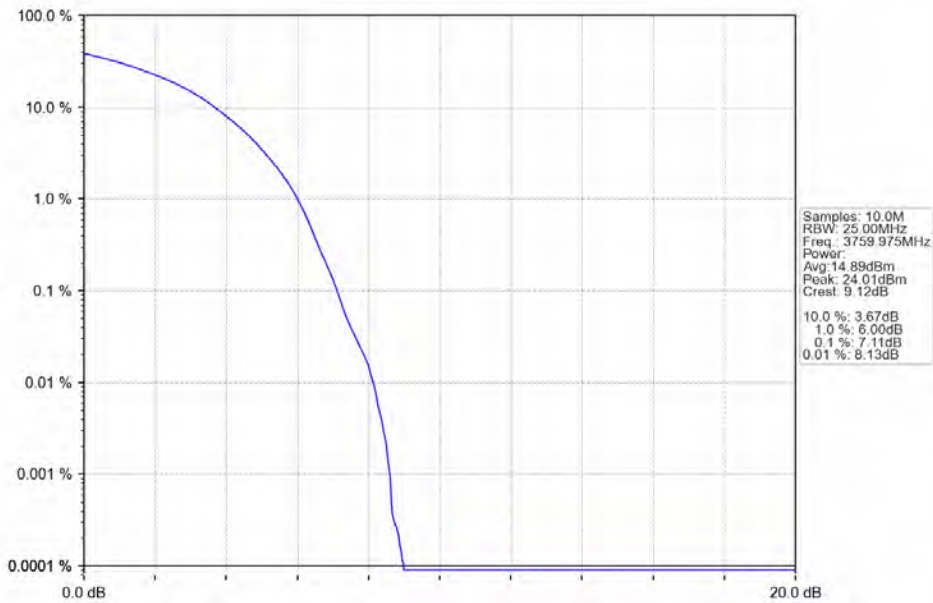
n78a 30kHz SISO NTN 80MHz DFT-s-OFDM QPSK 3759.975MHz Outer Full
