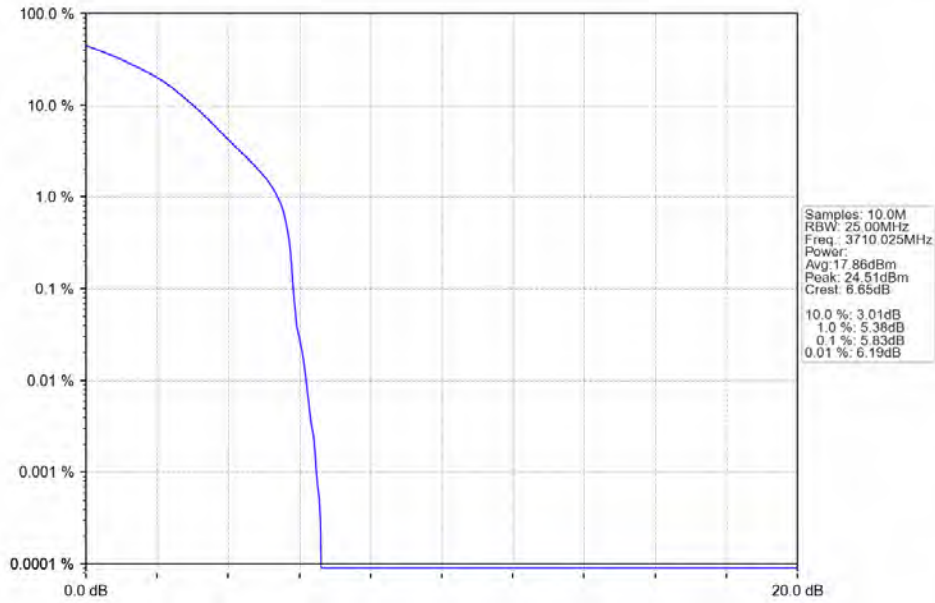
n78a 30kHz SISO NTN 20MHz DFT-s-OFDM 16 QAM 3710.025MHz Outer Full
