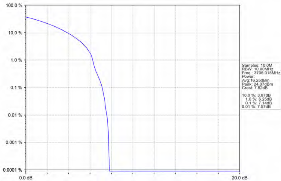
n78a 30kHz SISO NTN 10MHz CP-OFDM 64 QAM 3705.015MHz Outer Full
