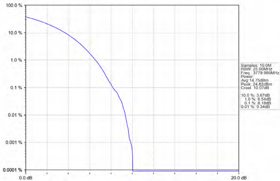
n78a 30kHz SISO NTN 40MHz CP-OFDM 64 QAM 3779.985MHz Outer Full
