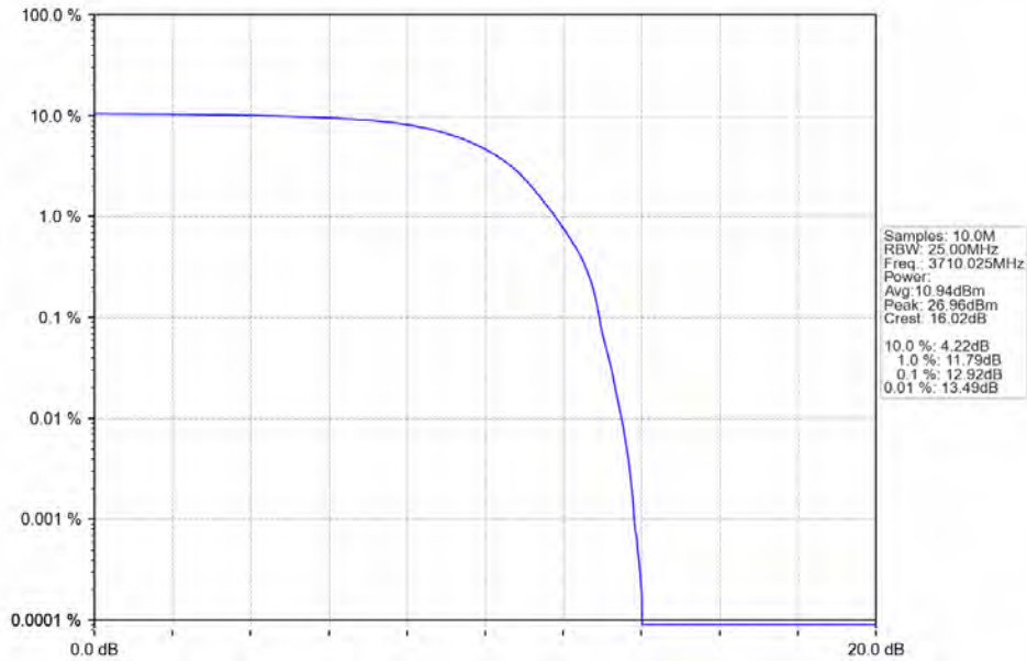
n78a_30kHz_SISO_NTNV_20MHz_DFT-s-OFDM_PI/2_BPSK_3710.025MHz_Outer_Full
