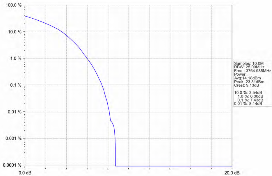
n78a 30kHz SISO NTN 70MHz DFT-s-OFDM 64 QAM 3764.985MHz Outer Full
