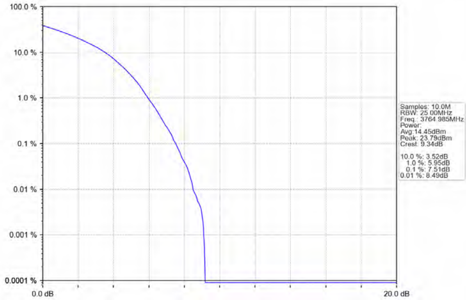
n78a 30kHz SISO NTN 70MHz DFT-s-OFDM 16 QAM 3764.985MHz Outer Full
