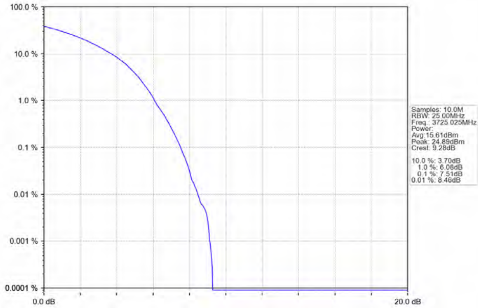
n78a 30kHz SISO NTN 50MHz DFT-s-OFDM 16 QAM 3725.025MHz Outer Full
