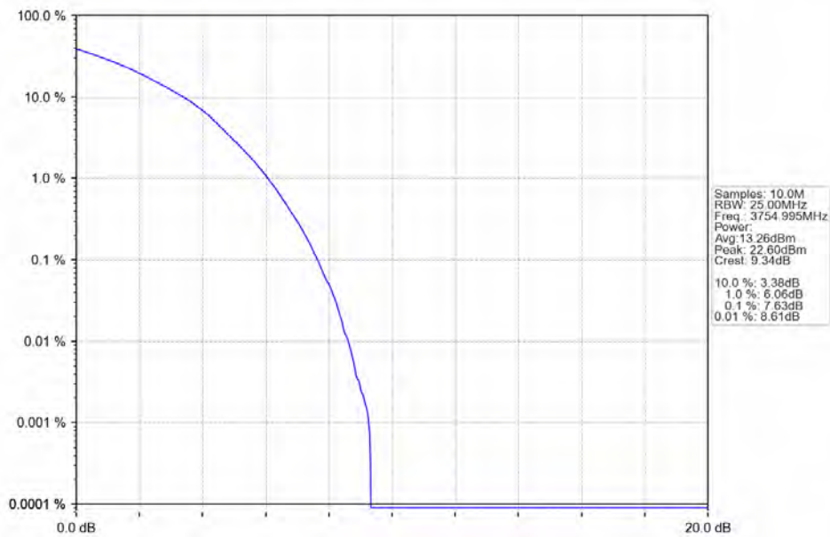
n78a 30kHz SISO NTN 90MHz DFT-s-OFDM 64 QAM 3754.995MHz Outer Full
