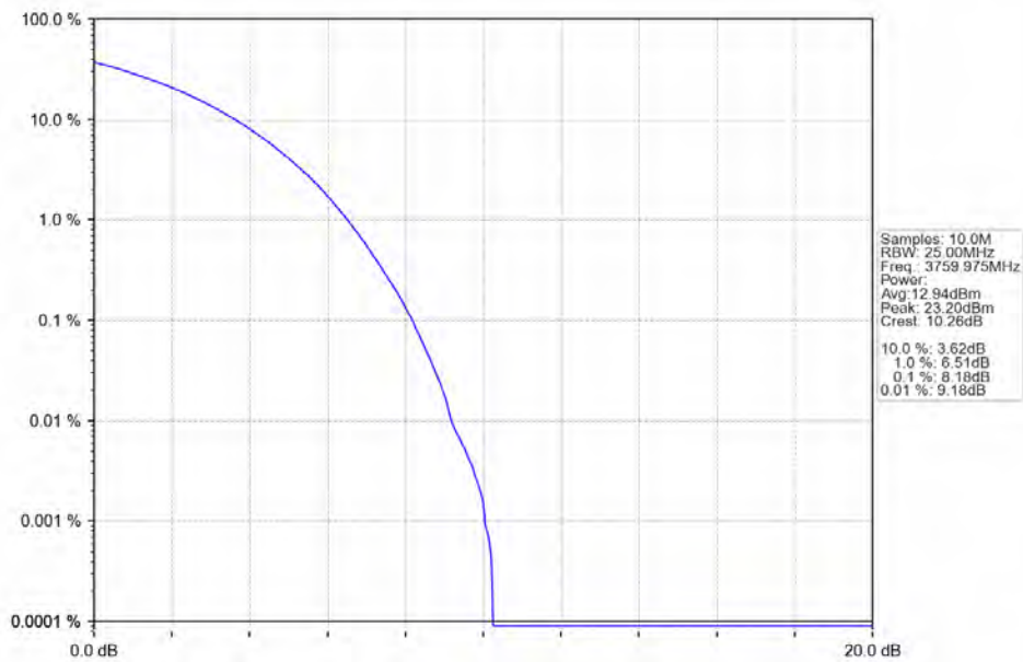
n78a 30kHz SISO NTV 80MHz CP-OFDM QPSK 3759.975MHz Outer Full
