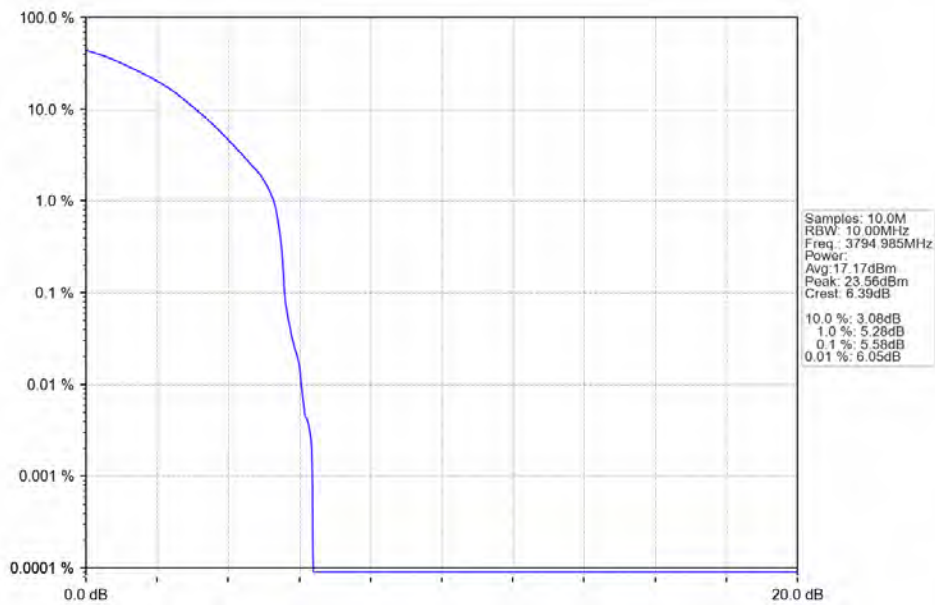
n78a 30kHz SISO NTN 10MHz DFT-s-OFDM 64 QAM 3794.985MHz Outer Full
