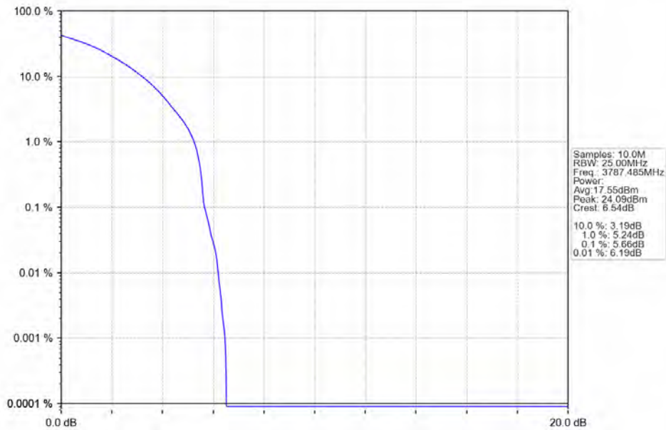
n78a 30kHz SISO NTN 25MHz DFT-s-OFDM 64 QAM 3787.485MHz Outer Full
