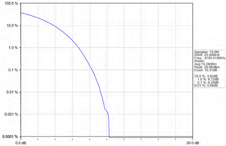
n78a 30kHz SISO NTN 40MHz CP-OFDM 16 QAM 3720.015MHz Outer Full
