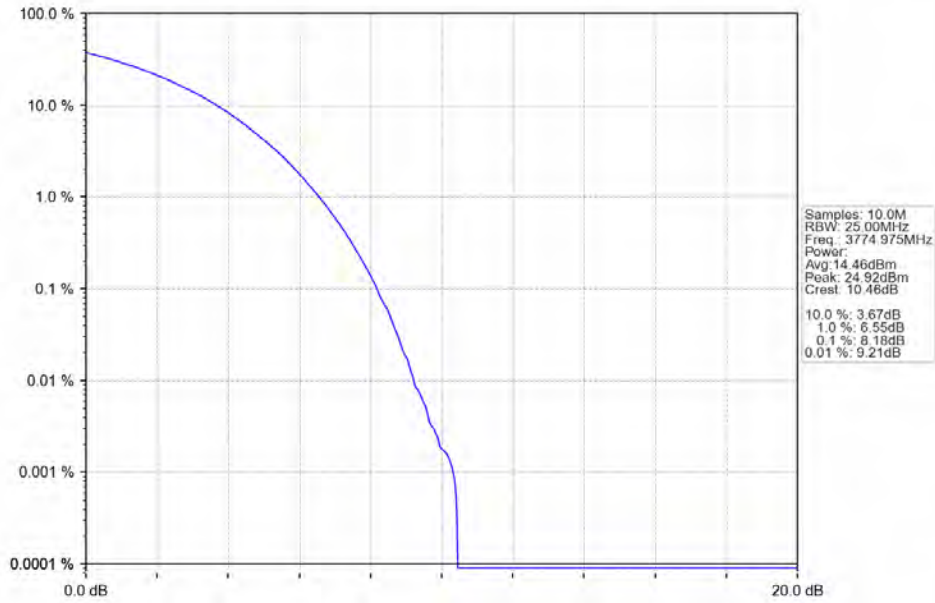
n78a 30kHz SISO NTN 50MHz CP-OFDM 16 QAM 3774.975MHz Outer Full
