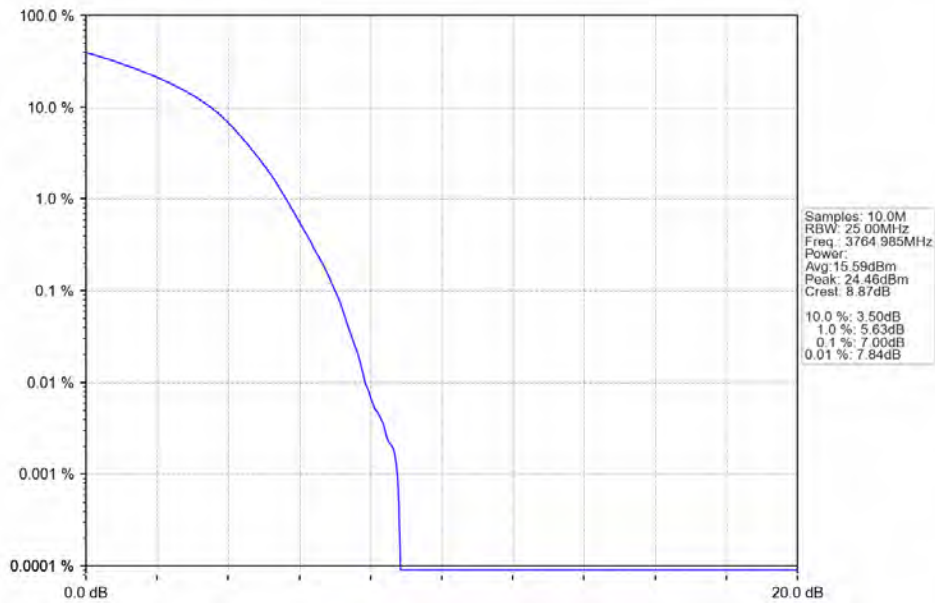
n78a 30kHz SISO NTN 70MHz DFT-s-OFDM QPSK 3764.985MHz Outer Full
