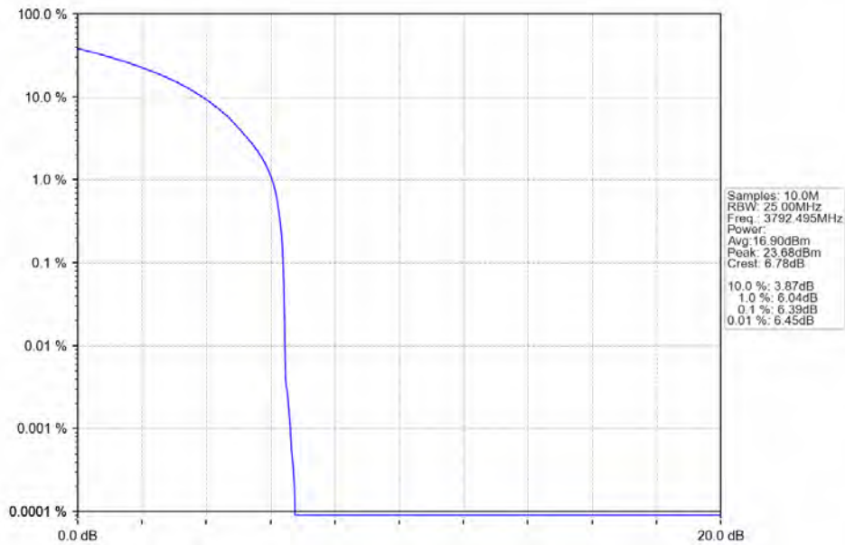
n78a 30kHz SISO NTV 15MHz CP-OFDM QPSK 3792.495MHz Outer Full
