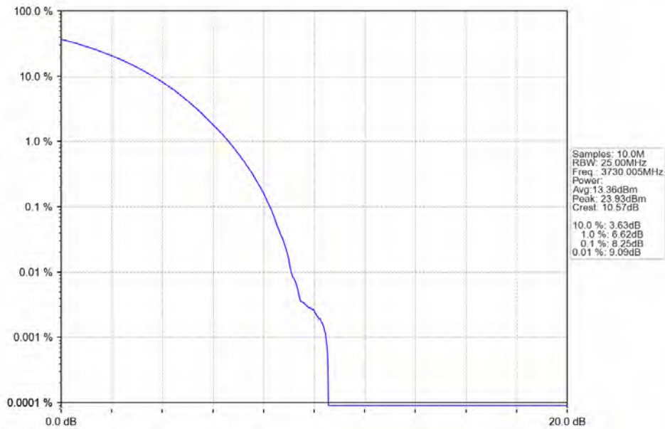
n78a 30kHz SISO NTN 60MHz CP-OFDM 64 QAM 3730.005MHz Outer Full
