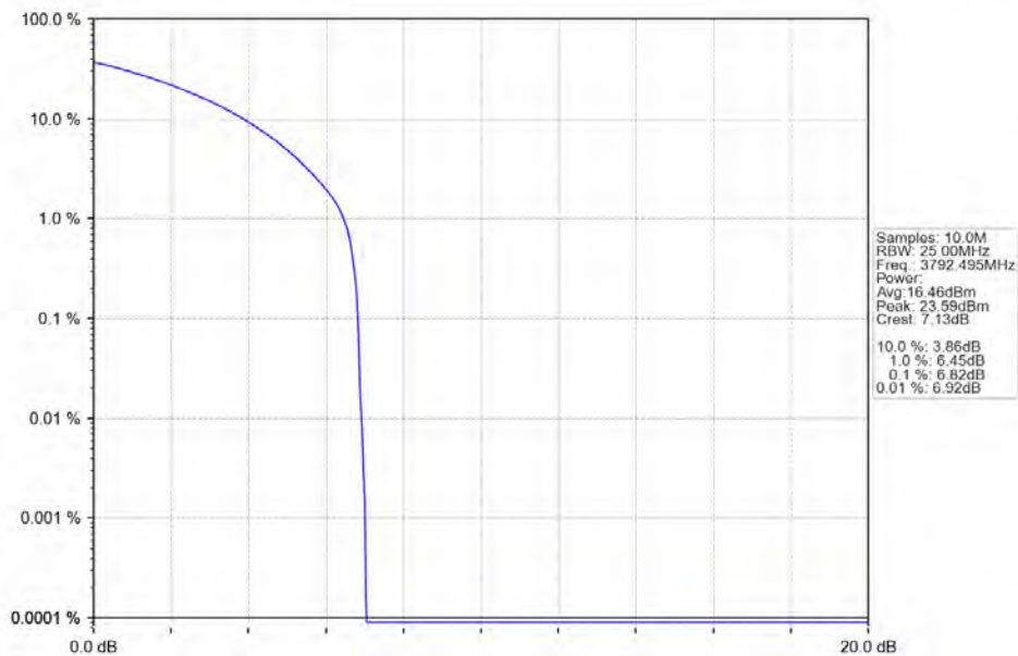
n78a 30kHz SISO NTN 15MHz CP-OFDM 64 QAM 3792.495MHz Outer Full
