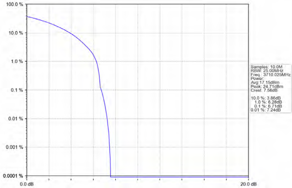
n78a 30kHz SISO NTN 20MHz CP-OFDM 16 QAM 3710.025MHz Outer Full
