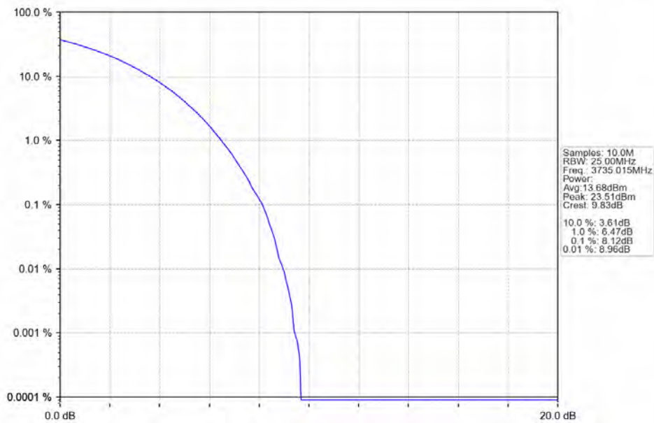
n78a 30kHz SISO NTV 70MHz CP-OFDM QPSK 3735.015MHz Outer Full
