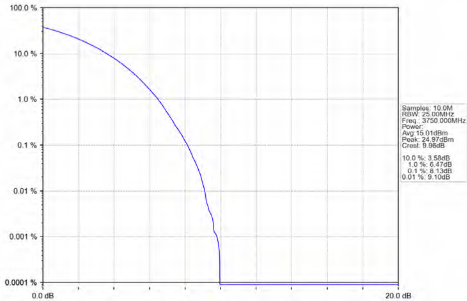
n78a 15kHz SISO NTV 50MHz CP-OFDM 16 QAM 3750MHz Outer Full
