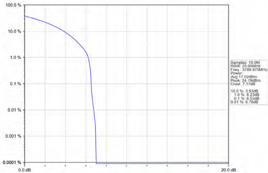
n78a 30kHz SISO NTV 20MHz CP-OFDM QPSK 3789.975MHz Outer Full
