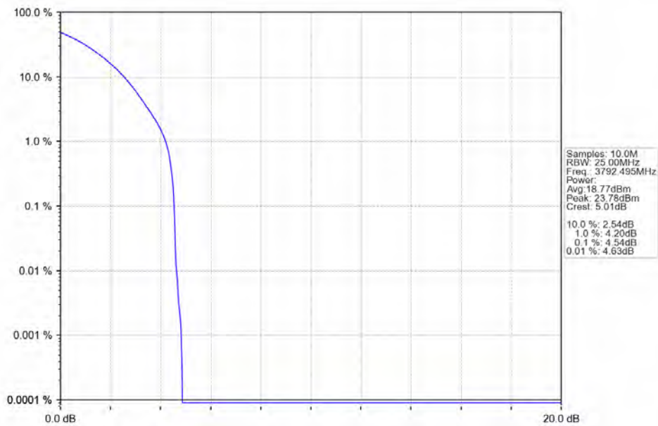
n78a 30kHz SISO NTN 15MHz DFT-s-OFDM QPSK 3792.495MHz Outer Full
