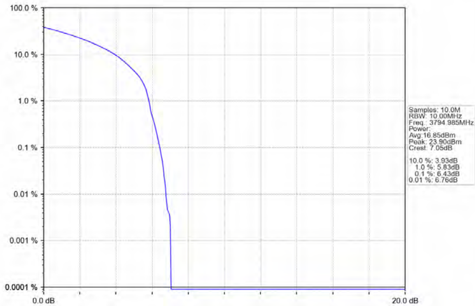
n78a 30kHz SISO NTV 10MHz CP-OFDM QPSK 3794.985MHz Outer Full
