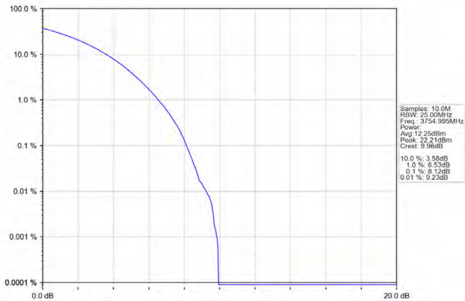
n78a 30kHz SISO NTN 90MHz CP-OFDM 64 QAM 3754.995MHz Outer Full
