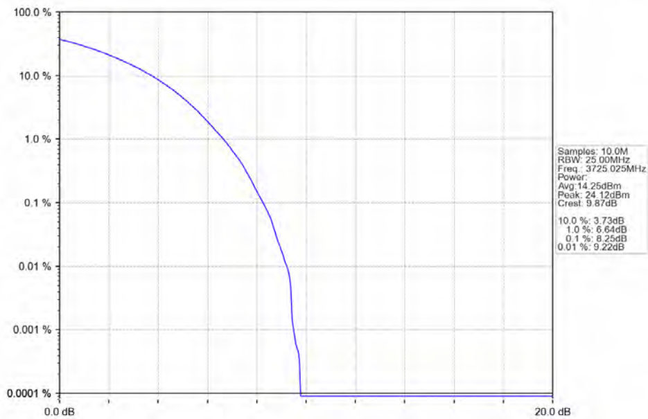
n78a 30kHz SISO NTN 50MHz CP-OFDM 64 QAM 3725.025MHz Outer Full
