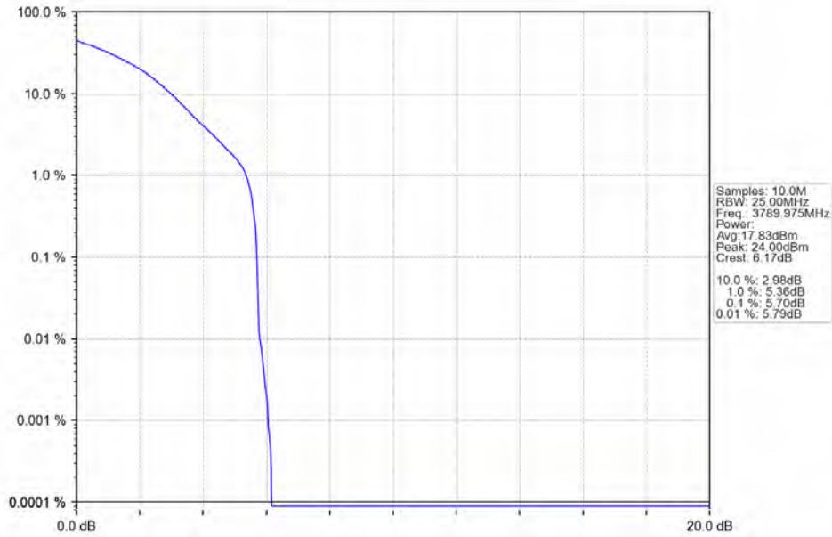
n78a 30kHz SISO NTN 20MHz DFT-s-OFDM 16 QAM 3789.975MHz Outer Full
