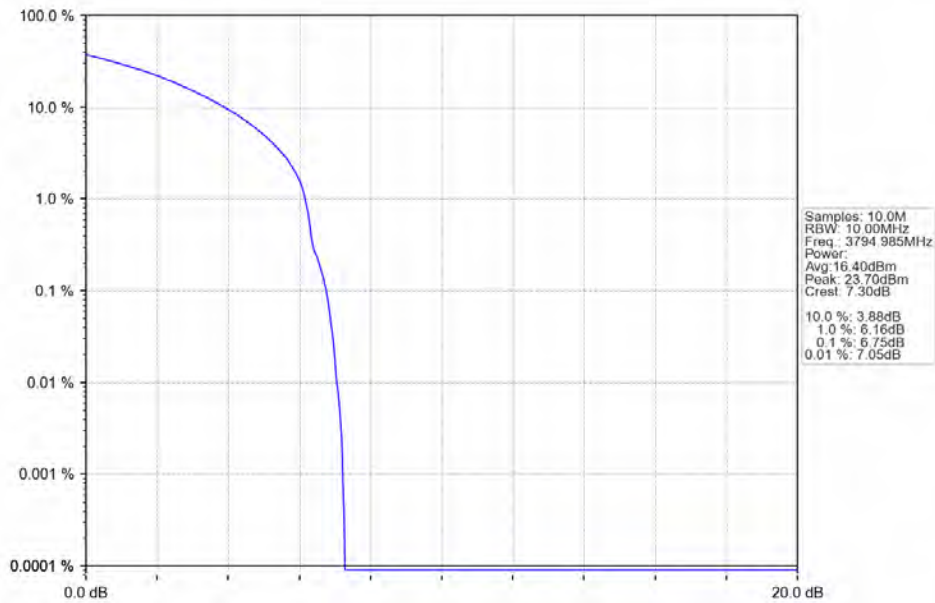
n78a 30kHz SISO NTN 10MHz CP-OFDM 64 QAM 3794.985MHz Outer Full
