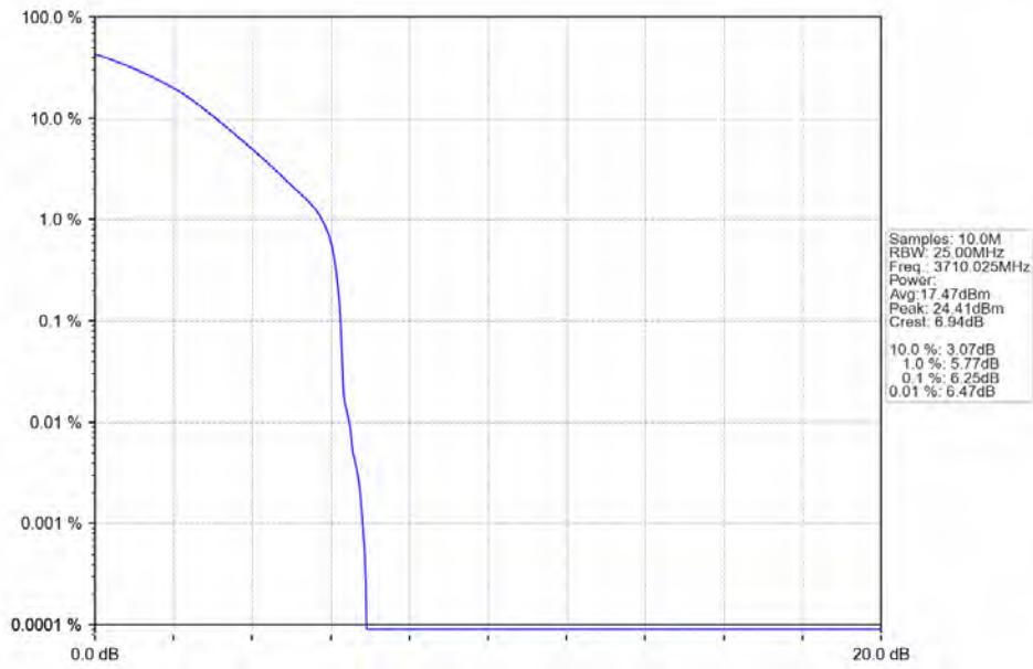
n78a 30kHz SISO NTN 20MHz DFT-s-OFDM 64 QAM 3710.025MHz Outer Full
