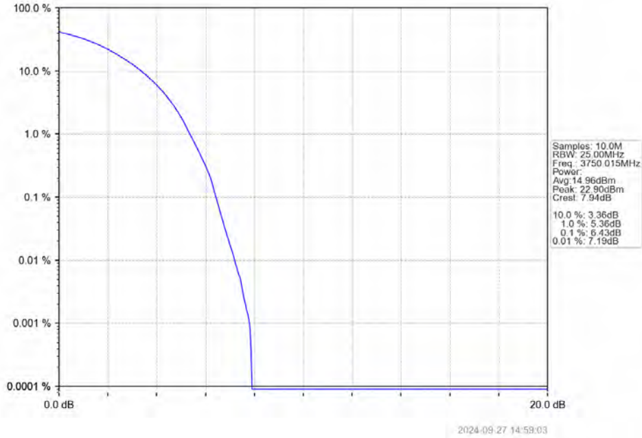
n78a_30kHz_SISO_NTNV_100MHz_DFT-s-OFDM_PI/2_BPSK_3750.015MHz_Outer_Full
