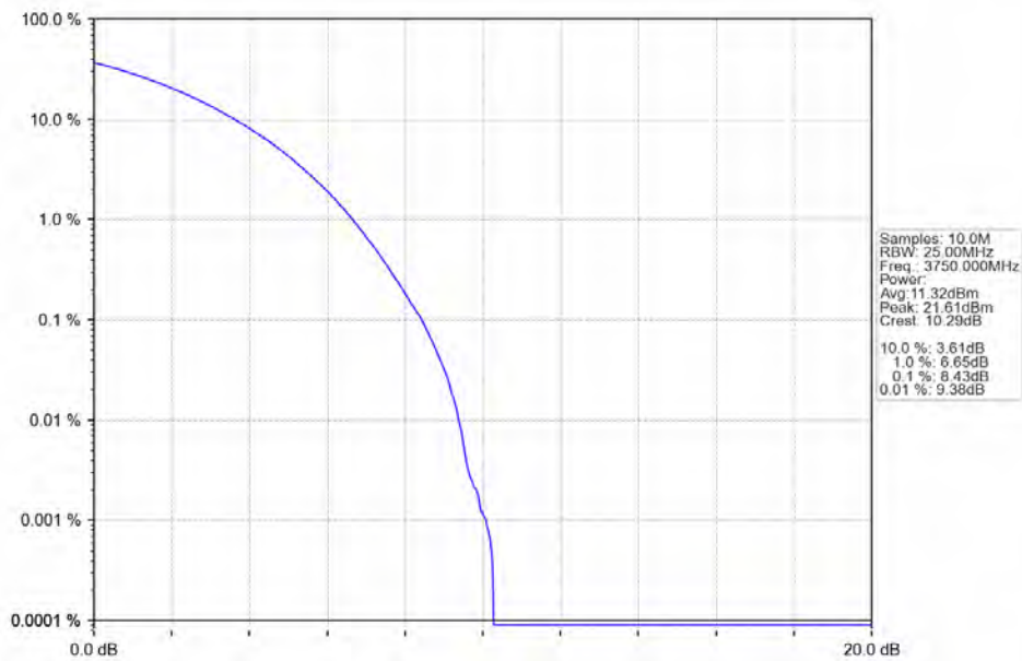
n78a 15kHz SISO NTN 50MHz CP-OFDM 256 QAM 3750MHz Outer Full
