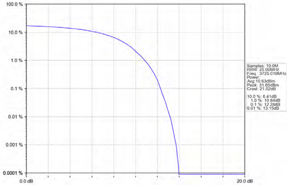
n78a_15kHz_SISO_NTNV_50MHz_DFT-s-OFDM_PI/2_BPSK_3725.01MHz_Outer_Full
