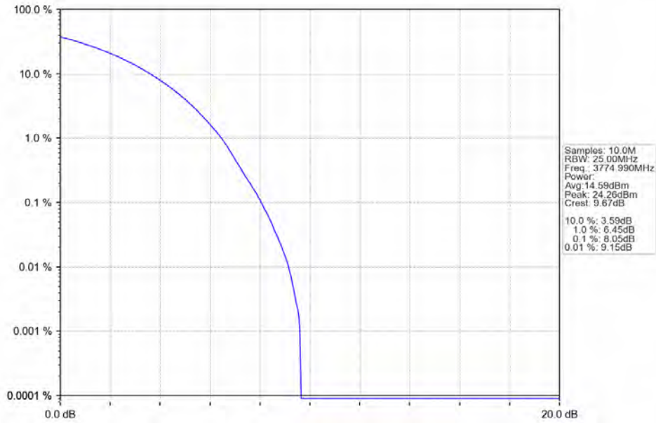
n78a 15kHz SISO NTV 50MHz CP-OFDM 16 QAM 3774.99MHz Outer Full
