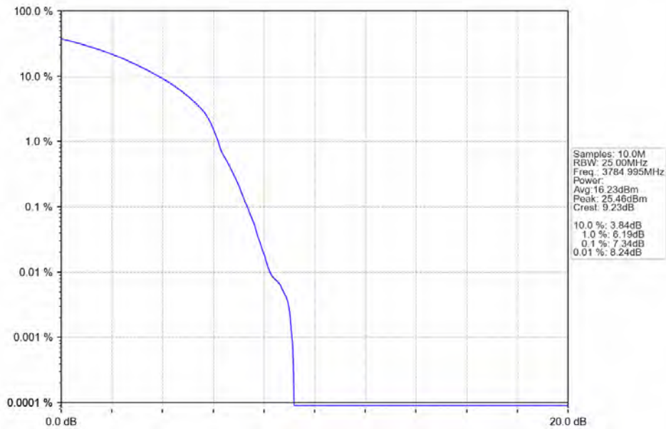
n78a 30kHz SISO NTN 30MHz CP-OFDM 64 QAM 3784.995MHz Outer Full
