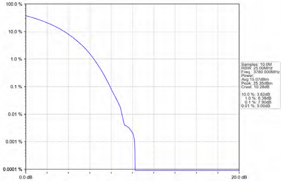
n78a 15kHz SISO NTN 40MHz CP-OFDM 16 QAM 3780MHz Outer Full
