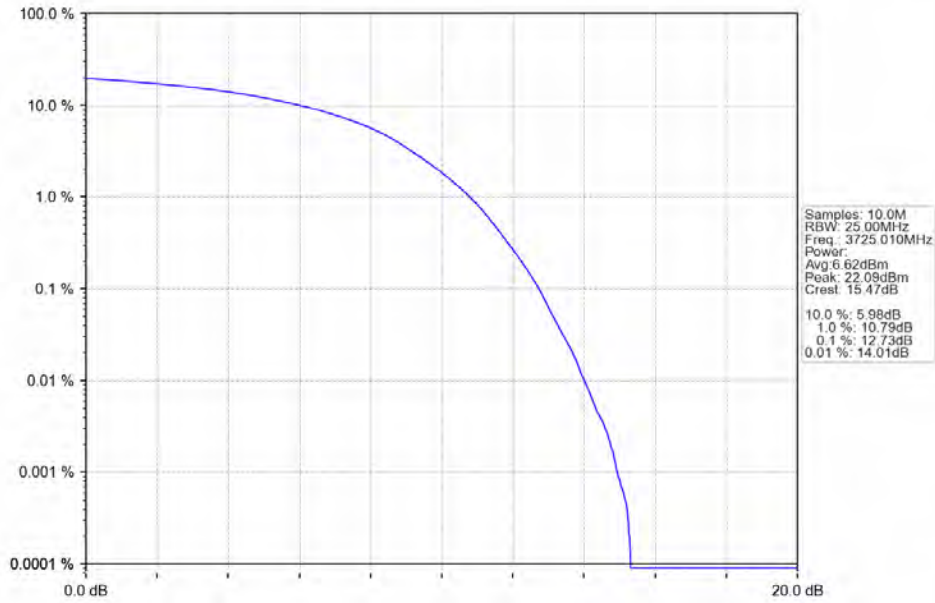
n78a 15kHz SISO NTN 50MHz DFT-s-OFDM 256 QAM 3725.01MHz Outer Full
