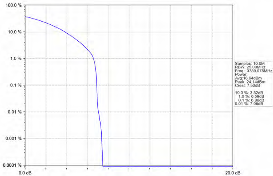
n78a 30kHz SISO NTN 20MHz CP-OFDM 64 QAM 3789.975MHz Outer Full
