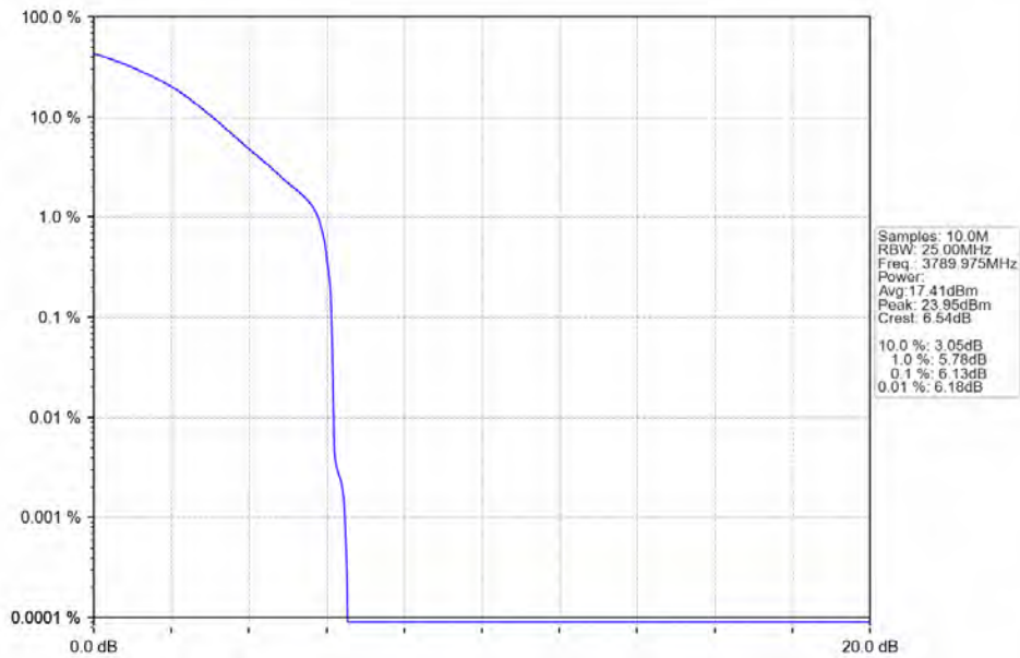
n78a 30kHz SISO NTN 20MHz DFT-s-OFDM 64 QAM 3789.975MHz Outer Full
