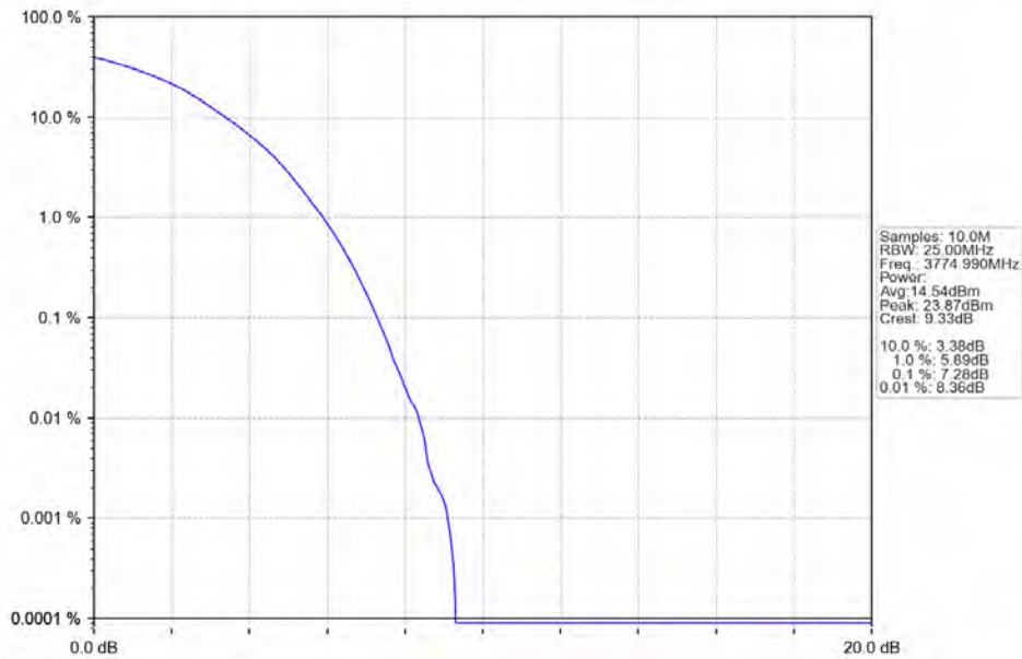
n78a 15kHz SISO NTN 50MHz DFT-s-OFDM 64 QAM 3774.99MHz Outer Full
