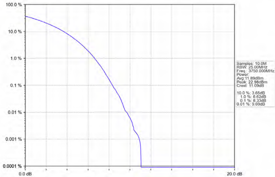
n78a 15kHz SISO NTN 40MHz CP-OFDM 256 QAM 3750MHz Outer Full
