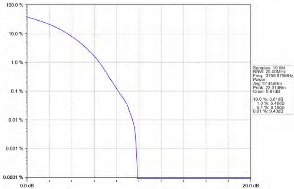
n78a 30kHz SISO NTN 80MHz CP-OFDM 64 QAM 3759.975MHz Outer Full
