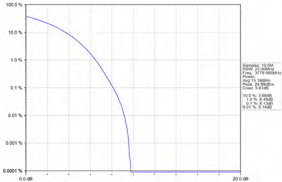
n78a 30kHz SISO NTV 40MHz CP-OFDM QPSK 3779.985MHz Outer Full
