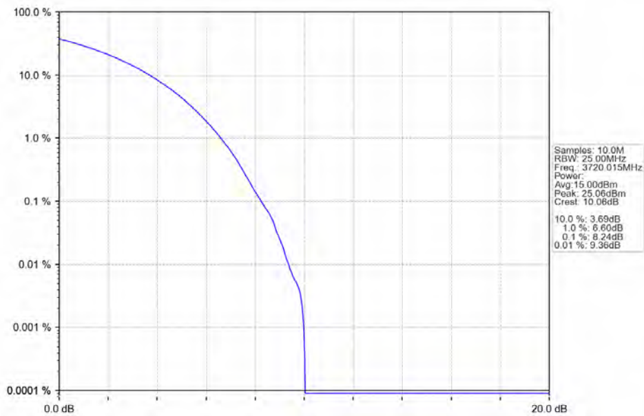
n78a 30kHz SISO NTN 40MHz CP-OFDM 64 QAM 3720.015MHz Outer Full
