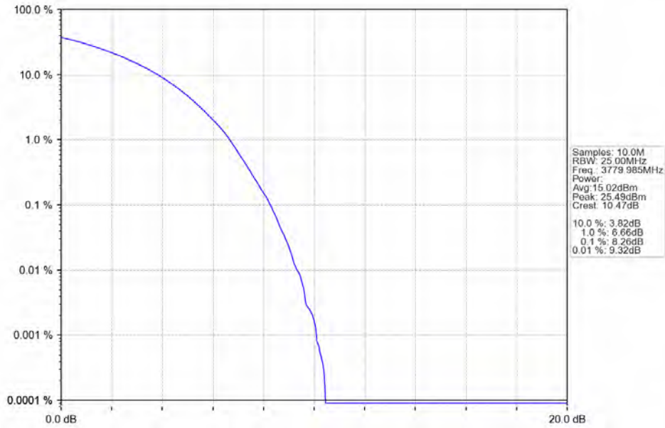
n78a 30kHz SISO NTN 40MHz CP-OFDM 16 QAM 3779.985MHz Outer Full
