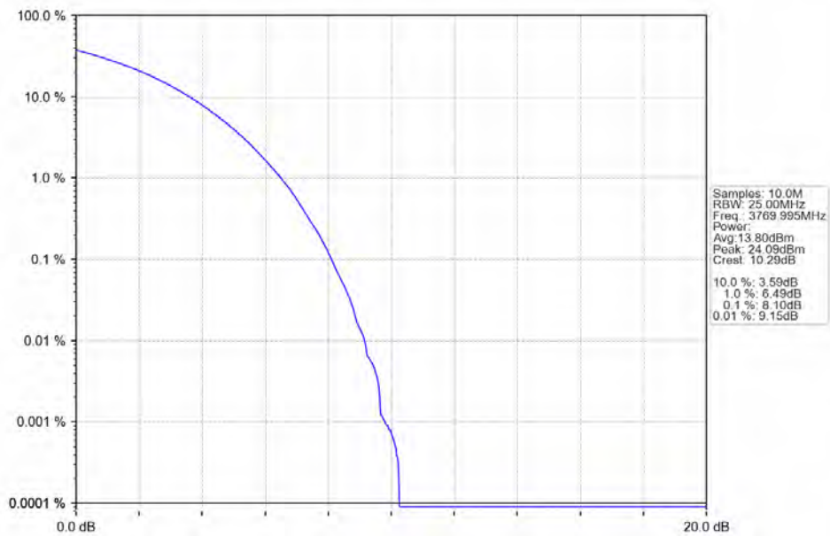
n78a 30kHz SISO NTV 60MHz CP-OFDM QPSK 3769.995MHz Outer Full
