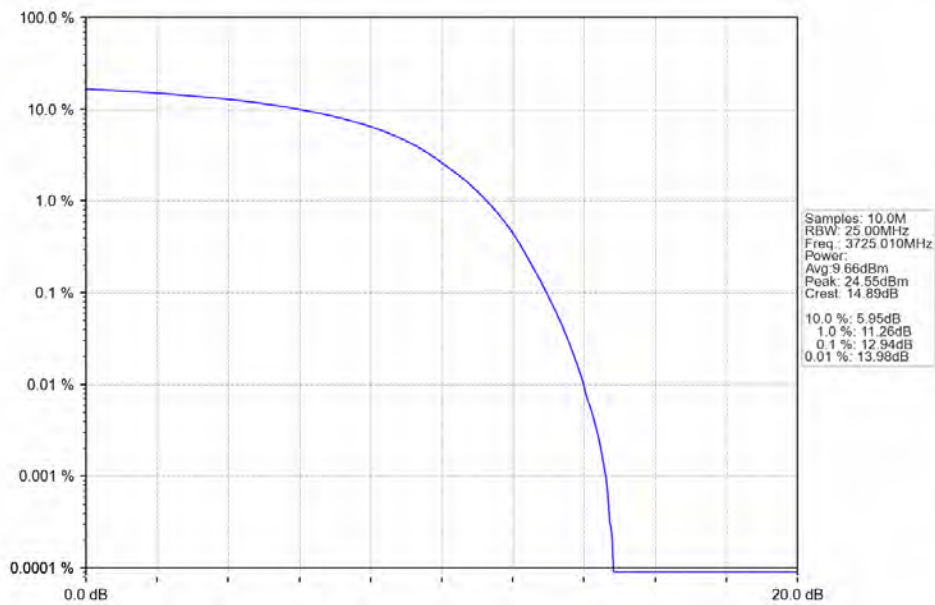
n78a 15kHz SISO NTN 50MHz DFT-s-OFDM QPSK 3725.01MHz Outer Full
