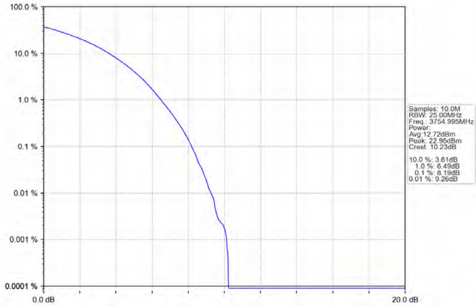
n78a 30kHz SISO NTN 90MHz CP-OFDM 16 QAM 3754.995MHz Outer Full
