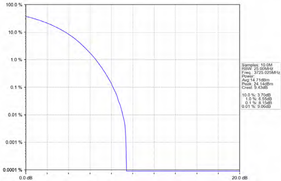
n78a 30kHz SISO NTV 50MHz CP-OFDM QPSK 3725.025MHz Outer Full
