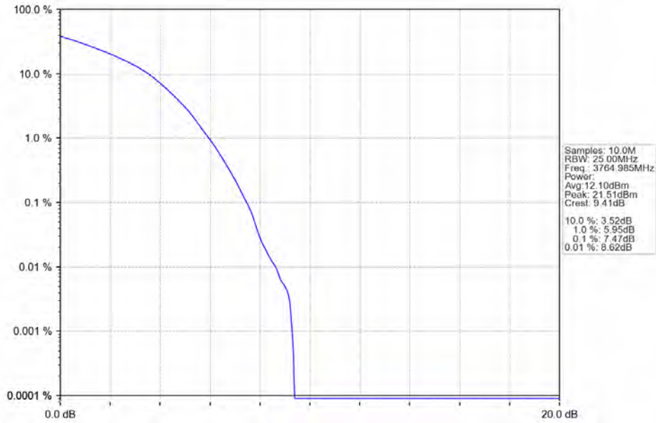
n78a 30kHz SISO NTV 70MHz DFT-s-OFDM 256 QAM 3764.985MHz Outer Full
