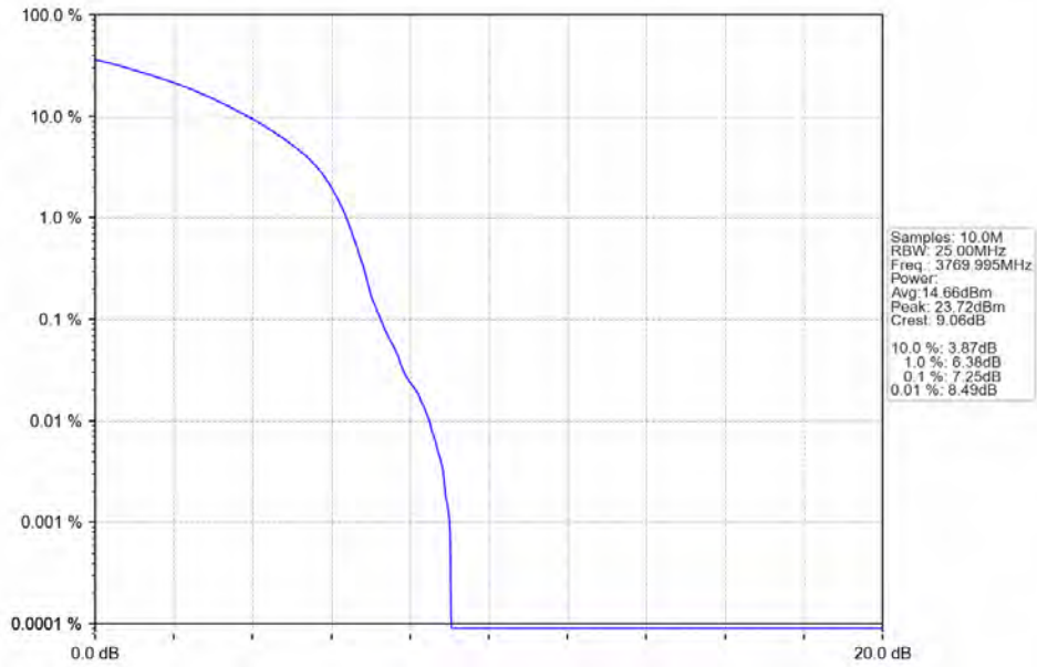
n78a 30kHz SISO NTN 60MHz DFT-s-OFDM 16 QAM 3769.995MHz Outer Full
