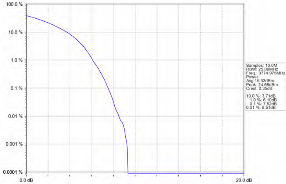
n78a 30kHz SISO NTN 50MHz DFT-s-OFDM 16 QAM 3774.975MHz Outer Full
