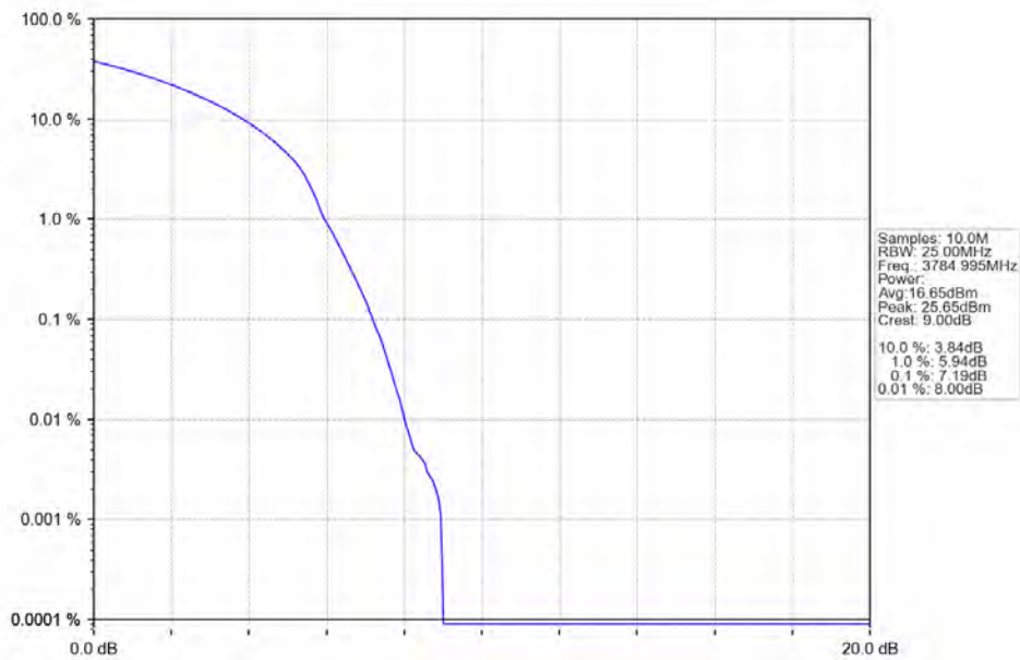
n78a 30kHz SISO NTV 30MHz CP-OFDM QPSK 3784.995MHz Outer Full
