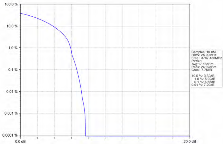
n78a 30kHz SISO NTV 25MHz CP-OFDM QPSK 3787.485MHz Outer Full
