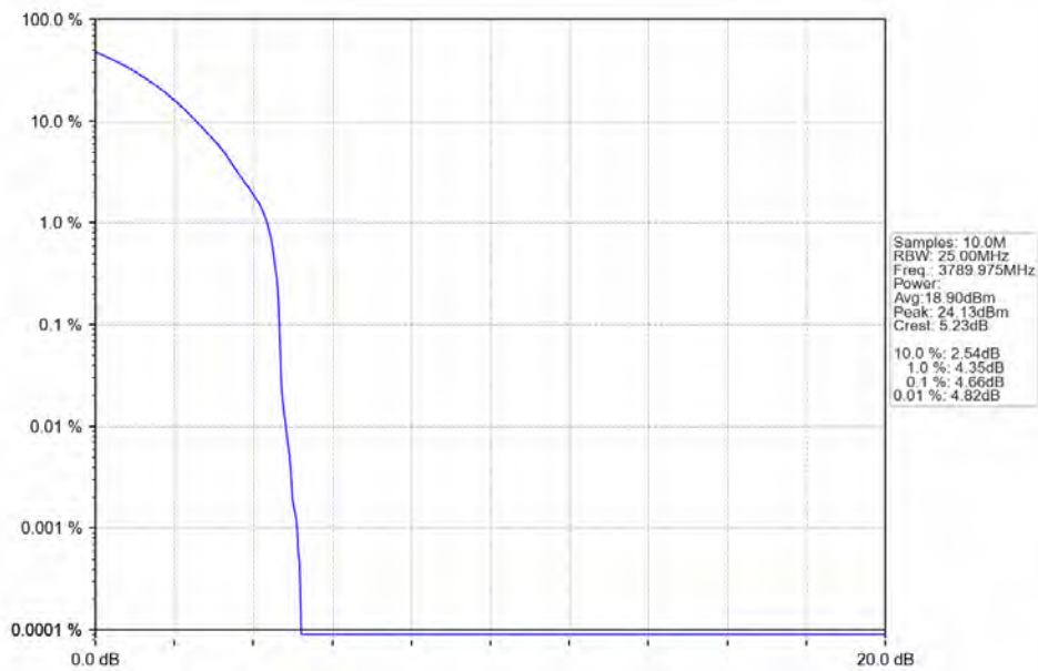
n78a 30kHz SISO NTN 20MHz DFT-s-OFDM QPSK 3789.975MHz Outer Full
