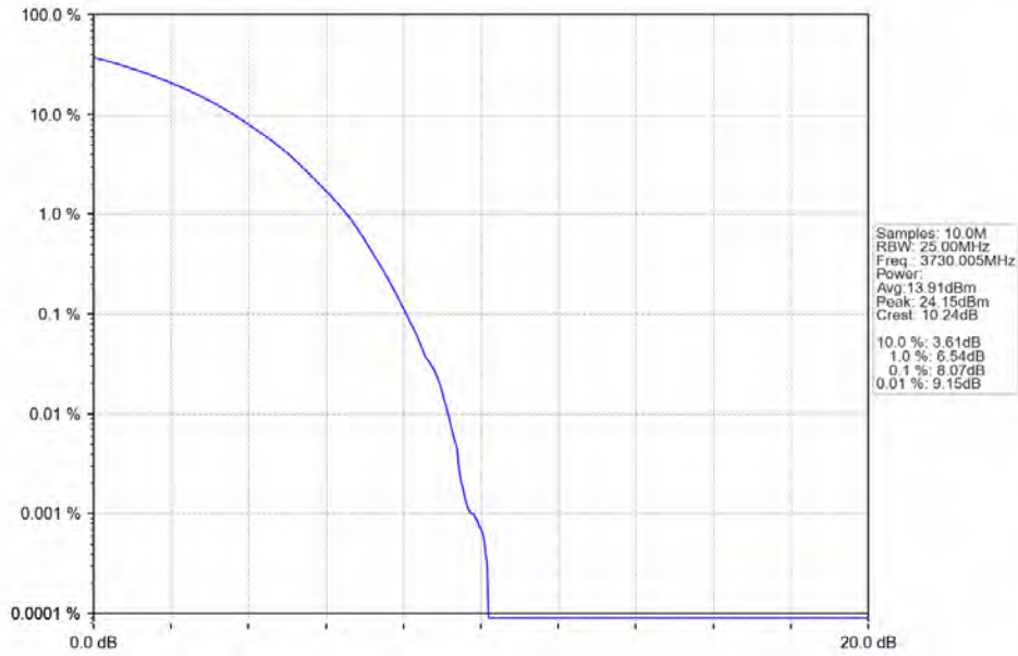
n78a 30kHz SISO NTN 60MHz CP-OFDM 16 QAM 3730.005MHz Outer Full
