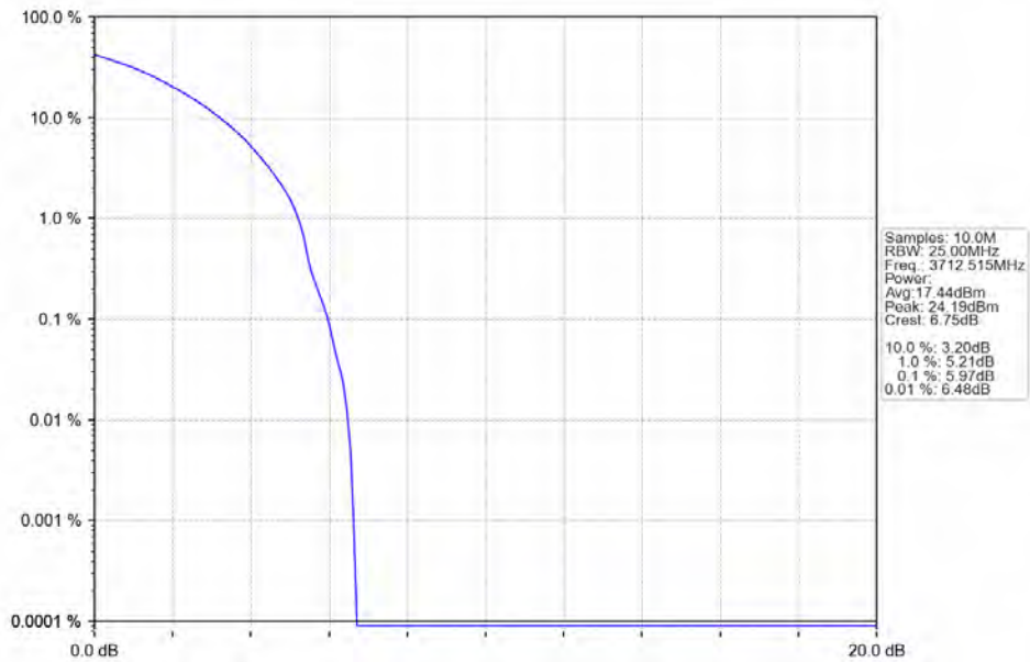
n78a 30kHz SISO NTN 25MHz DFT-s-OFDM 64 QAM 3712.515MHz Outer Full
