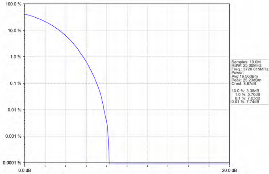
n78a 30kHz SISO NTN 40MHz DFT-s-OFDM 16 QAM 3720.015MHz Outer Full
