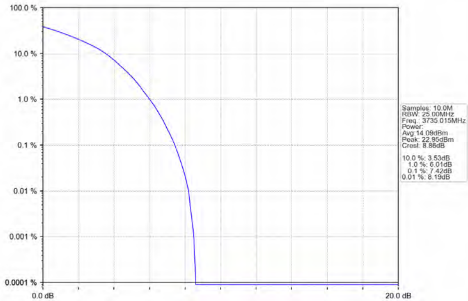
n78a 30kHz SISO NTN 70MHz DFT-s-OFDM 64 QAM 3735.015MHz Outer Full
