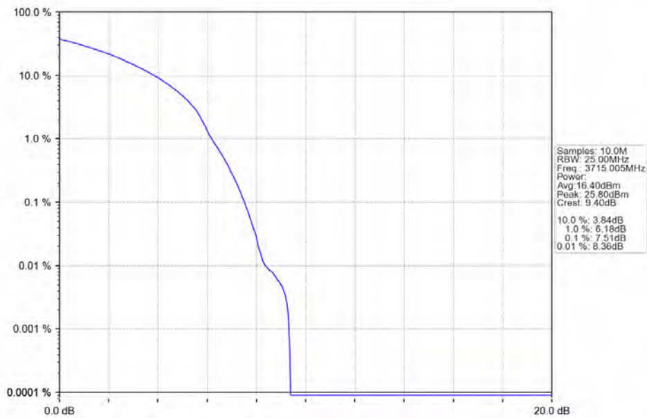
n78a 30kHz SISO NTN 30MHz CP-OFDM 64 QAM 3715.005MHz Outer Full
