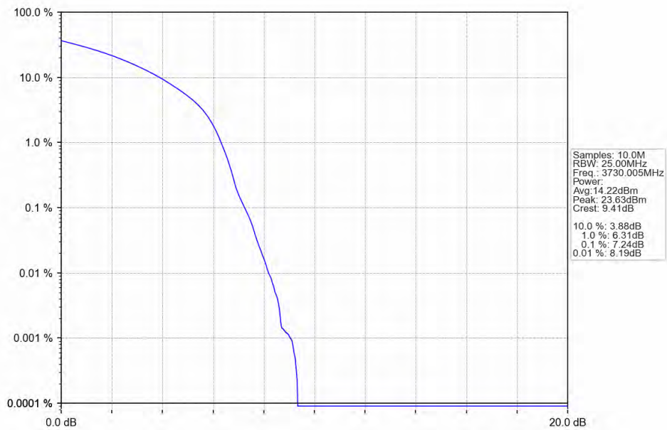
n78a 30kHz SISO NTN 60MHz DFT-s-OFDM 64 QAM 3730.005MHz Outer Full
