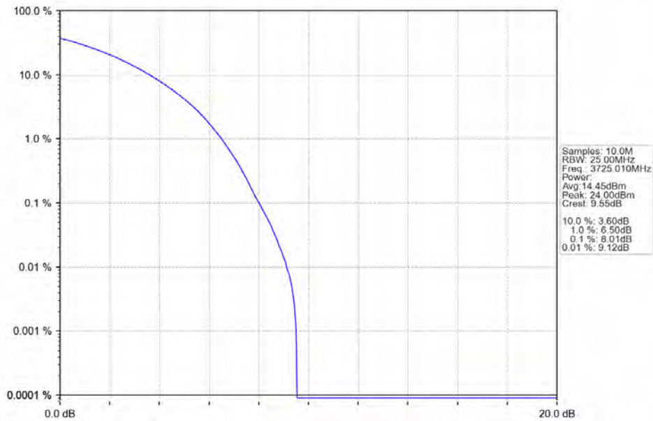
n78a 15kHz SISO NTV 50MHz CP-OFDM 64 QAM 3725.01MHz Outer Full
