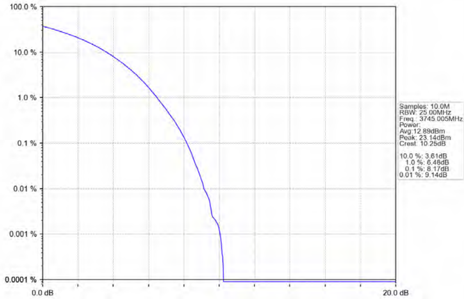
n78a 30kHz SISO NTN 90MHz CP-OFDM 16 QAM 3745.005MHz Outer Full
