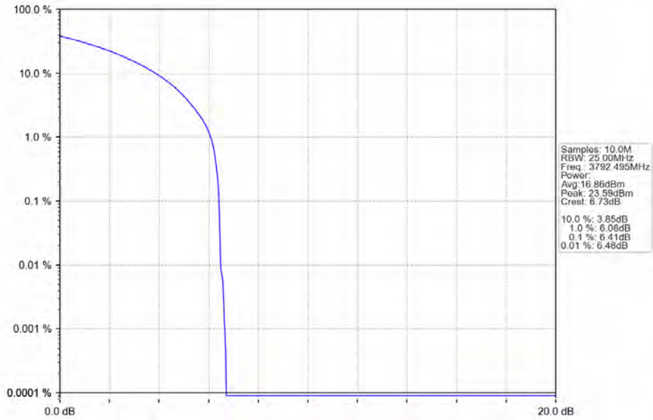
n78a 30kHz SISO NTN 15MHz CP-OFDM 16 QAM 3792.495MHz Outer Full
