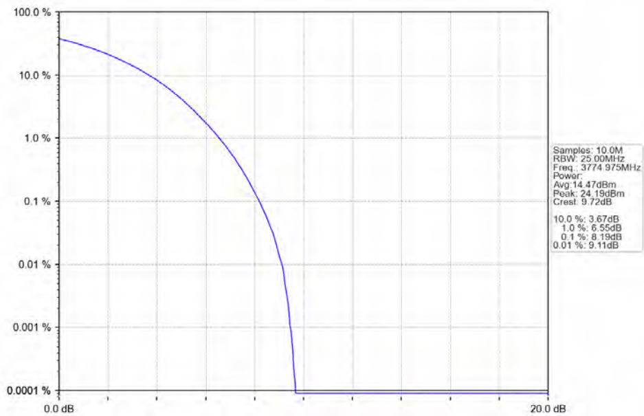
n78a 30kHz SISO NTV 50MHz CP-OFDM QPSK 3774.975MHz Outer Full
