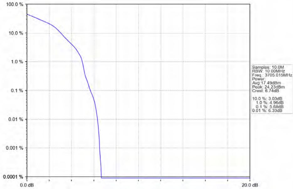
n78a 30kHz SISO NTN 10MHz DFT-s-OFDM 16 QAM 3705.015MHz Outer Full
