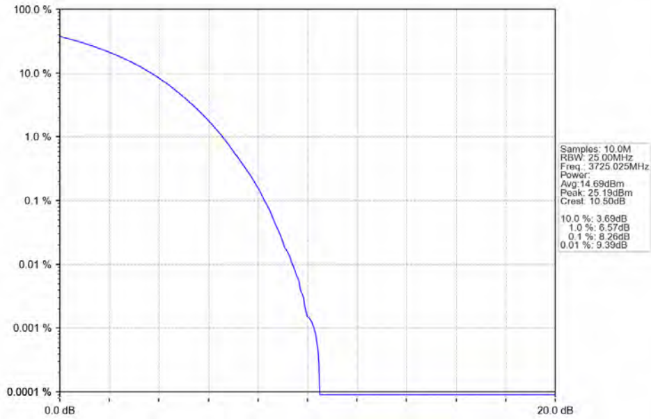
n78a 30kHz SISO NTN 50MHz CP-OFDM 16 QAM 3725.025MHz Outer Full
