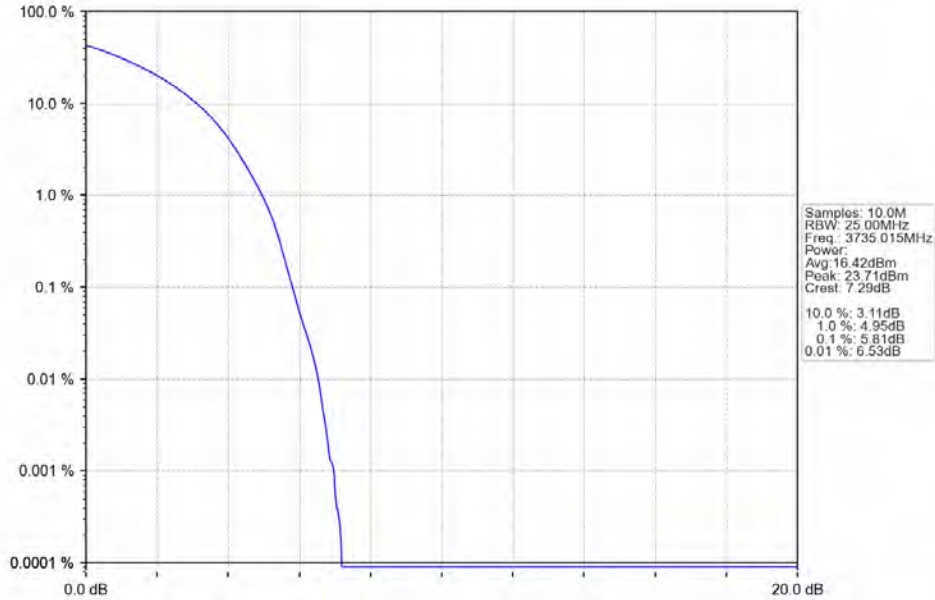
n78a_30kHz_SISO_NTNV_70MHz_DFT-s-OFDM_PI/2_BPSK_3735.015MHz_Outer_Full
