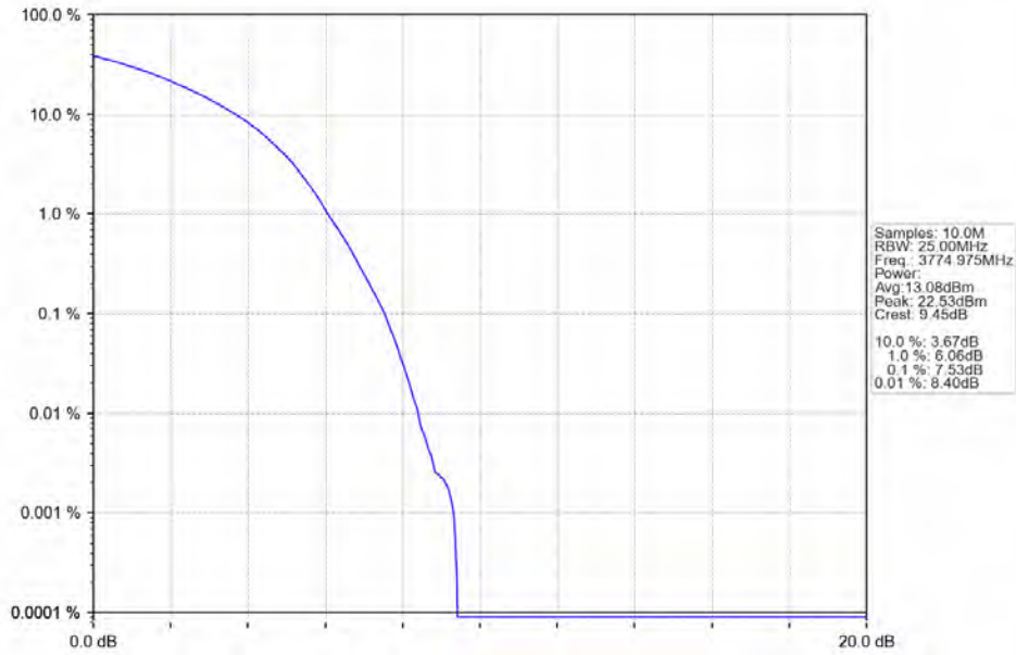
n78a 30kHz SISO NTV 50MHz DFT-s-OFDM 256 QAM 3774.975MHz Outer Full
