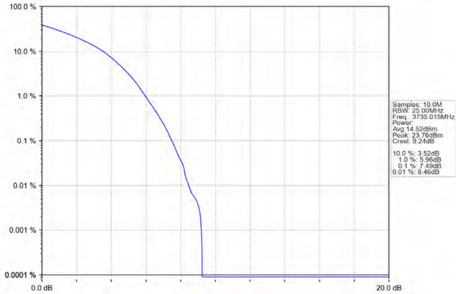
n78a 30kHz SISO NTN 70MHz DFT-s-OFDM 16 QAM 3735.015MHz Outer Full
