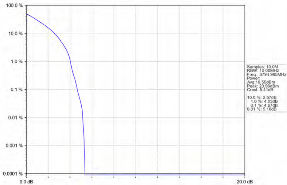
n78a 30kHz SISO NTN 10MHz DFT-s-OFDM QPSK 3794.985MHz Outer Full
