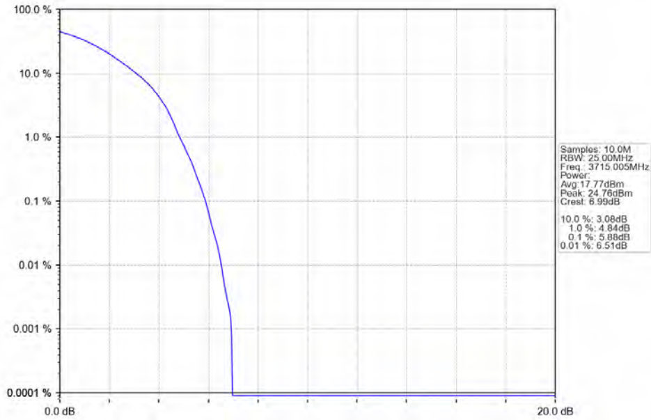
n78a 30kHz SISO NTN 30MHz DFT-s-OFDM 16 QAM 3715.005MHz Outer Full
