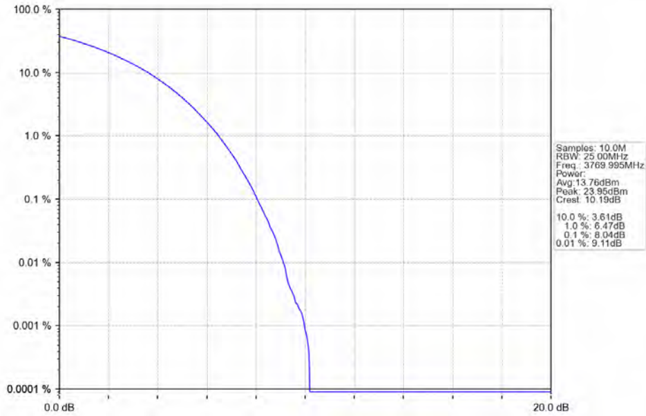
n78a 30kHz SISO NTN 60MHz CP-OFDM 16 QAM 3769.995MHz Outer Full
