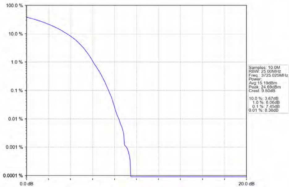
n78a 30kHz SISO NTN 50MHz DFT-s-OFDM 64 QAM 3725.025MHz Outer Full
