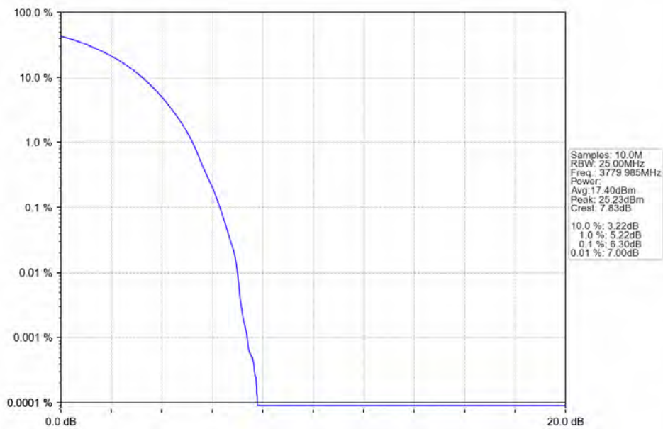
n78a 30kHz SISO NTN 40MHz DFT-s-OFDM QPSK 3779.985MHz Outer Full
