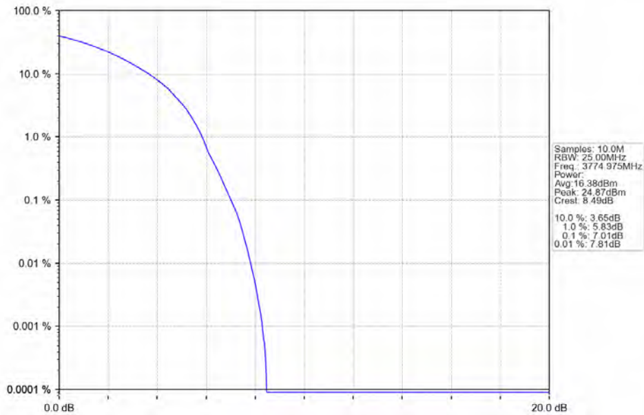
n78a 30kHz SISO NTN 50MHz DFT-s-OFDM QPSK 3774.975MHz Outer Full
