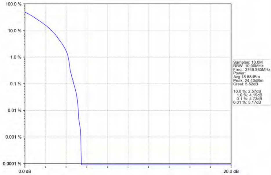
n78a 30kHz SISO NTN 10MHz DFT-s-OFDM QPSK 3750.015MHz Outer Full
