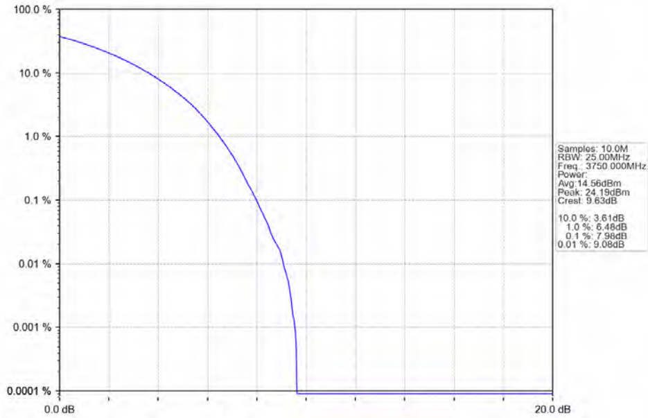
n78a 15kHz SISO NTN 50MHz CP-OFDM 64 QAM 3750MHz Outer Full
