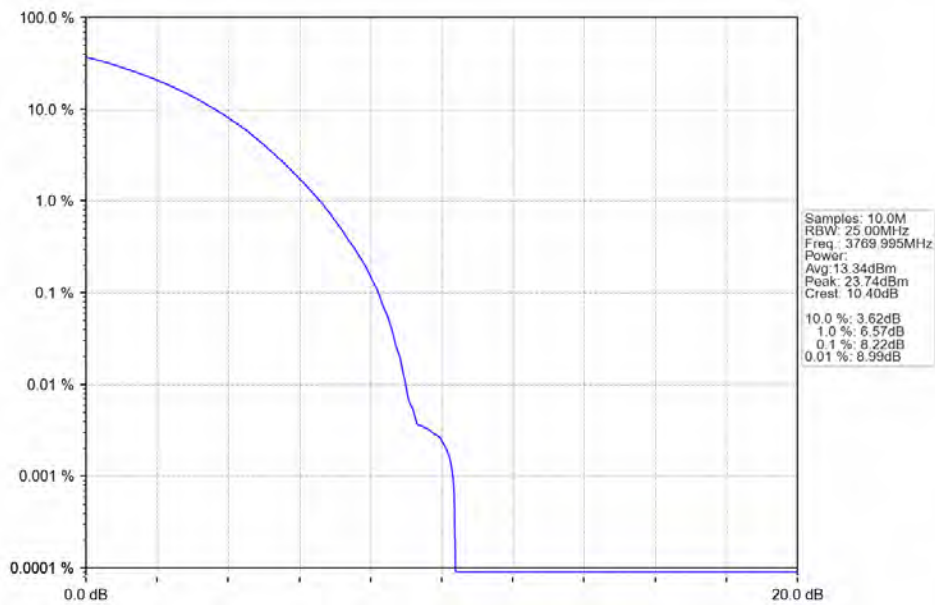
n78a 30kHz SISO NTN 60MHz CP-OFDM 64 QAM 3769.995MHz Outer Full
