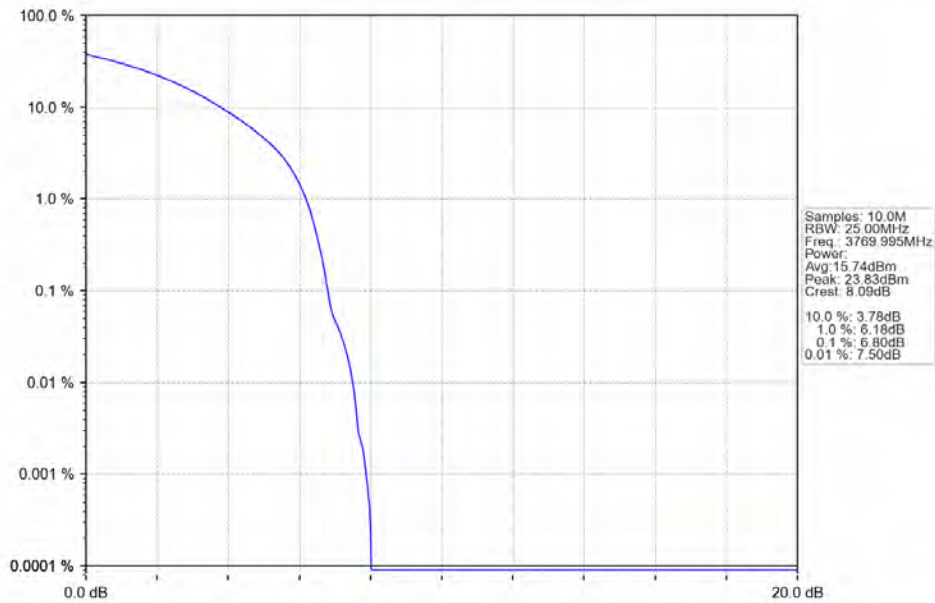
n78a 30kHz SISO NTN 60MHz DFT-s-OFDM QPSK 3769.995MHz Outer Full
