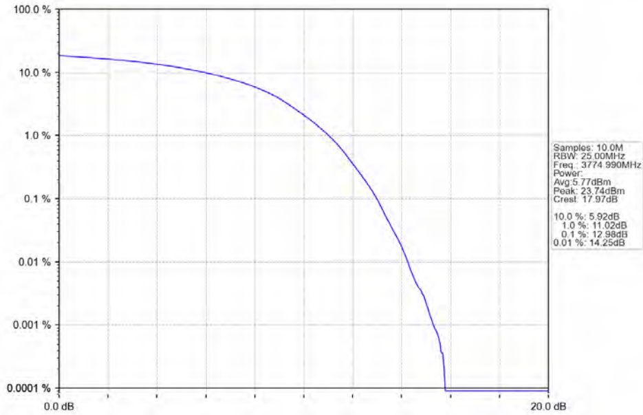
n78a 15kHz SISO NTN 50MHz DFT-s-OFDM 256 QAM 3774.99MHz Outer Full
