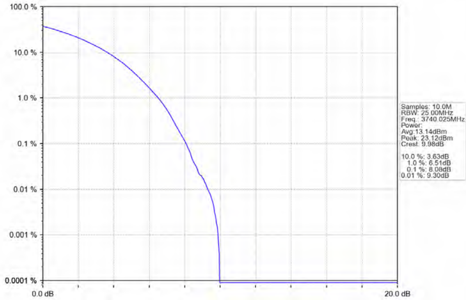
n78a 30kHz SISO NTN 80MHz CP-OFDM 16 QAM 3740.025MHz Outer Full
