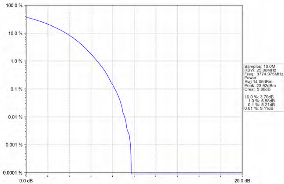
n78a 30kHz SISO NTN 50MHz CP-OFDM 64 QAM 3774.975MHz Outer Full
