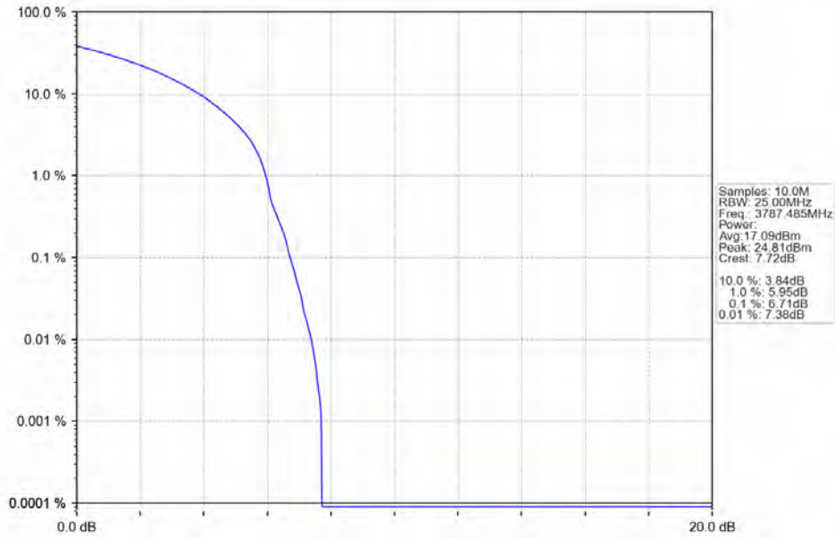
n78a 30kHz SISO NTN 25MHz CP-OFDM 16 QAM 3787.485MHz Outer Full
