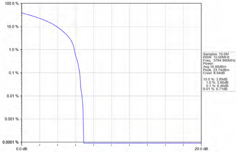
n78a 30kHz SISO NTN 10MHz CP-OFDM 16 QAM 3794.985MHz Outer Full
