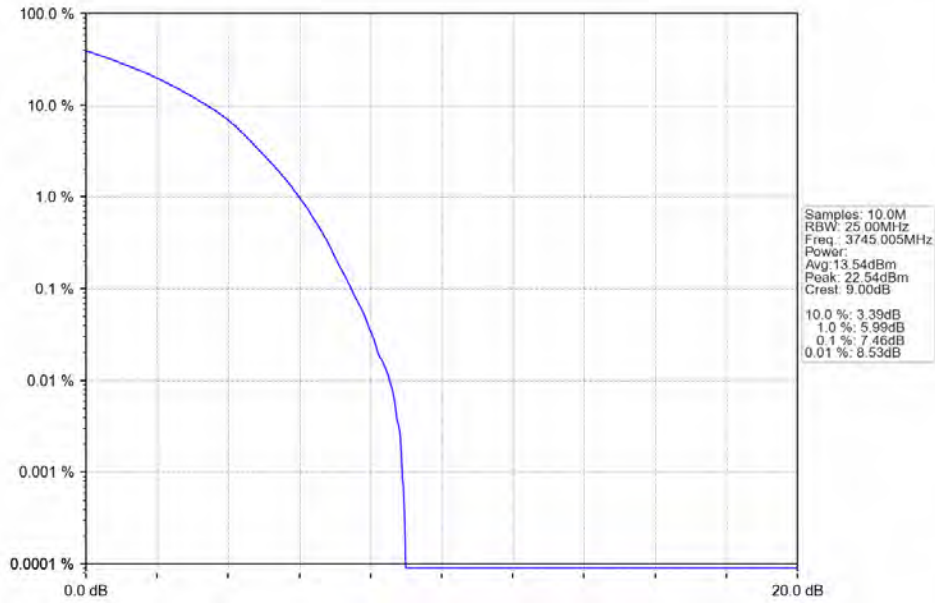
n78a 30kHz SISO NTN 90MHz DFT-s-OFDM 16 QAM 3745.005MHz Outer Full
