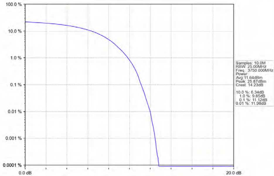
n78a_15kHz_SISO_NTNV_50MHz_DFT-s-OFDM_PI/2_BPSK_3750MHz_Outer_Full
