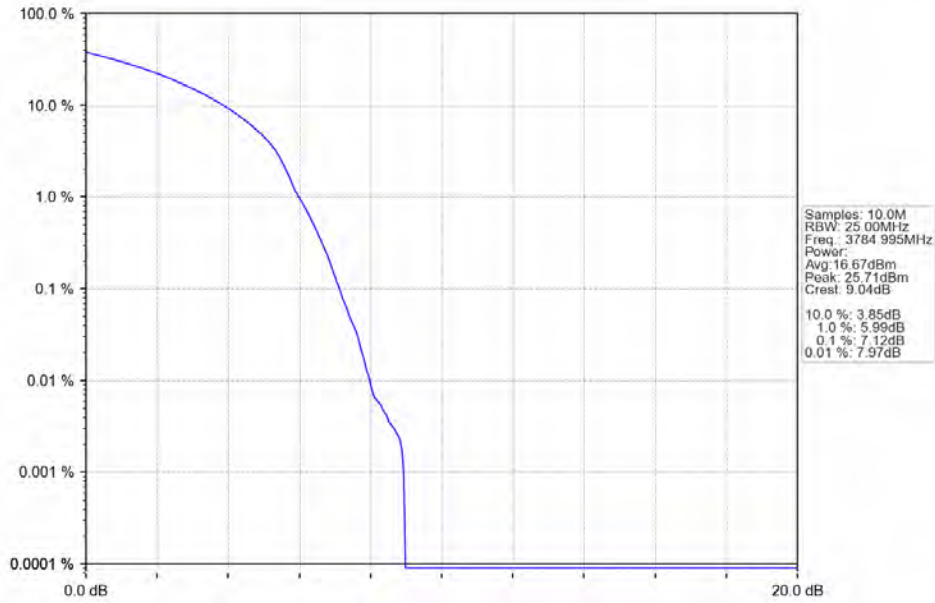
n78a 30kHz SISO NTN 30MHz CP-OFDM 16 QAM 3784.995MHz Outer Full
