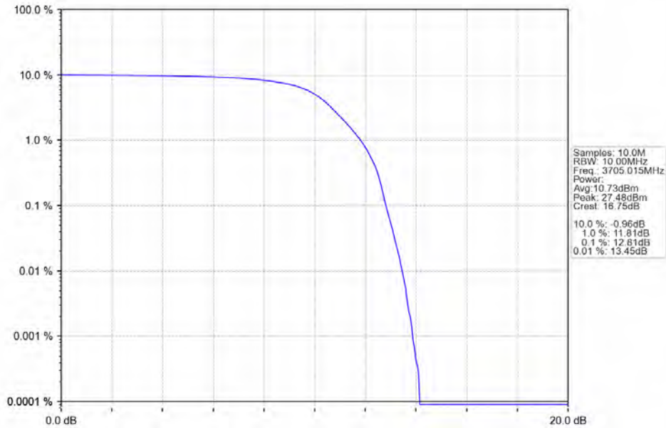
n78a_30kHz_SISO_NTNV_10MHz_DFT-s-OFDM_PI/2_BPSK_3705.015MHz_Outer_Full
