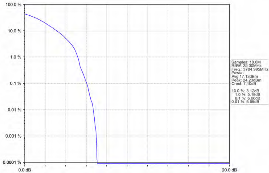
n78a 30kHz SISO NTN 30MHz DFT-s-OFDM 64 QAM 3784.995MHz Outer Full
