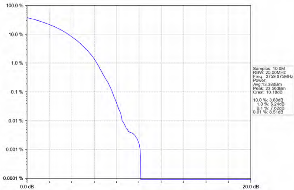
n78a 30kHz SISO NTN 80MHz DFT-s-OFDM 64 QAM 3759.975MHz Outer Full
