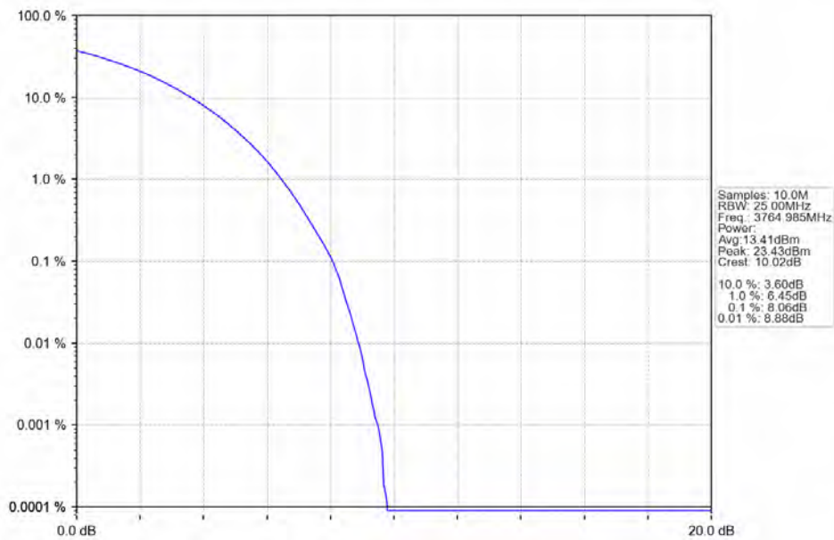
n78a 30kHz SISO NTV 70MHz CP-OFDM QPSK 3764.985MHz Outer Full
