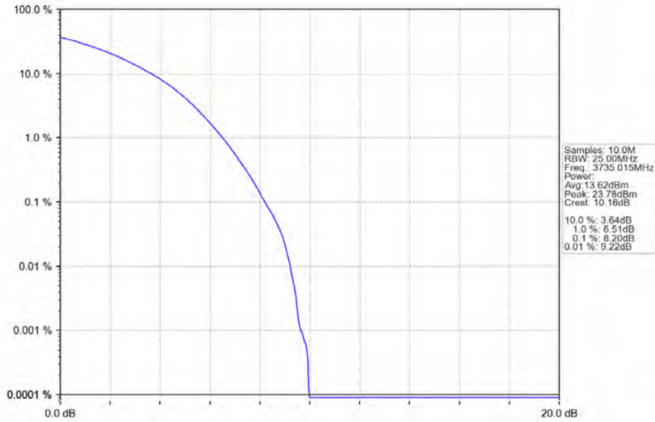
n78a 30kHz SISO NTN 70MHz CP-OFDM 16 QAM 3735.015MHz Outer Full
