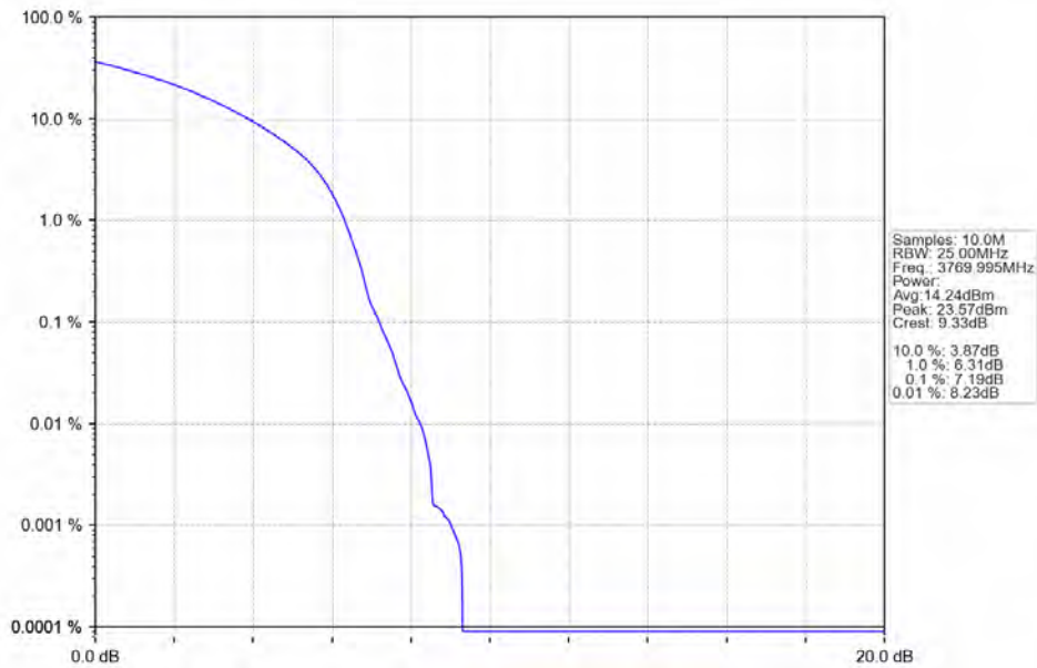
n78a 30kHz SISO NTN 60MHz DFT-s-OFDM 64 QAM 3769.995MHz Outer Full
