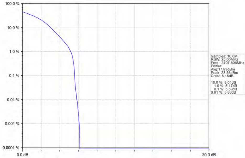
n78a 30kHz SISO NTN 15MHz DFT-s-OFDM 16 QAM 3707.505MHz Outer Full
