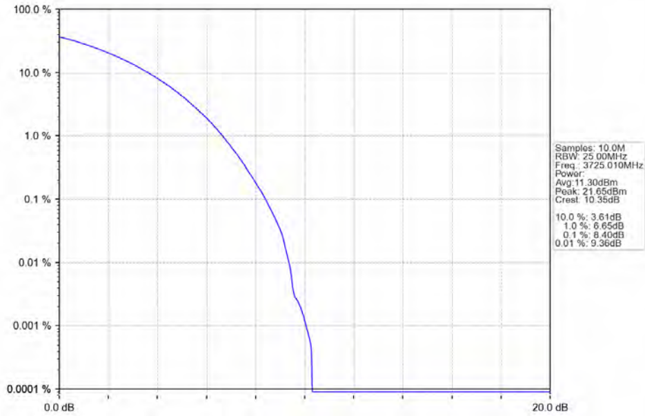
n78a 15kHz SISO NTN 50MHz CP-OFDM 256 QAM 3725.01MHz Outer Full
