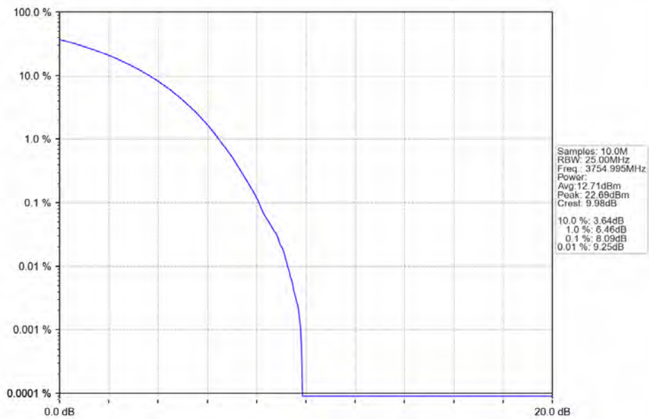
n78a 30kHz SISO NTV 90MHz CP-OFDM QPSK 3754.995MHz Outer Full
