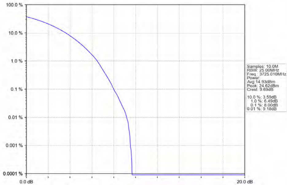
n78a 15kHz SISO NTN 50MHz CP-OFDM QPSK 3725.01MHz Outer Full
