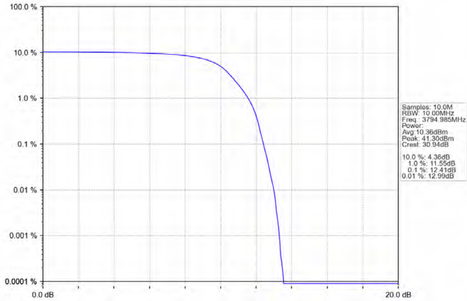
n78a 30kHz SISO NTN 10MHz DFT-s-OFDM PI/2 BPSK 3794.985MHz Outer Full
