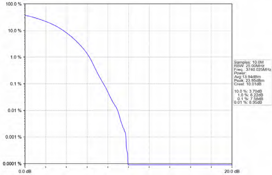
n78a 30kHz SISO NTN 80MHz DFT-s-OFDM 16 QAM 3740.025MHz Outer Full
