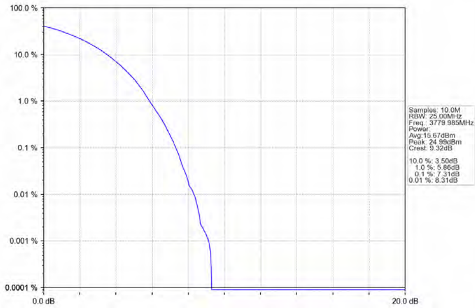
n78a 30kHz SISO NTN 40MHz DFT-s-OFDM 64 QAM 3779.985MHz Outer Full
