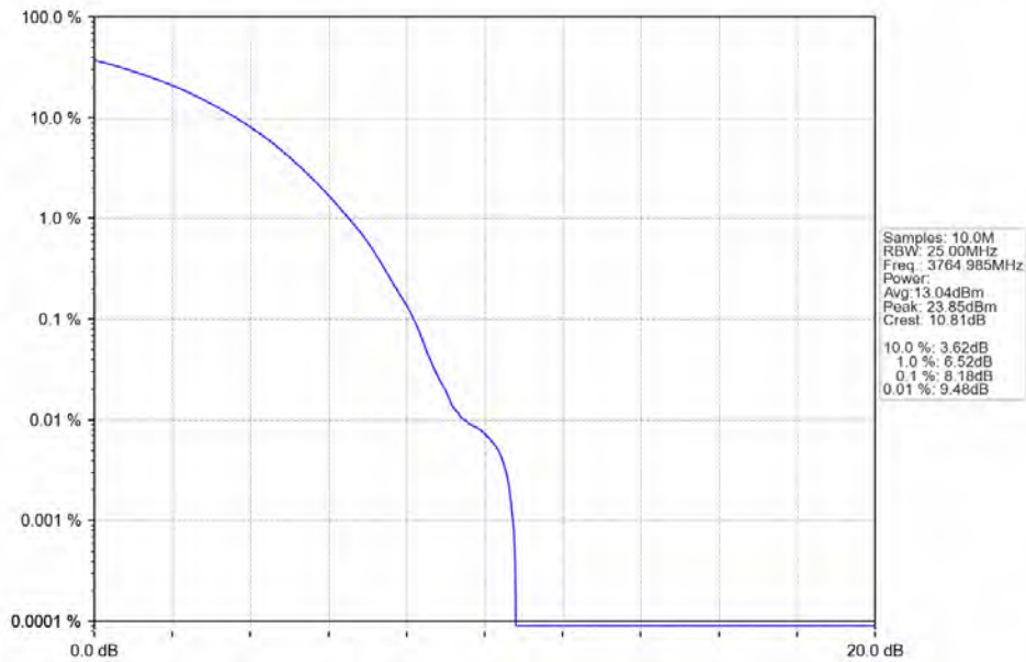
n78a 30kHz SISO NTN 70MHz CP-OFDM 64 QAM 3764.985MHz Outer Full
