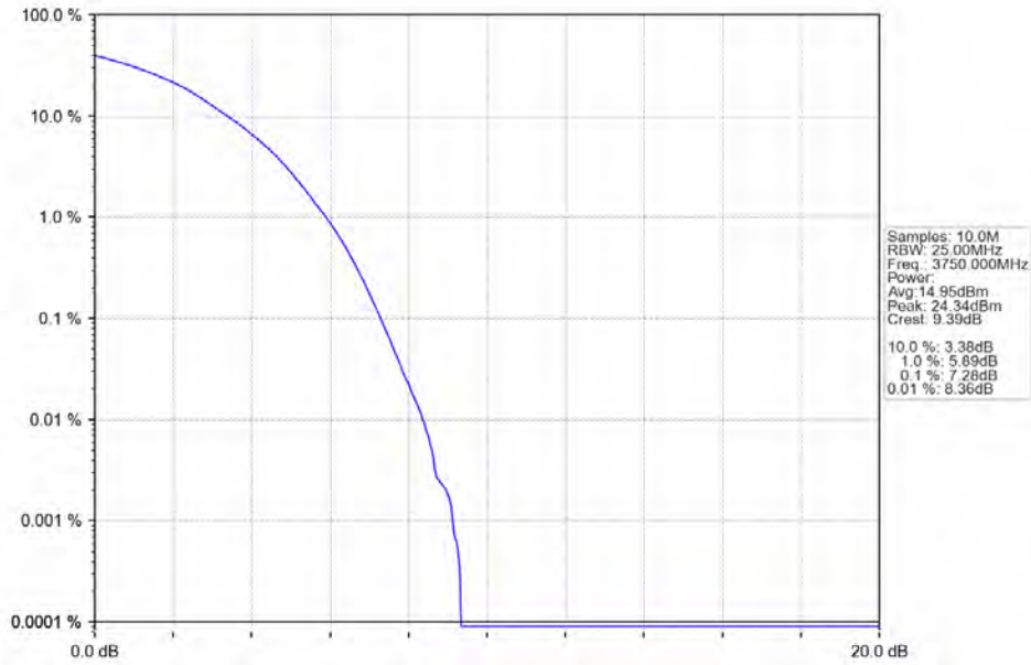
n78a 15kHz SISO NTN 50MHz DFT-s-OFDM 64 QAM 3750MHz Outer Full
