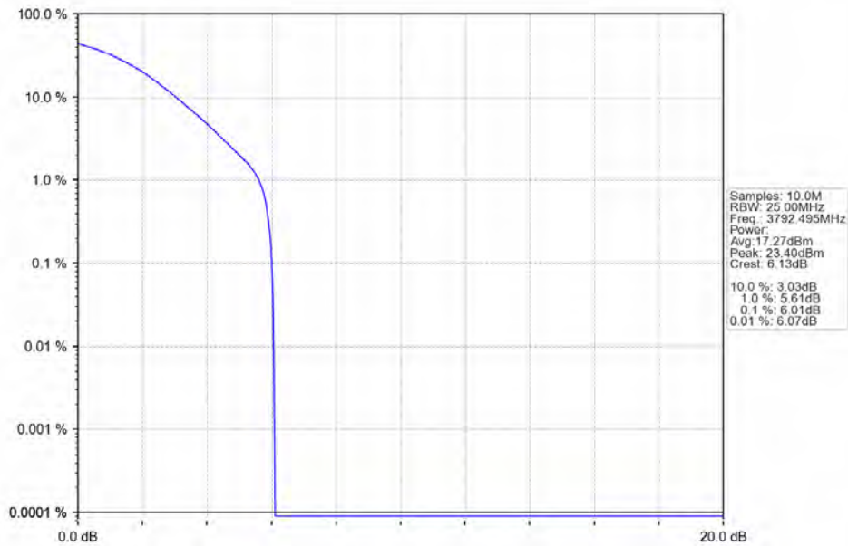
n78a 30kHz SISO NTN 15MHz DFT-s-OFDM 64 QAM 3792.495MHz Outer Full
