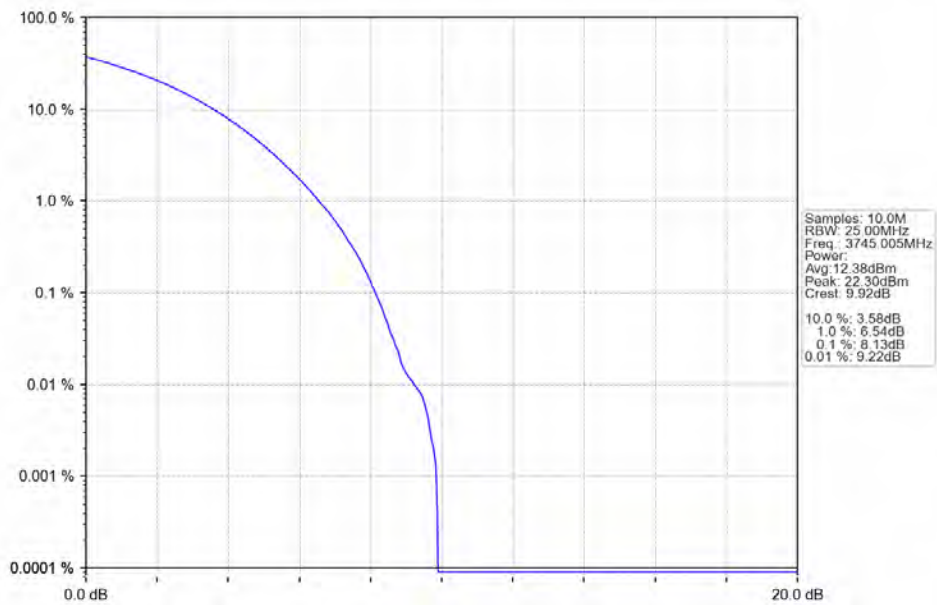
n78a 30kHz SISO NTN 90MHz CP-OFDM 64 QAM 3745.005MHz Outer Full
