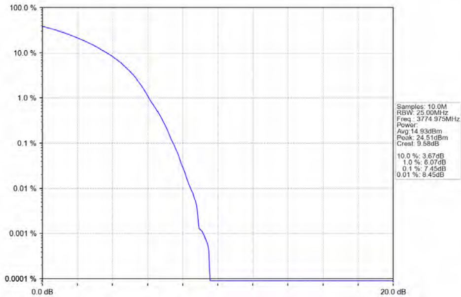
n78a 30kHz SISO NTN 50MHz DFT-s-OFDM 64 QAM 3774.975MHz Outer Full
