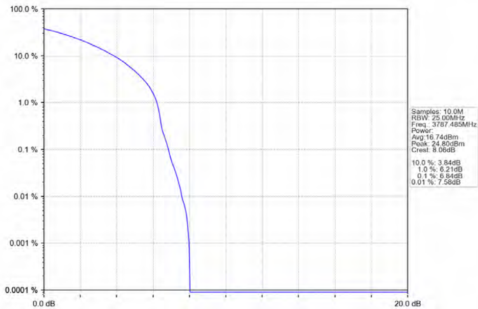
n78a 30kHz SISO NTN 25MHz CP-OFDM 64 QAM 3787.485MHz Outer Full
