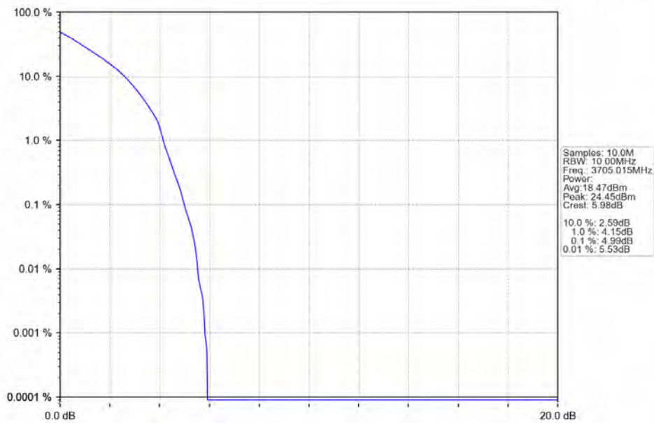
n78a 30kHz SISO NTN 10MHz DFT-s-OFDM QPSK 3705.015MHz Outer Full
