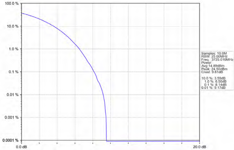
n78a 15kHz SISO NTV 50MHz CP-OFDM 16 QAM 3725.01MHz Outer Full
