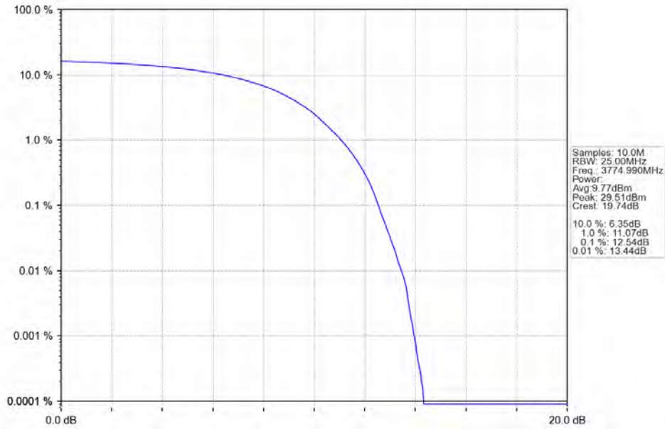
n78a 15kHz SISO NTN 50MHz DFT-s-OFDM PI/2 BPSK 3774.99MHz Outer Full
