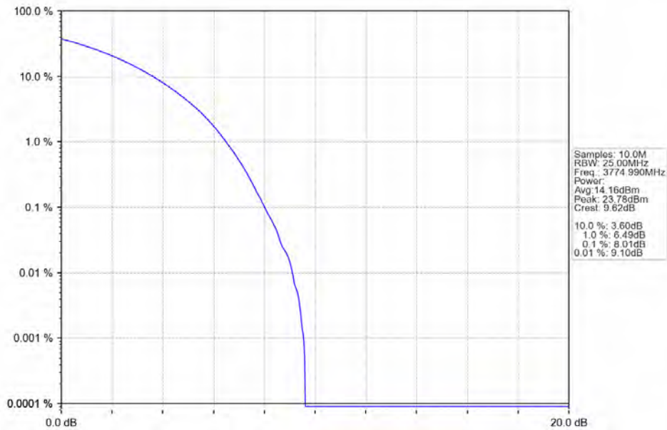
n78a 15kHz SISO NTN 50MHz CP-OFDM 64 QAM 3774.99MHz Outer Full
