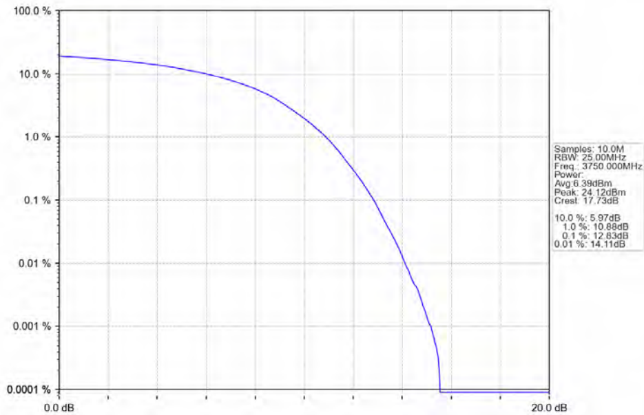
n78a 15kHz SISO NTN 50MHz DFT-s-OFDM 256 QAM 3750MHz Outer Full
