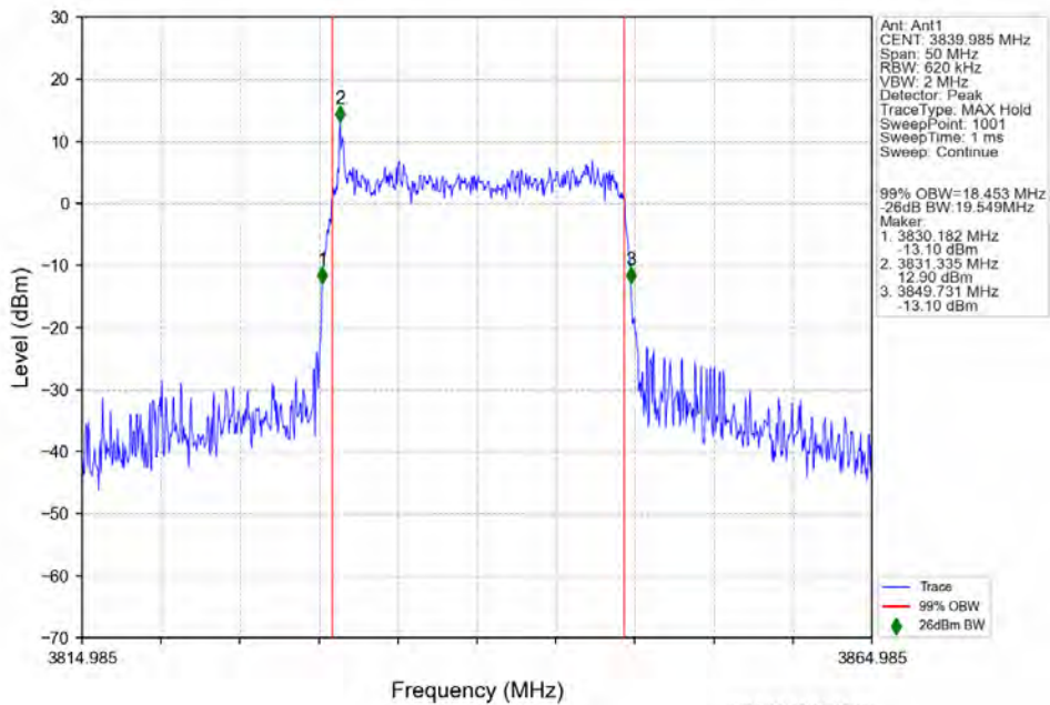
n77a 30kHz SISO NTN 20MHz CP-OFDM 256 QAM 3839.985MHz Outer Full
