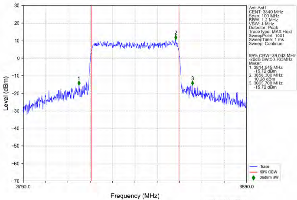
n77a 15kHz SISO NTN 40MHz CP-OFDM 16 QAM 3840MHz Outer Full
