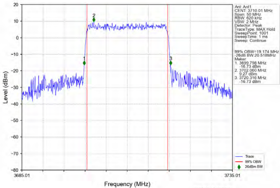
n77a 15kHz SISO NTV 20MHz CP-OFDM 64 QAM 3710.01MHz Outer Full
