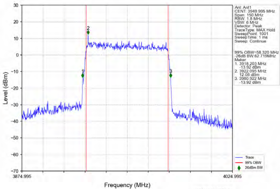
n77a 30kHz SISO NTN 60MHz DFT-s-OFDM QPSK 3949.995MHz Outer Full
