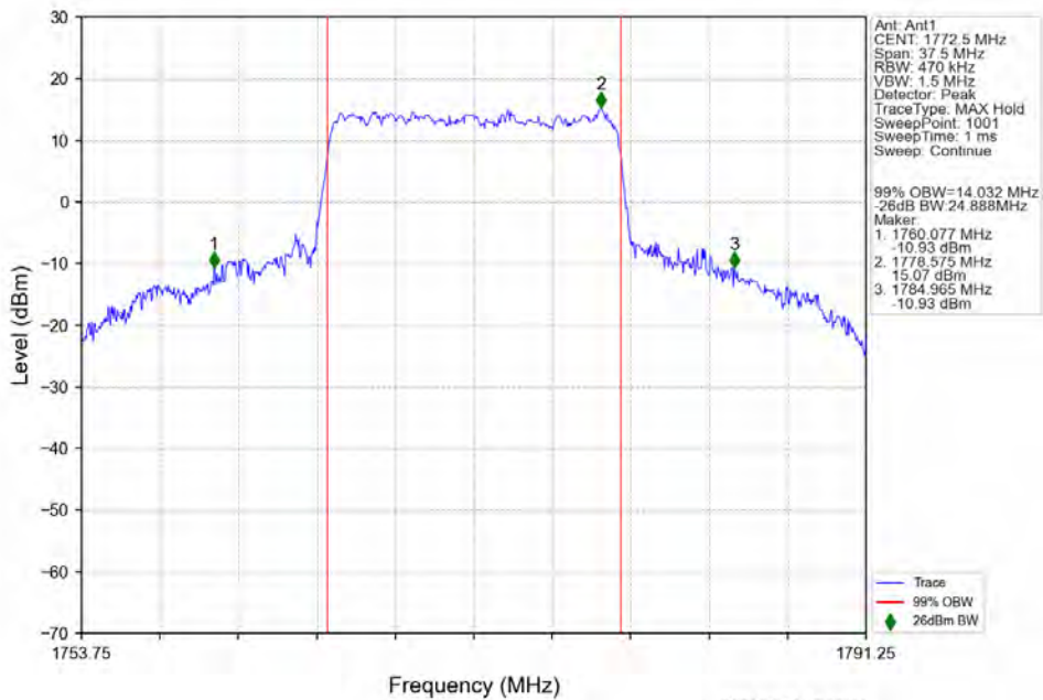
n66 30kHz SISO NTV 15MHz CP-OFDM 64 QAM 1772.5MHz Outer Full
