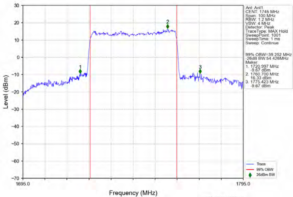
n66 15kHz SISO NTV 40MHz CP-OFDM 16 QAM 1745MHz Outer Full
