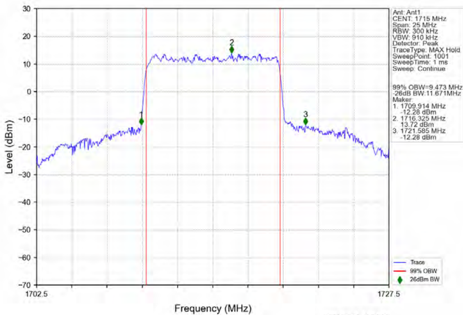
n66 15kHz SISO NTV 10MHz CP-OFDM 64 QAM 1715MHz Outer Full
