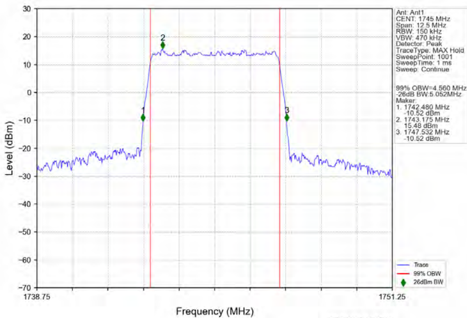
n66 15kHz SISO NTN 5MHz DFT-s-OFDM 16 QAM 1745MHz Outer Full
