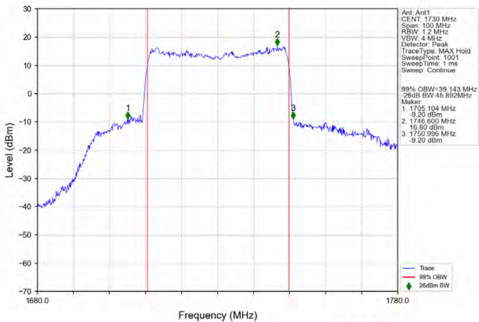
n66 15kHz SISO NTV 40MHz CP-OFDM 64 QAM 1730MHz Outer Full
