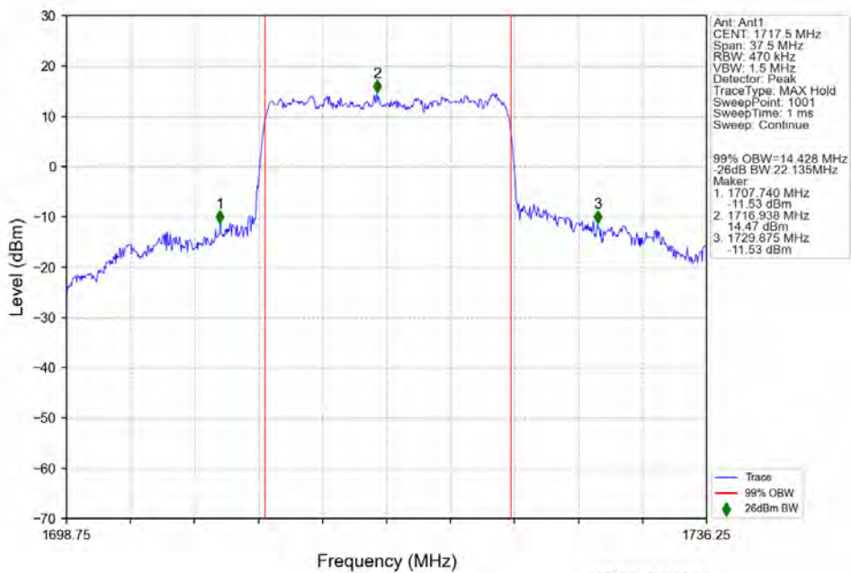
n66 15kHz SISO NTV 15MHz CP-OFDM 64 QAM 1717.5MHz Outer Full
