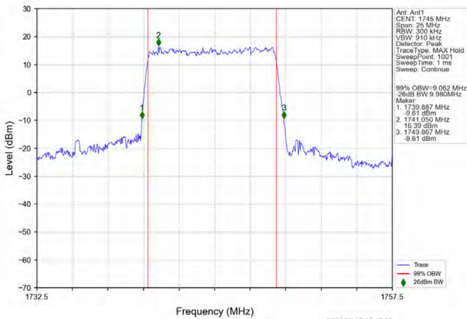
n66 15kHz SISO NTN 10MHz DFT-s-OFDM 16 QAM 1745MHz Outer Full
