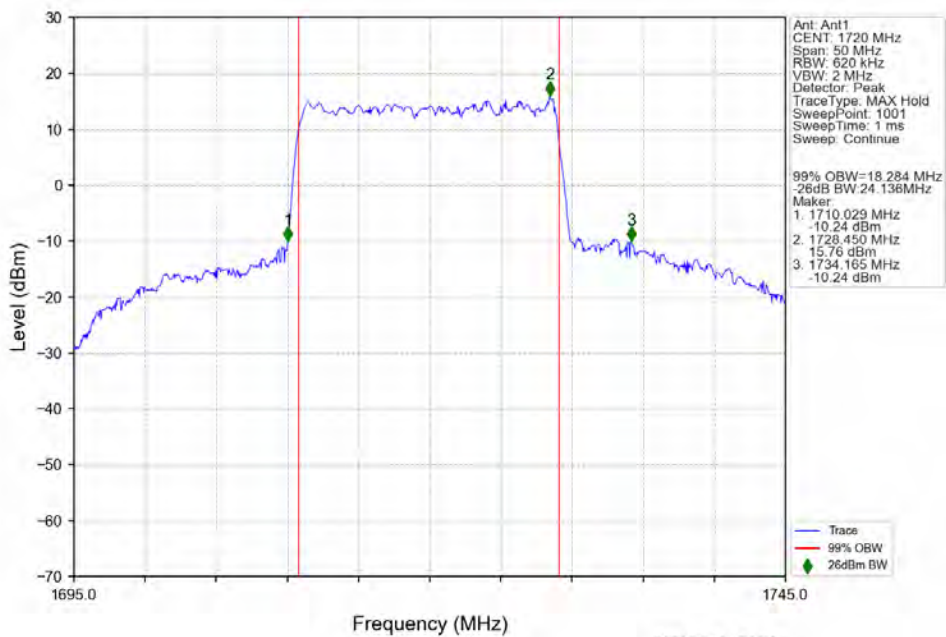
n66 30kHz SISO NTNv 20MHz DFT-s-OFDM 64 QAM 1720MHz Outer Full
