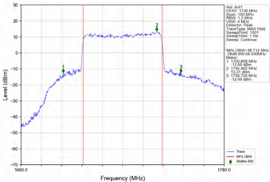
n66 30kHz SISO NTV 40MHz CP-OFDM 64 QAM 1730MHz Outer Full
