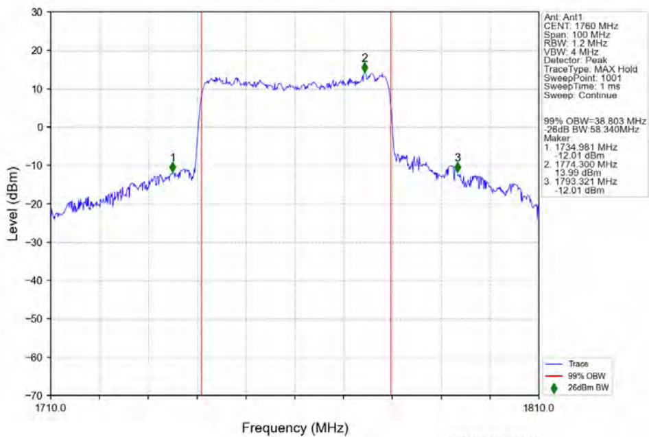
n66 30kHz SISO NTN 40MHz CP-OFDM QPSK 1760MHz Outer Full
