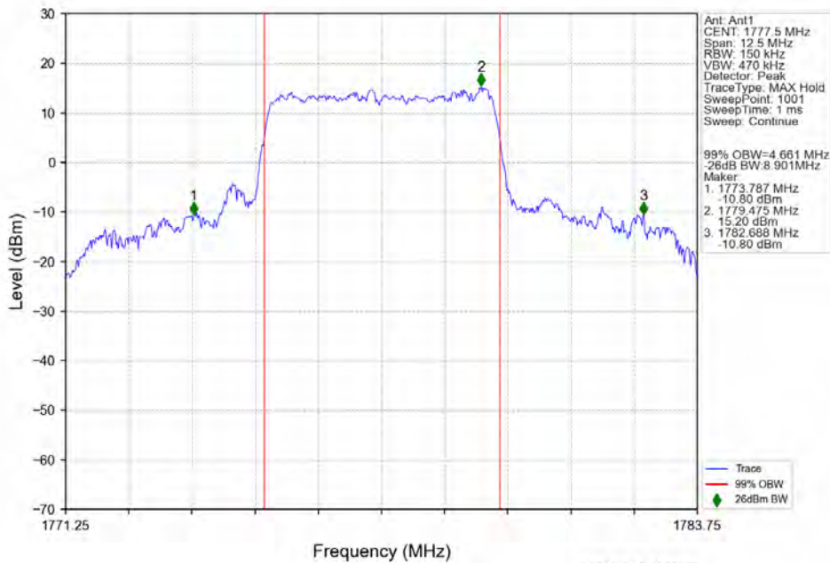
n66 15kHz SISO NTV 5MHz CP-OFDM 64 QAM 1777.5MHz Outer Full
