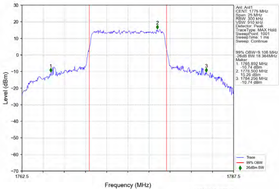
n66 30kHz SISO NTN 10MHz CP-OFDM QPSK 1775MHz Outer Full
