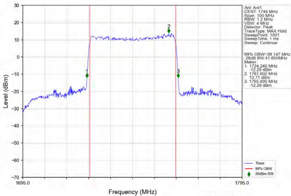
n66 15kHz SISO NTV 40MHz CP-OFDM 256 QAM 1745MHz Outer Full
