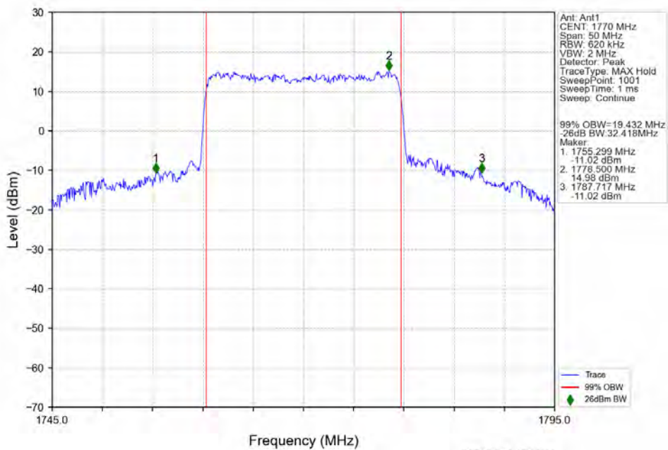
n66 15kHz SISO NTV 20MHz CP-OFDM 64 QAM 1770MHz Outer Full
