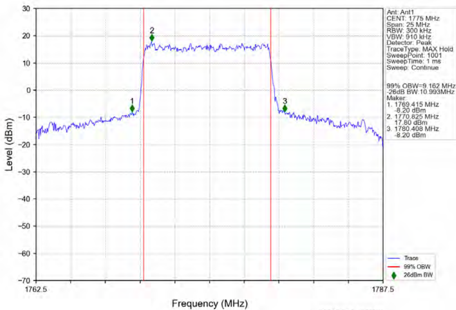
n66 15kHz SISO NTV 10MHz DFT-s-OFDM QPSK 1775MHz Outer Full
