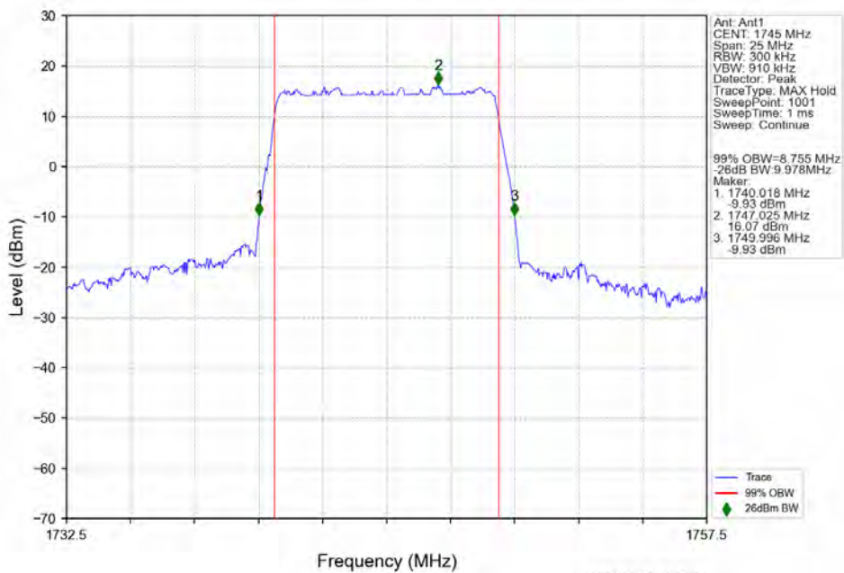
n66 30kHz SISO NTN 10MHz DFT-s-OFDM 16 QAM 1745MHz Outer Full
