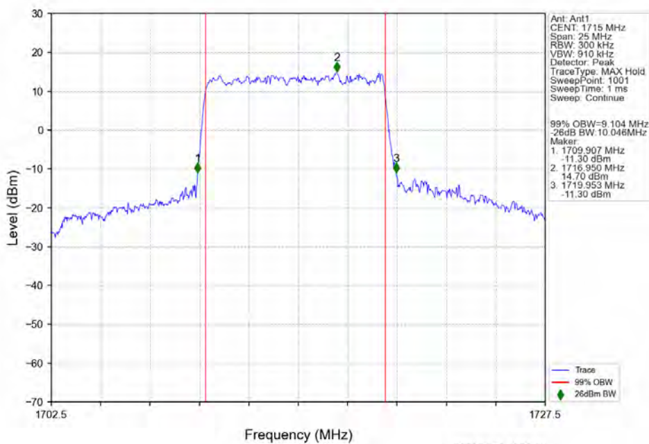
n66 15kHz SISO NTN 10MHz DFT-s-OFDM 64 QAM 1715MHz Outer Full
