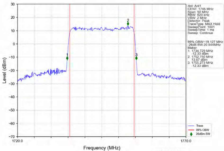
n66 15kHz SISO NTV 20MHz CP-OFDM 256 QAM 1745MHz Outer Full
