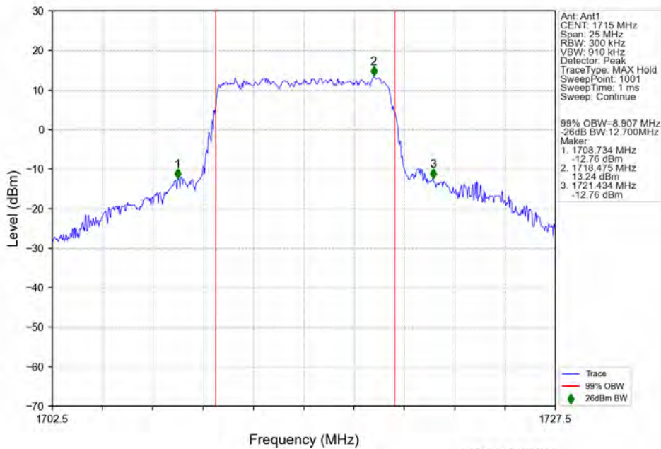
n66 30kHz SISO NTV 10MHz CP-OFDM 64 QAM 1715MHz Outer Full
