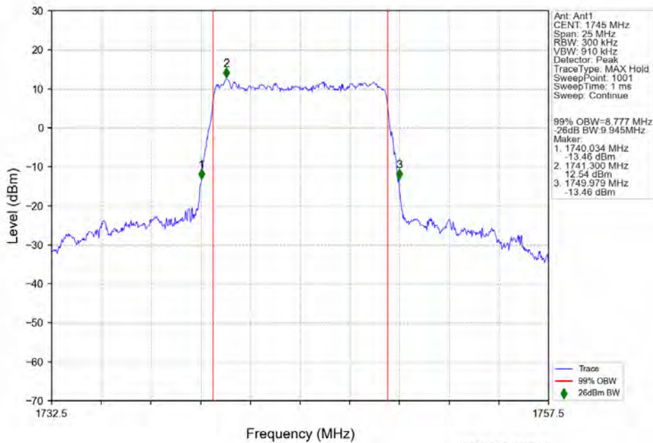
n66 30kHz SISO NTV 10MHz CP-OFDM 256 QAM 1745MHz Outer Full
