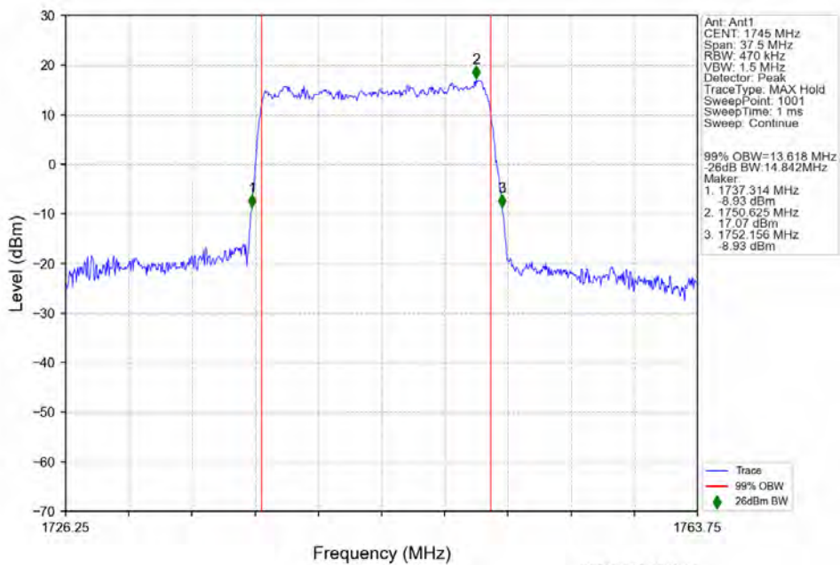
n66 15kHz SISO NTNv 15MHz DFT-s-OFDM 16 QAM 1745MHz Outer Full
