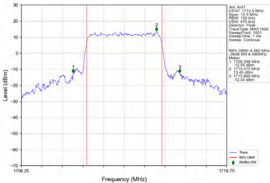
n66 15kHz SISO NTV 5MHz CP-OFDM 64 QAM 1712.5MHz Outer Full
