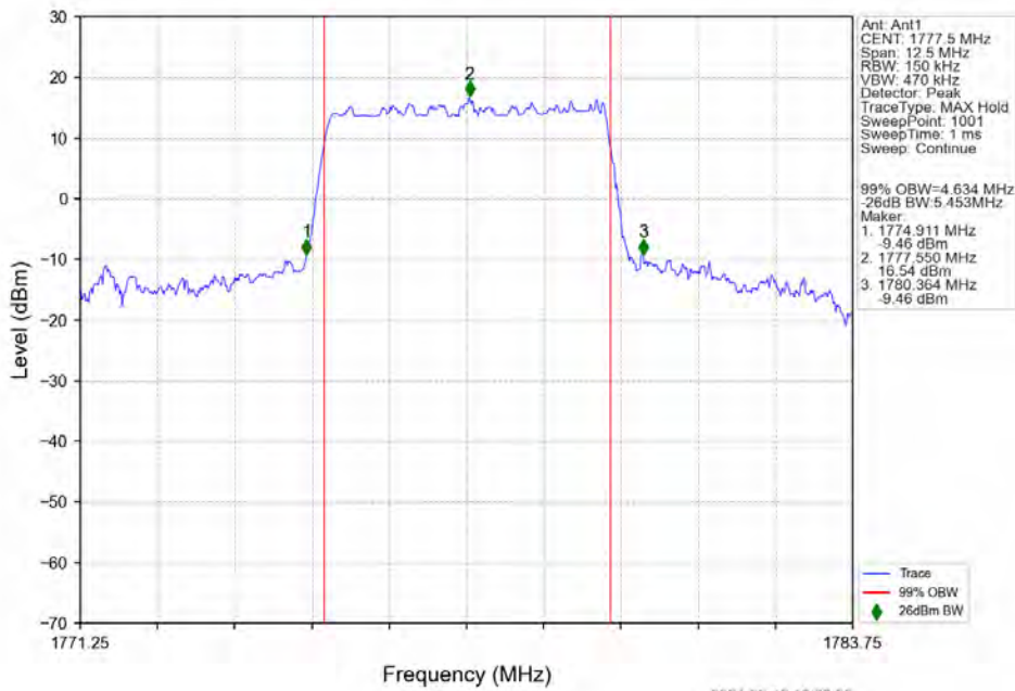
n66 15kHz SISO NTV 5MHz DFT-s-OFDM 64 QAM 1777.5MHz Outer Full
