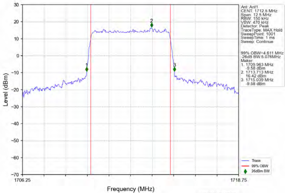
n66 15kHz SISO NTN 5MHz DFT-s-OFDM QPSK 1712.5MHz Outer Full
