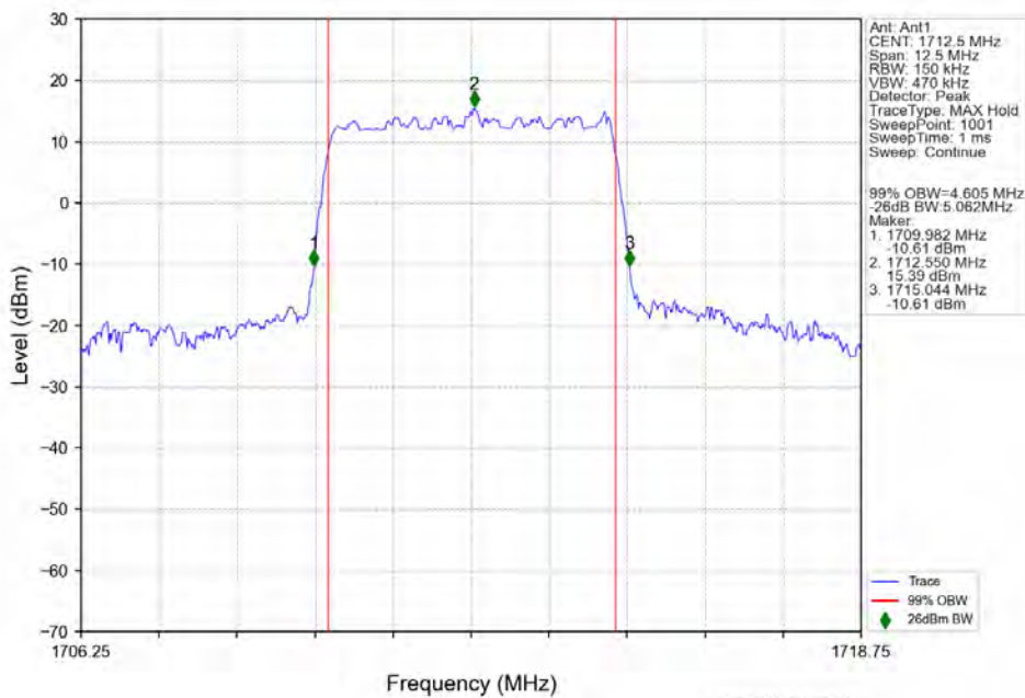
n66 15kHz SISO NTNv 5MHz DFT-s-OFDM 64 QAM 1712.5MHz Outer Full
