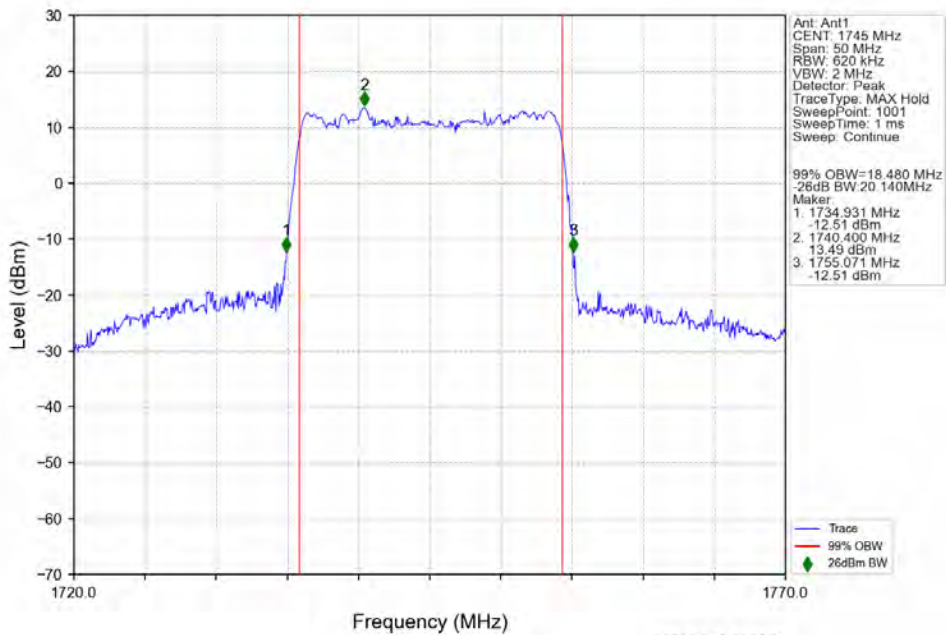
n66 30kHz SISO NTV 20MHz CP-OFDM 256 QAM 1745MHz Outer Full
