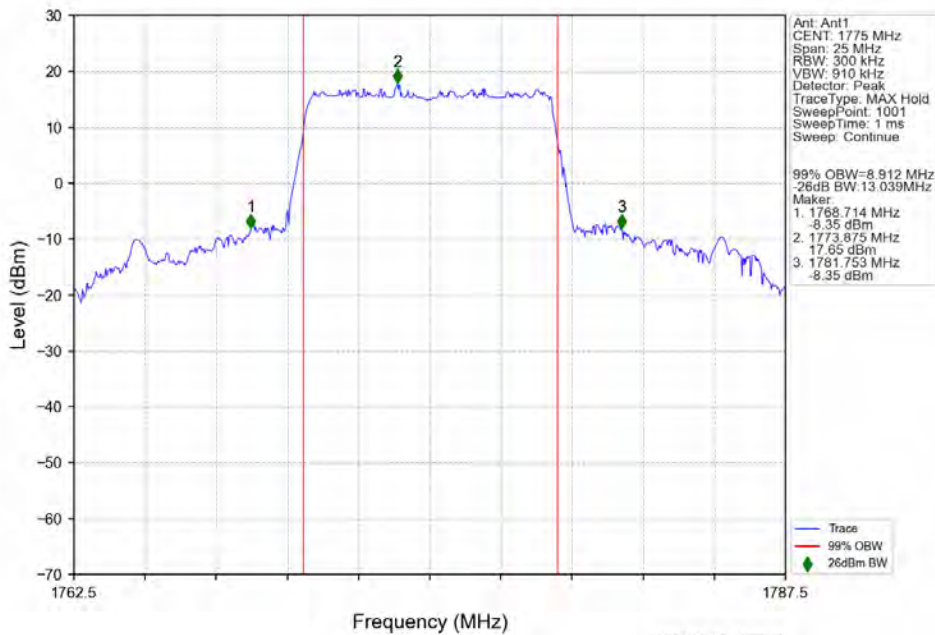
n66 30kHz SISO NTN 10MHz DFT-s-OFDM QPSK 1775MHz Outer Full
