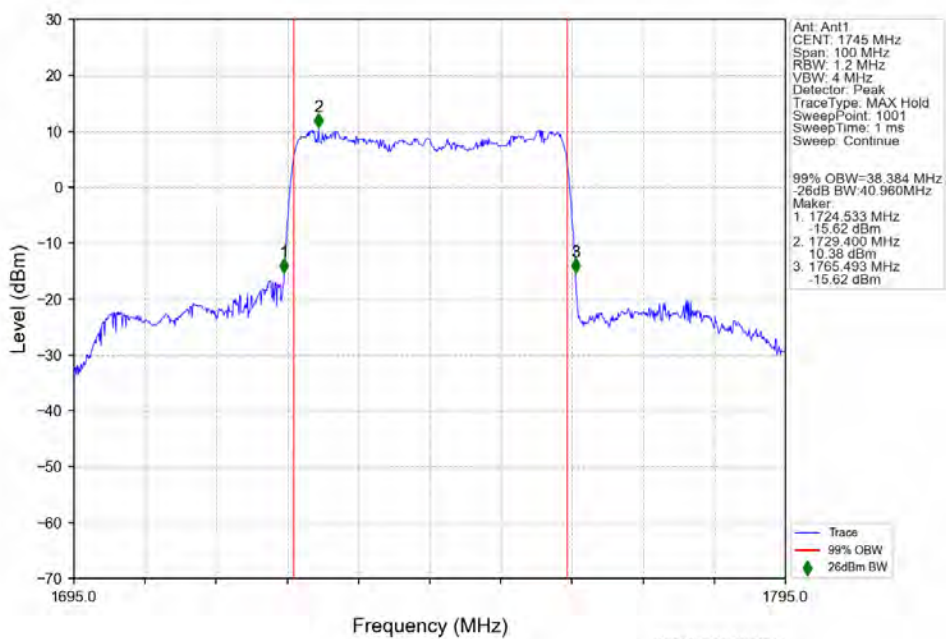
n66 30kHz SISO NTV 40MHz CP-OFDM 256 QAM 1745MHz Outer Full
