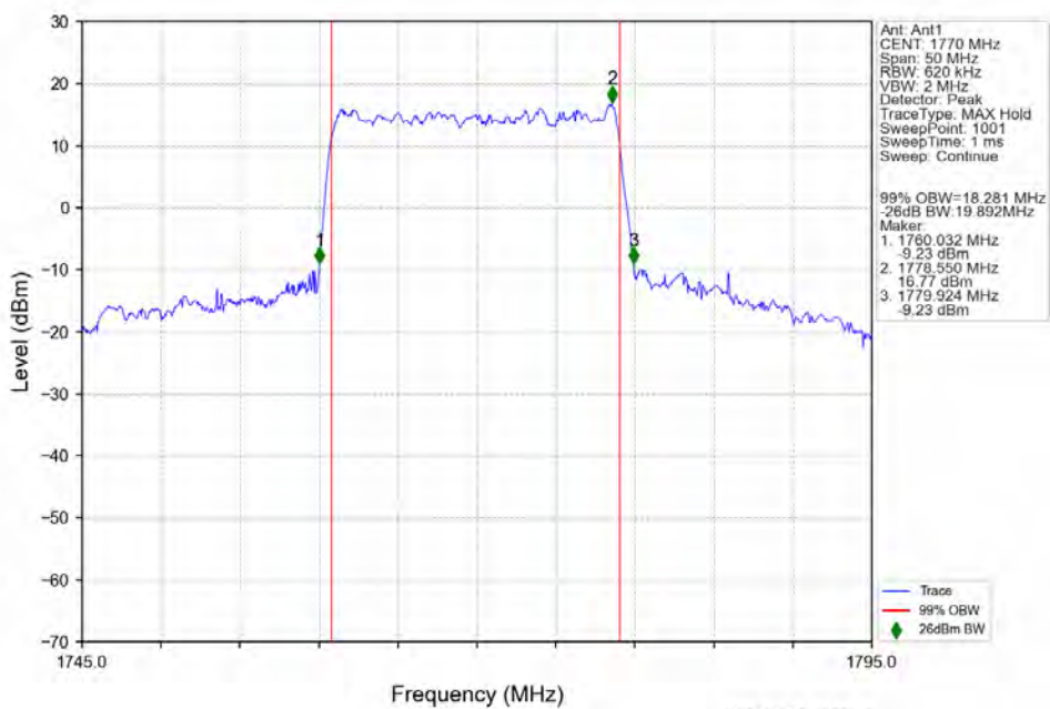
n66 30kHz SISO NTN 20MHz DFT-s-OFDM 64 QAM 1770MHz Outer Full
