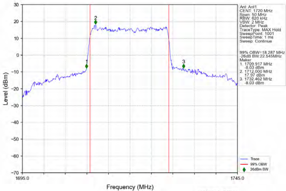
n66 30kHz SISO NTV 20MHz DFT-s-OFDM QPSK 1720MHz Outer Full
