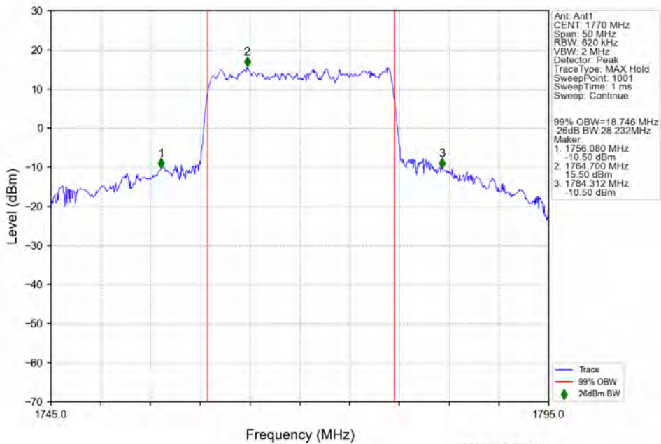
n66 30kHz SISO NTV 20MHz CP-OFDM 64 QAM 1770MHz Outer Full
