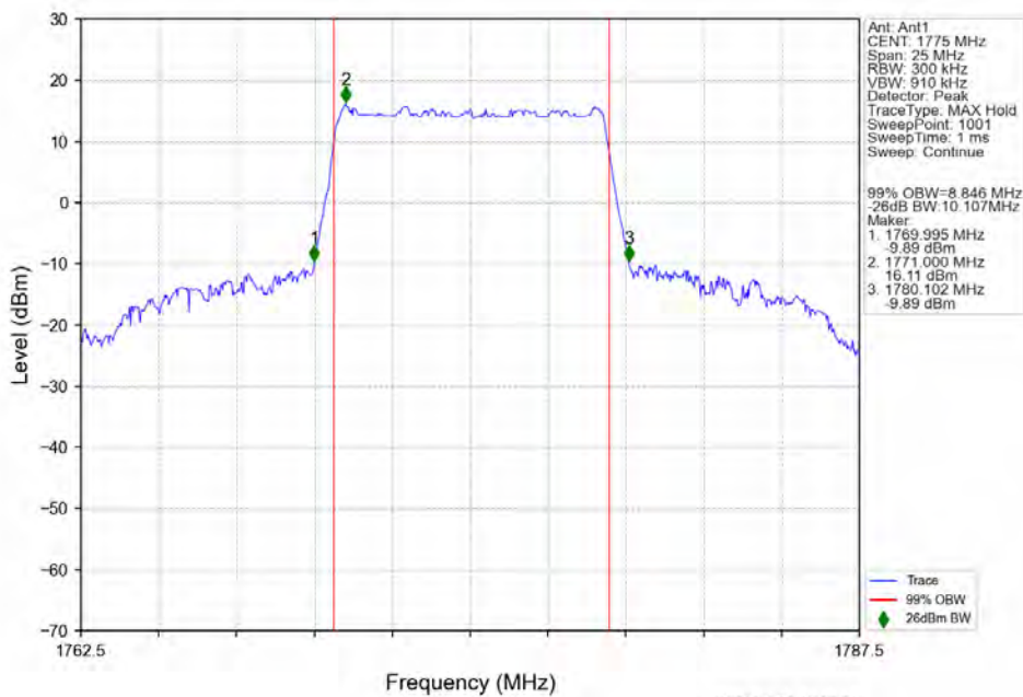
n66 30kHz SISO NTN 10MHz DFT-s-OFDM 64 QAM 1775MHz Outer Full
