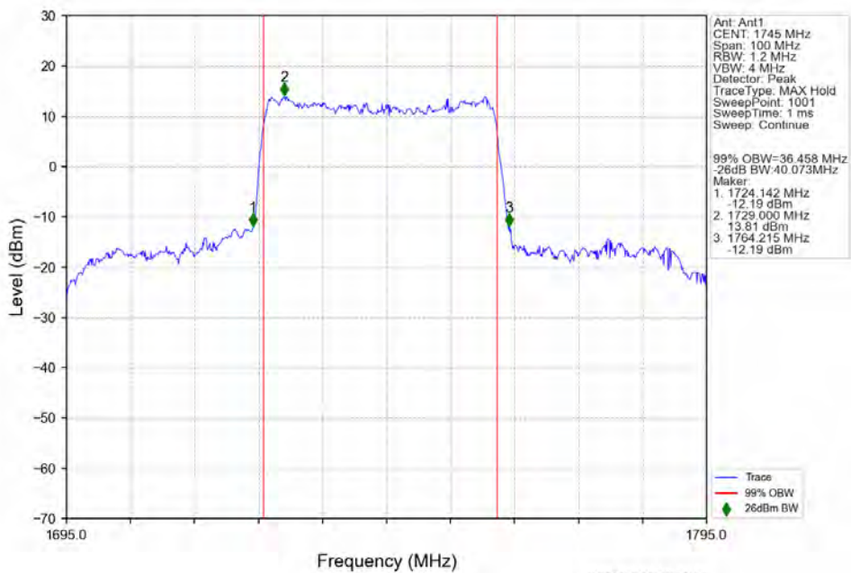
n66 30kHz SISO NTN 40MHz DFT-s-OFDM 16 QAM 1745MHz Outer Full
