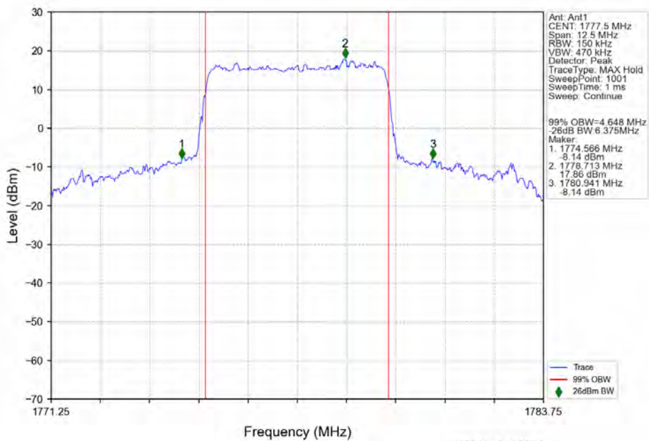
n66 15kHz SISO NTN 5MHz DFT-s-OFDM QPSK 1777.5MHz Outer Full
