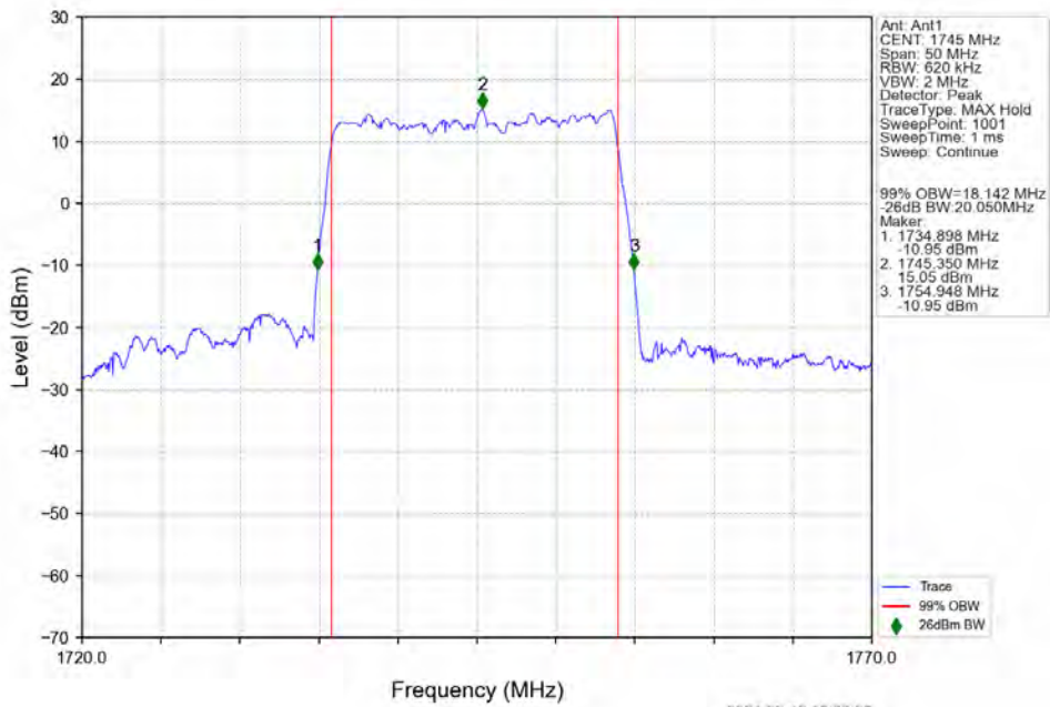
n66 30kHz SISO NTVN 20MHz DFT-s-OFDM 256 QAM 1745MHz Outer Full
