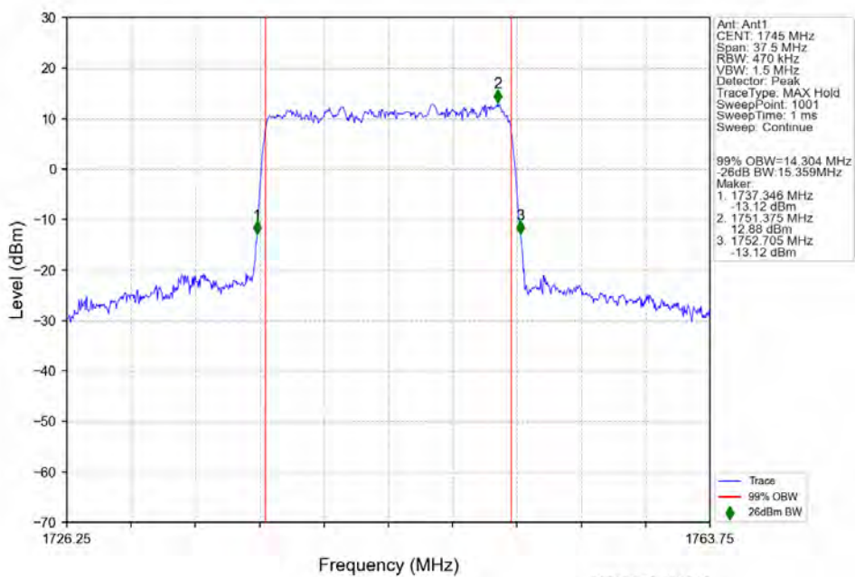
n66 15kHz SISO NTN 15MHz CP-OFDM 256 QAM 1745MHz Outer Full
