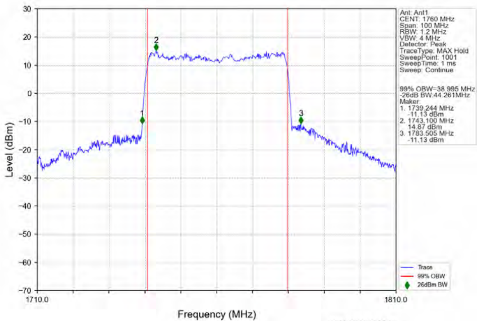
n66 15kHz SISO NTV 40MHz CP-OFDM 64 QAM 1760MHz Outer Full
