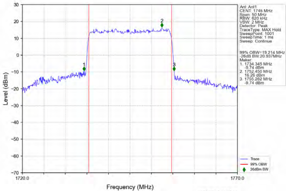
n66 15kHz SISO NTV 20MHz CP-OFDM 16 QAM 1745MHz Outer Full
