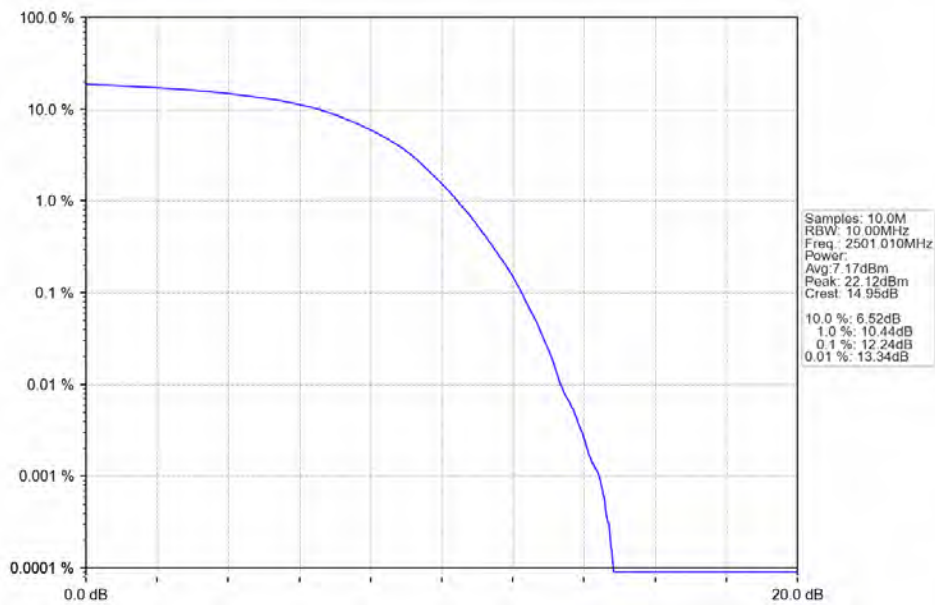
n41 15kHz SISO NTN 10MHz DFT-s-OFDM 256 QAM 2501.01MHz Outer Full
