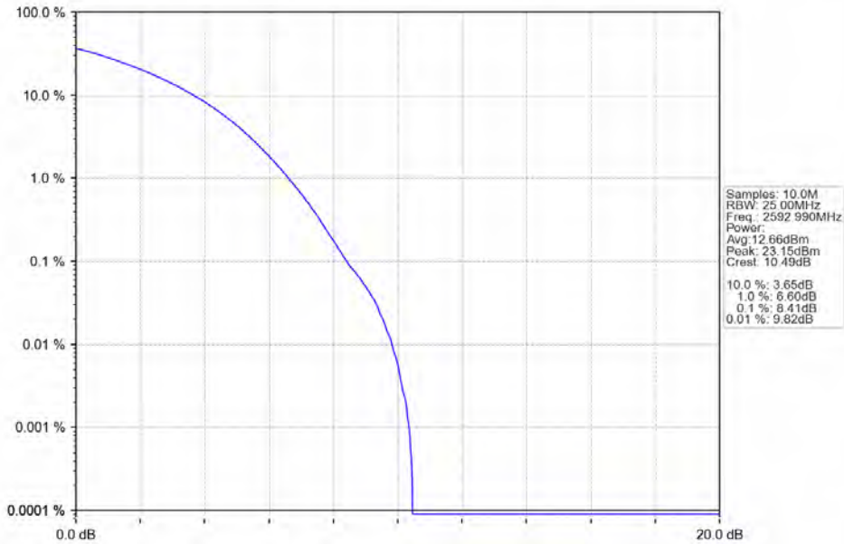
n41 30kHz SISO NTV 100MHz CP-OFDM 16 QAM 2592.99MHz Outer Full
