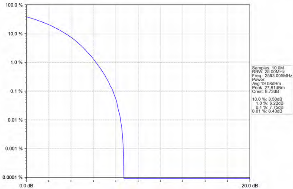
n41 15kHz SISO NTN 15MHz CP-OFDM QPSK 2593.005MHz Outer Full
