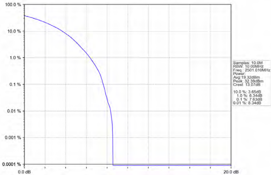
n41 15kHz SISO NTN 10MHz CP-OFDM 16 QAM 2501.01MHz Outer Full
