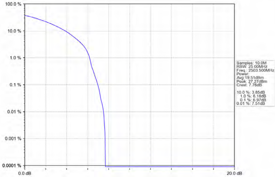
n41 30kHz SISO NTN 15MHz CP-OFDM QPSK 2503.5MHz Outer Full
