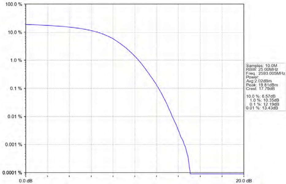
n41 15kHz SISO NTN 15MHz DFT-s-OFDM 256 QAM 2593.005MHz Outer Full
