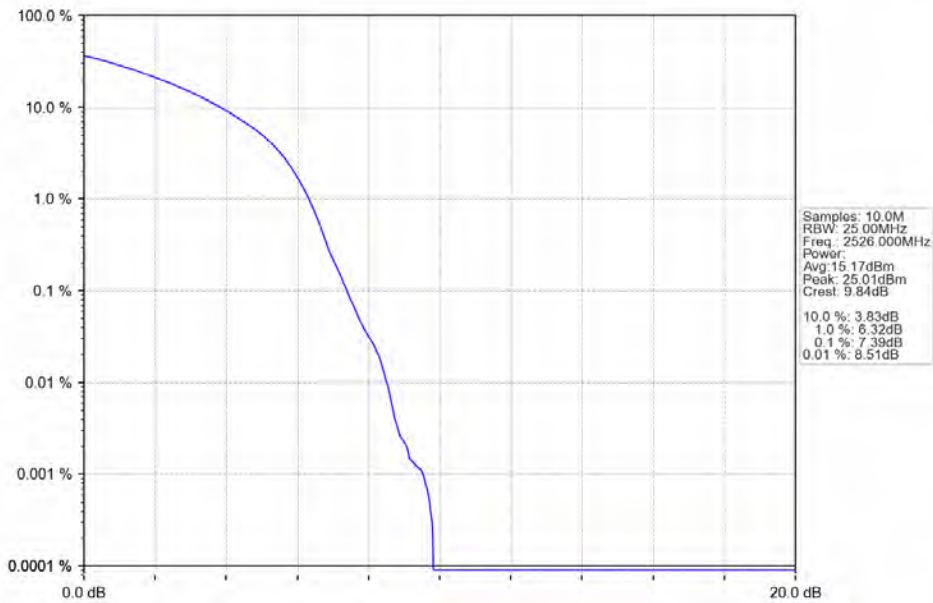
n41 30kHz SISO NTN 60MHz DFT-s-OFDM 16 QAM 2526MHz Outer Full
