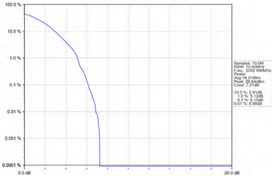
n41 30kHz SISO NTN 10MHz DFT-s-OFDM 64 QAM 2592.99MHz Outer Full
