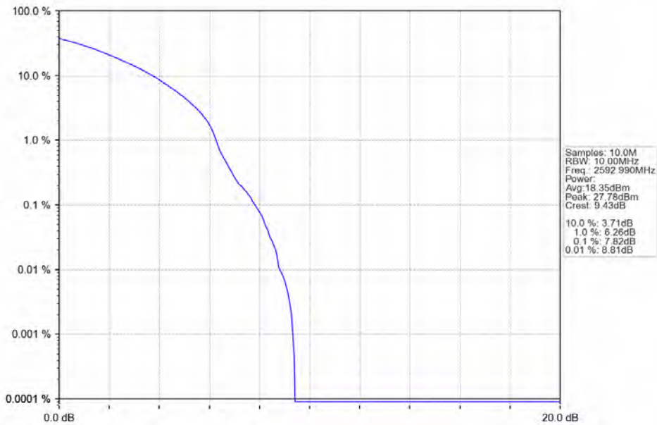
n41 30kHz SISO NTN 10MHz CP-OFDM 64 QAM 2592.99MHz Outer Full
