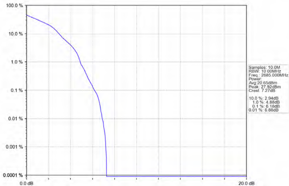
n41 30kHz SISO NTN 10MHz DFT-s-OFDM 16 QAM 2685MHz Outer Full
