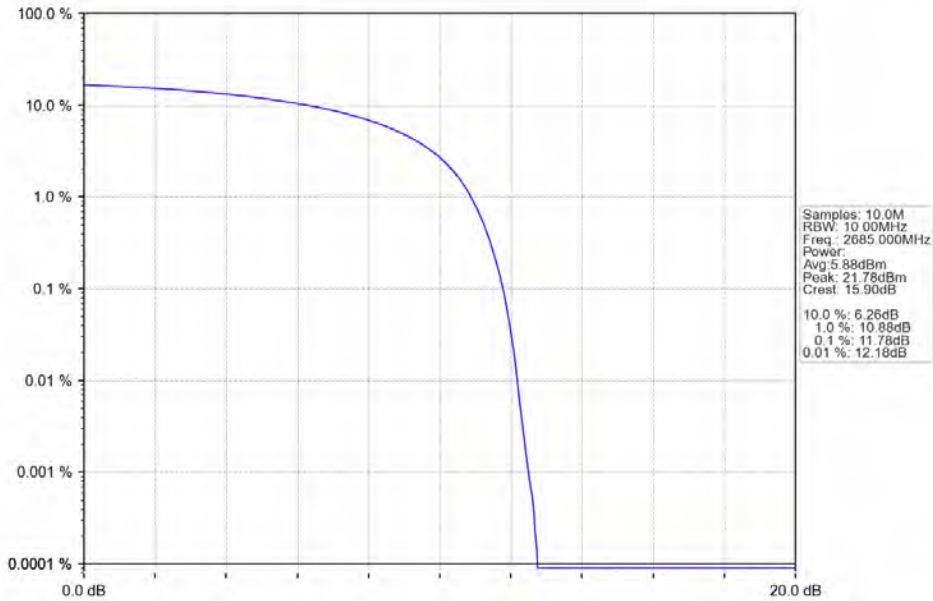
n41 15kHz SISO NTN 10MHz CP-OFDM QPSK 2685MHz Outer Full
