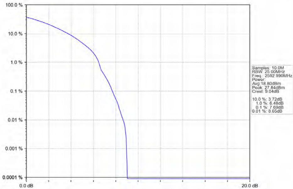
n41 30kHz SISO NTN 20MHz CP-OFDM 64 QAM 2592.99MHz Outer Full
