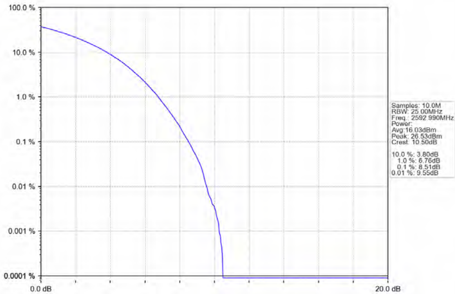
n41 30kHz SISO NTN 50MHz CP-OFDM 64 QAM 2592.99MHz Outer Full
