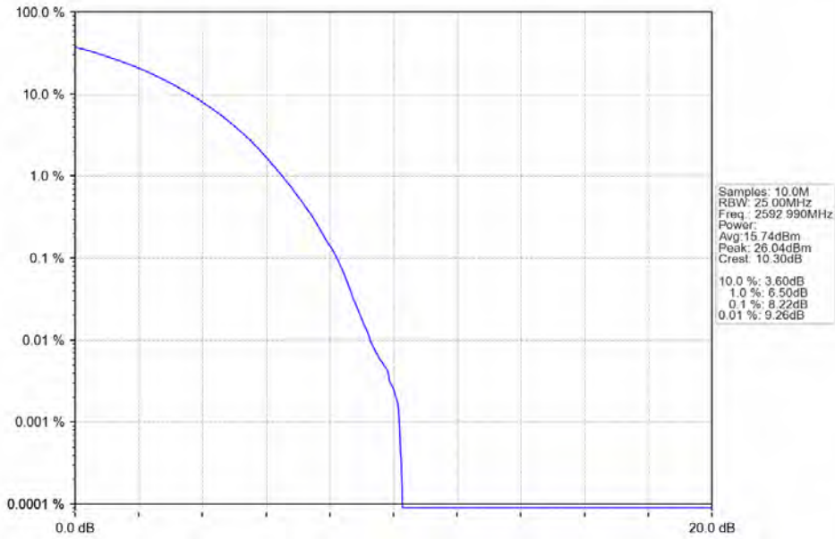
n41 30kHz SISO NTN 60MHz CP-OFDM 16 QAM 2592.99MHz Outer Full
