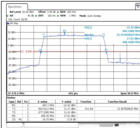
Band71-15MHz-QPSK-133197-75RB#0-PASS
