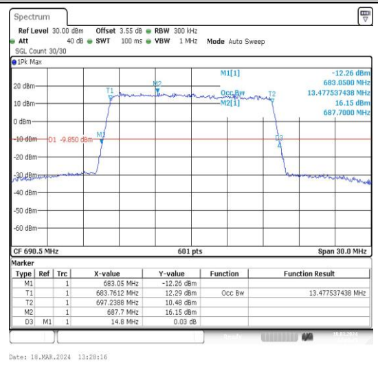
Band71-15MHz-16QAM-133397-75RB#0-PASS
