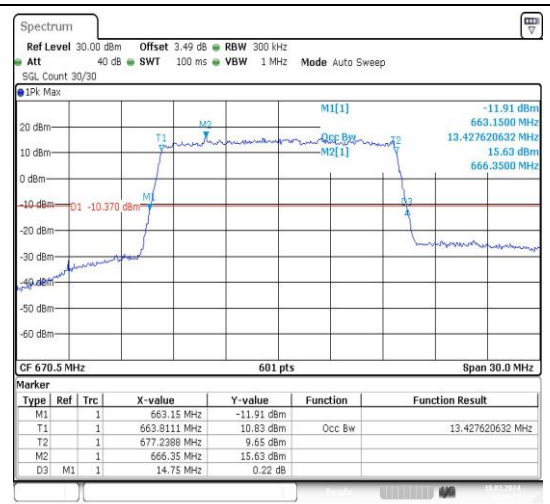
Band71-15MHz-16QAM-133197-75RB#0-PASS
