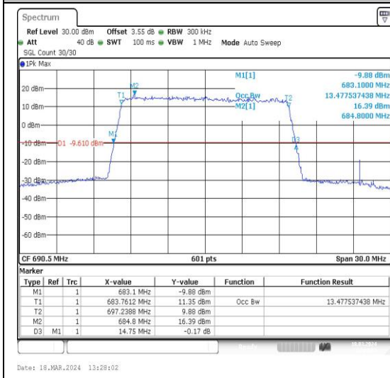
Band71-15MHz-QPSK-133397-75RB#0-PASS
