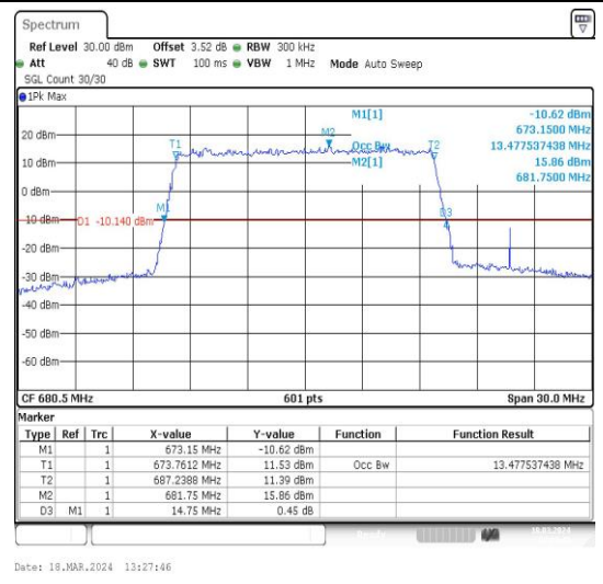
Band71-15MHz-16QAM-133297-75RB#0-PASS
