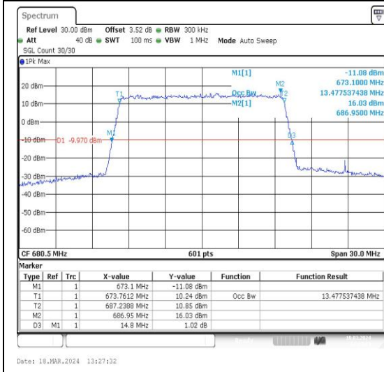
Band71-15MHz-QPSK-133297-75RB#0-PASS
