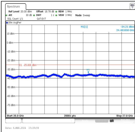
Band41_15MHz_QPSK_40620_1RB#0_20000~27000_20000~27000
