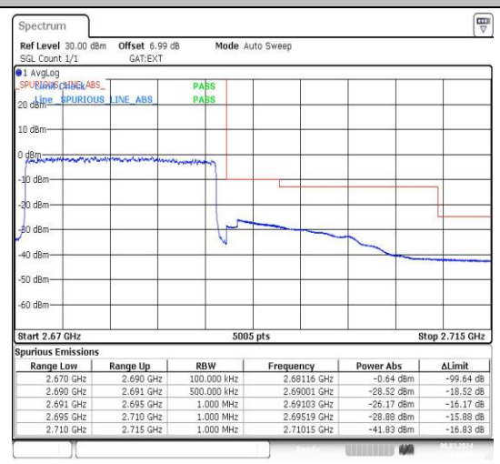
Band41_20MHz_16QAM_41490_1RB#99
