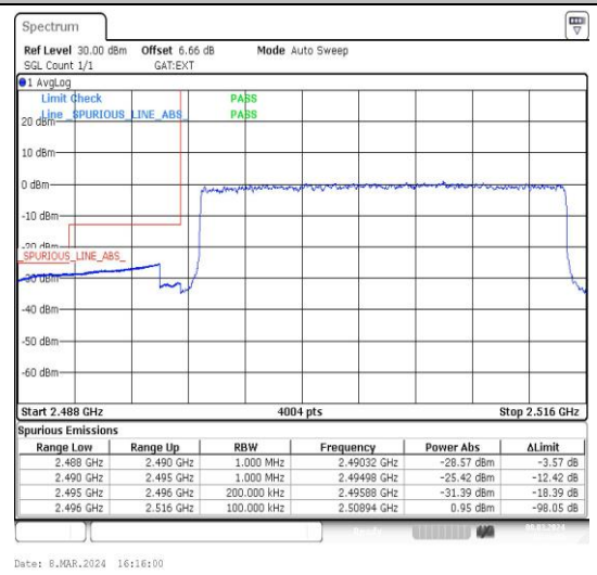
Band41_20MHz_16QAM_39750_100RB#0
