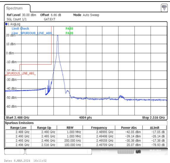
Band41_20MHz_16QAM_39750_1RB#0
