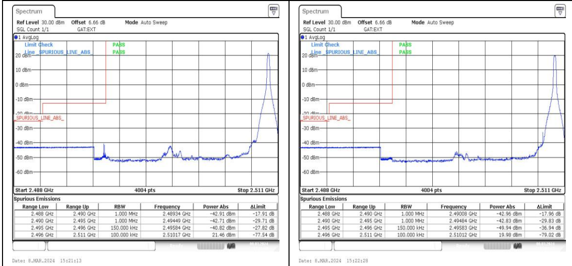
Band41_15MHz_QPSK_39725_1RB#74 Band41_15MHz_16QAM_39725_1RB#74
