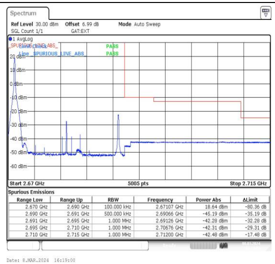
Band41_20MHz_16QAM_41490_1RB#0
