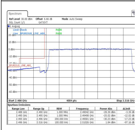
Band41_20MHz_QPSK_39750_100RB#0
