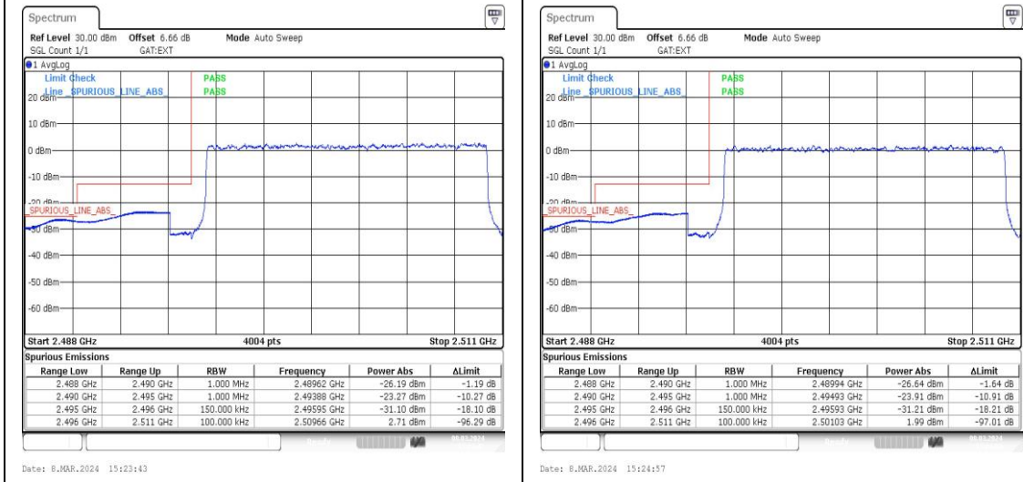
Band41_15MHz_QPSK_39725_75RB#0 Band41_15MHz_16QAM_39725_75RB#0
