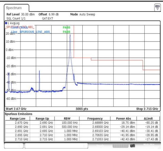
Band41_20MHz_16QAM_41490_1RB#0
