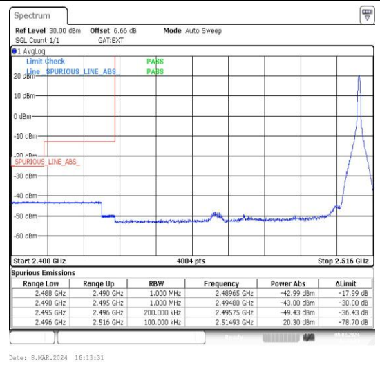
Band41_20MHz_16QAM_39750_1RB#99
