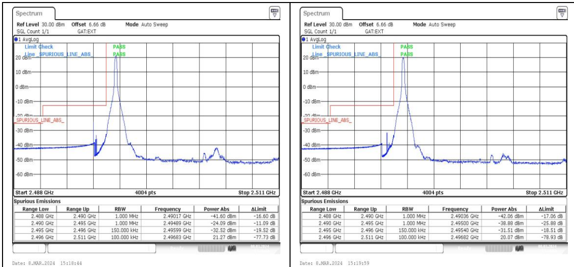
Band41_15MHz_QPSK_39725_1RB#0 Band41_15MHz_16QAM_39725_1RB#0
