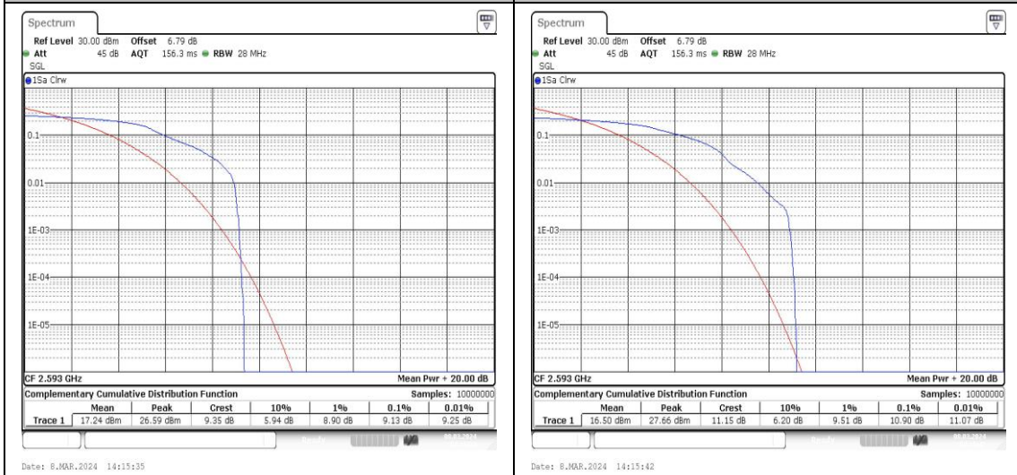
Band41-5MHz-QPSK-40620-1RB#0-PASS Band41-5MHz-16QAM-40620-1RB#0-PASS
