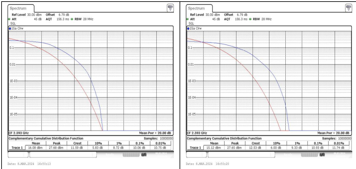
Band41-20MHz-QPSK-40620-100RB#0-PASS Band41-20MHz-16QAM-40620-100RB#0-PASS
