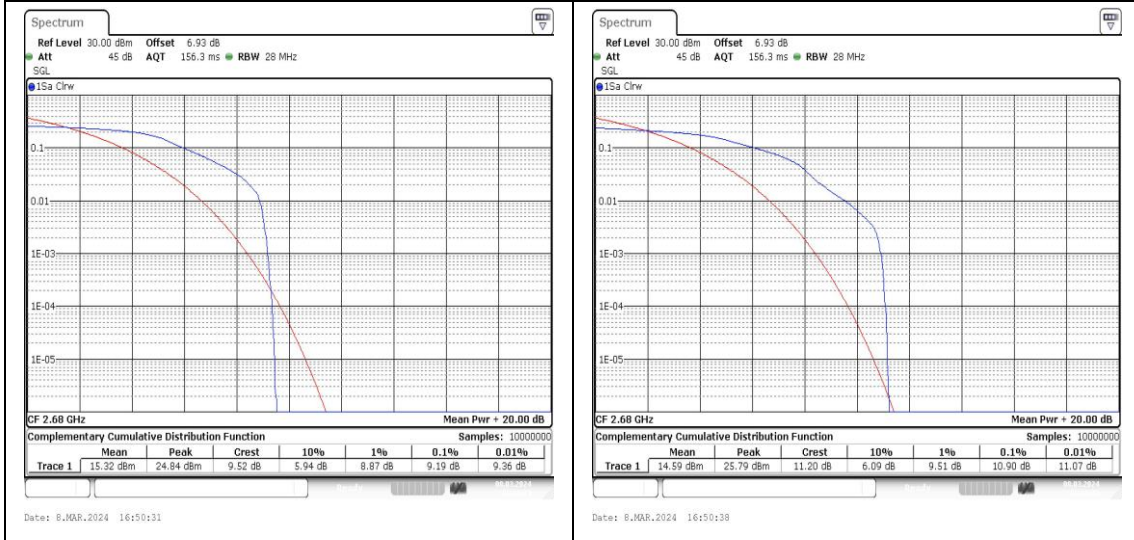
Band41-20MHz-QPSK-41490-1RB#0-PASS Band41-20MHz-16QAM-41490-1RB#0-PASS
