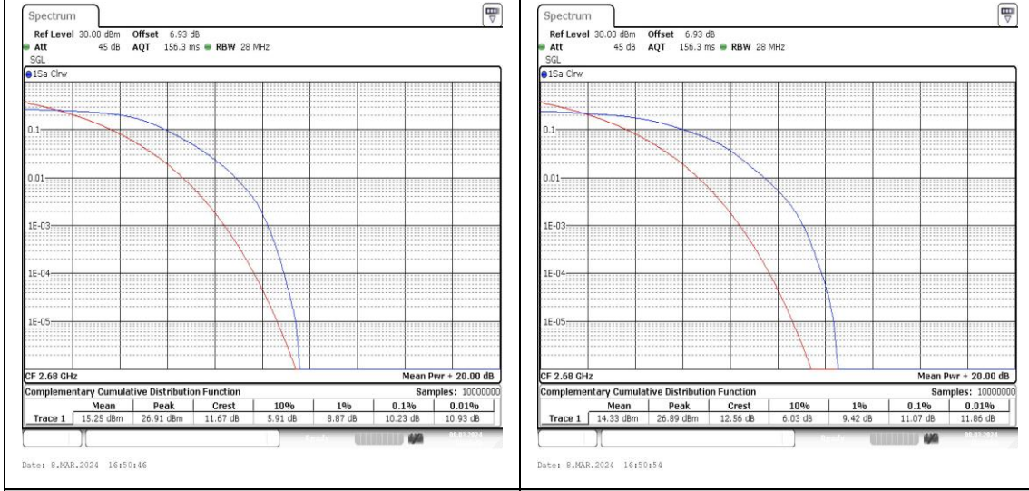
Band41-20MHz-QPSK-41490-100RB#0-PASS Band41-20MHz-16QAM-41490-100RB#0-PASS
