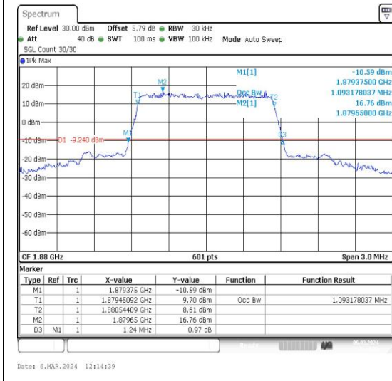
Band2-1.4MHz-QPSK-18900-6RB#0-PASS
