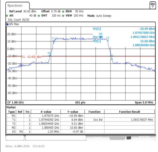
Band2-1.4MHz-16QAM-18900-6RB#0-PASS
