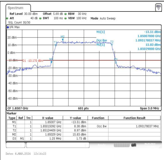
Band2-1.4MHz-16QAM-18607-6RB#0-PASS
