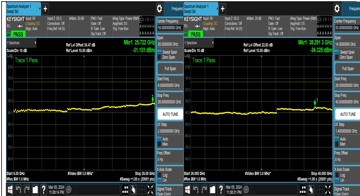
NTNV_DC_13A_n77A-3450-3550_PC3_30_5+20 _M+M_TID19_NS_01_0.009_0.15_#1
