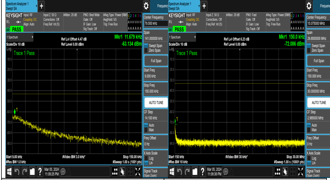
NTNV_DC_13A_n77A-3450-3550_PC3_30_5+20 _M+M_TID19_NS_01_30_1000_#1
