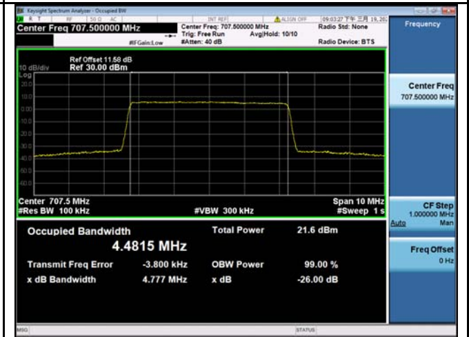
LTE band 12 - Middle CH 16QAM-5
