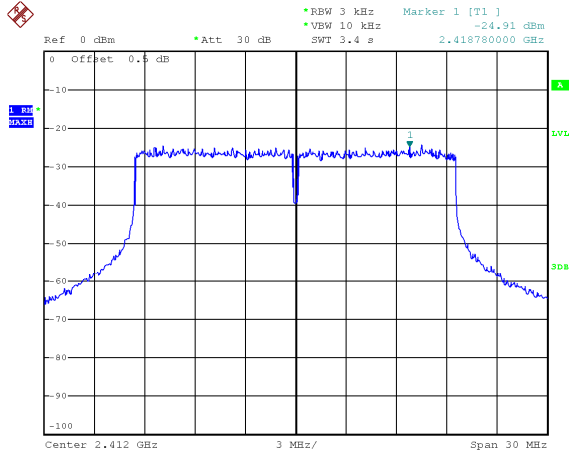
Mode: TX 11ax HT20 channel 1
