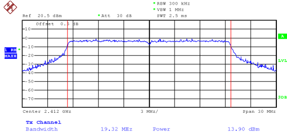
Mode: TX 11ax HT20 channel 1
