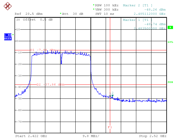
TX 11ax HT40: Band edge-right side
