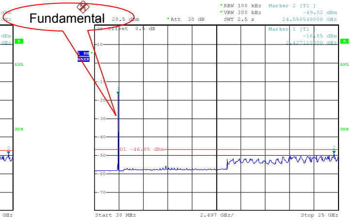
Mode: TX 11g channel 6
