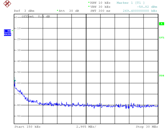
Mode: TX 11 ax HT20 channel 11
