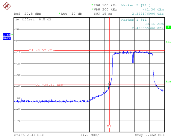
TX 11ax HT40: Band edge-left side
