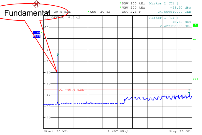
Mode: TX 11 ax HT20 channel 6
