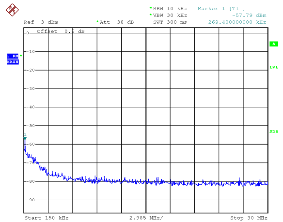
Mode: TX 11 ax HT20 channel 6
