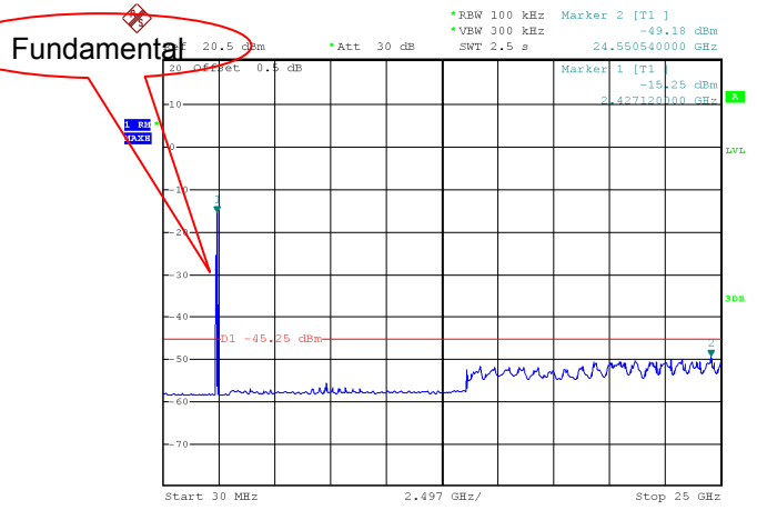
Mode: TX 11 ax HT40 channel 6
