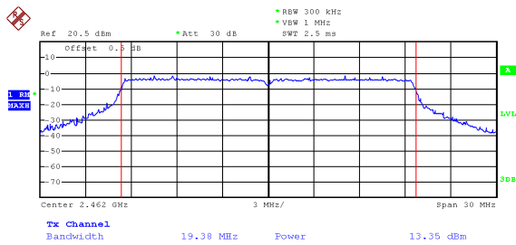
Mode: TX 11ax HT20 channel 11
