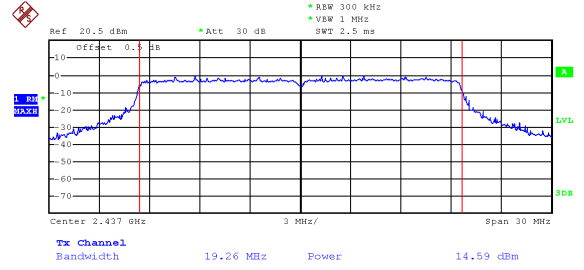
Mode: TX 11ax HT20 channel 6
