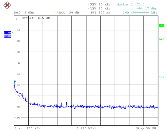
Mode: TX 11 ax HT40 channel 9
