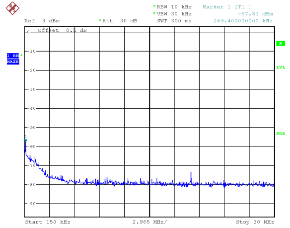
Mode: TX 11 ax HT40 channel 6
