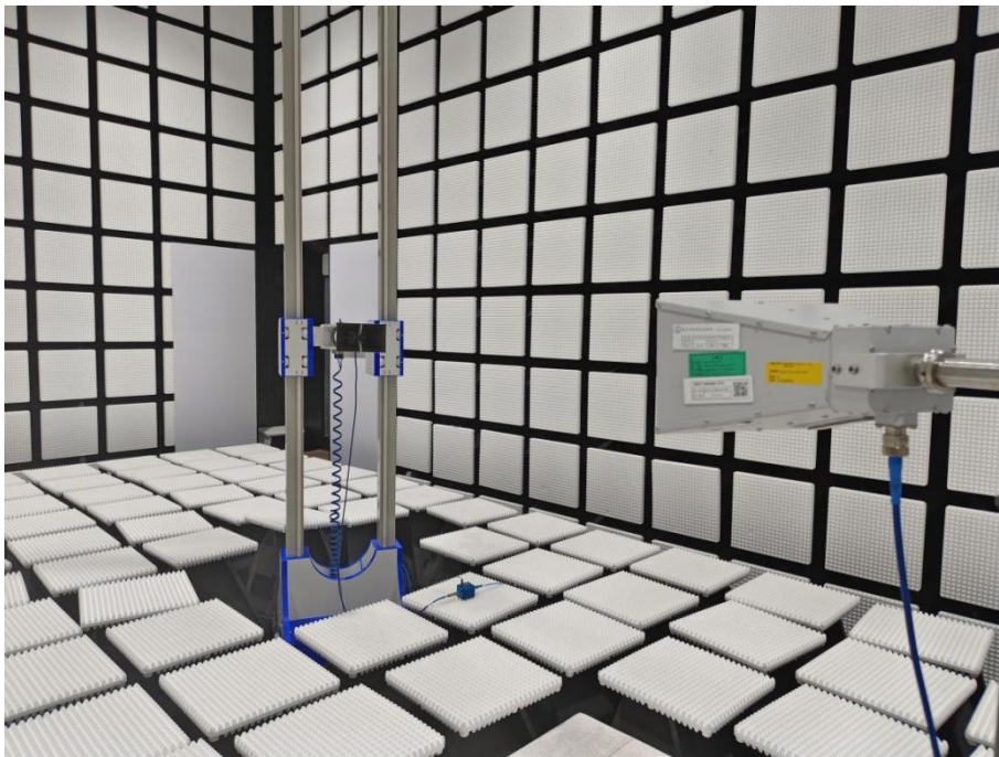
Description: substitution Antenna for Radiated Emissions above 1GHz Test Setup
