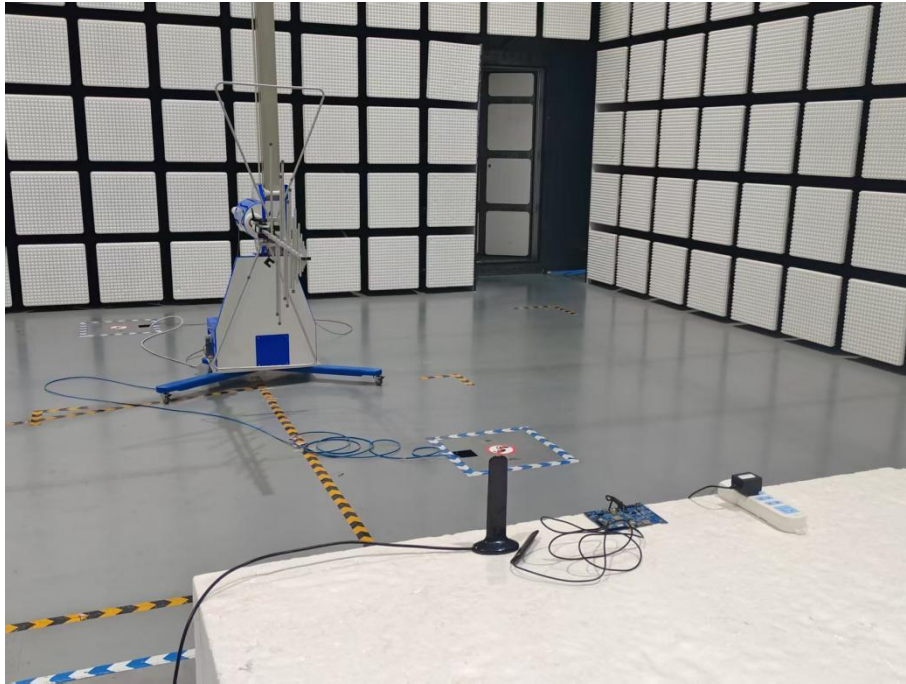
Description: Radiated Emissions below 1GHz Test Setup
