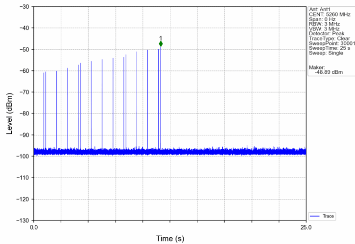
Signal Calibration_802.11a_2A_5260MHz_RadarType5_Trial0
