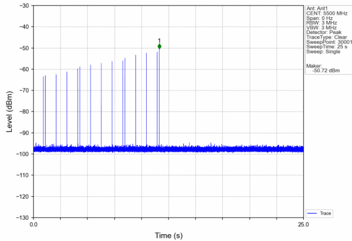
Signal Calibration_802.11a_2C_5500MHz_RadarType5_Trial0
