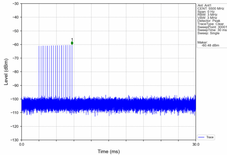
Signal Calibration_802.11a_2C_5500MHz_RadarType3_Trial0
