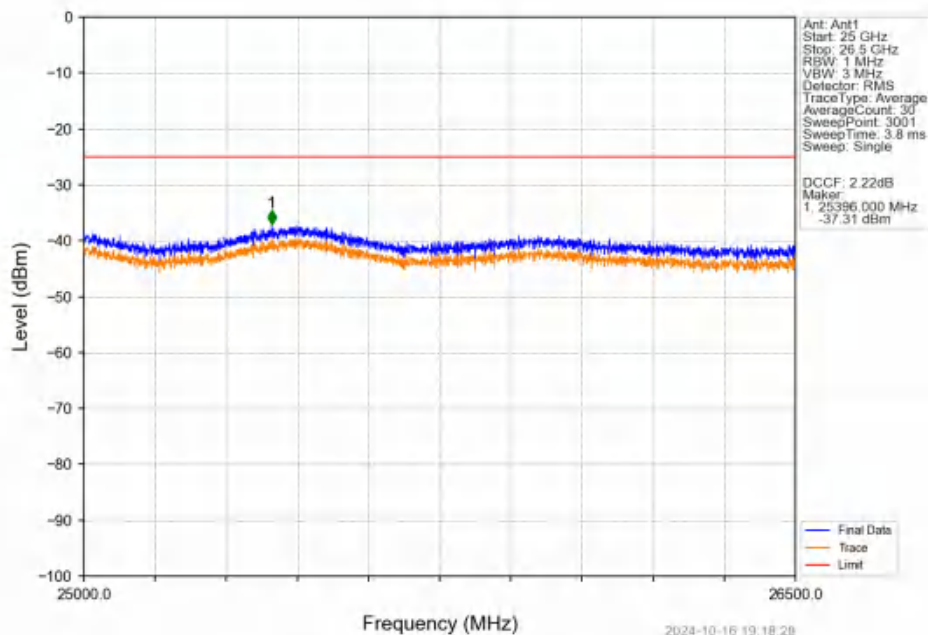
Band41 15MHz 16QAM LCH 2503.5MHz RB 75 0 NTN
