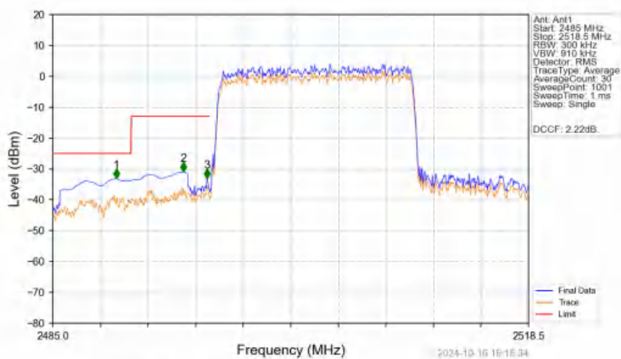
Band41 15MHz 16QAM LCH 2503.5MHz RB 75 0 NTN
