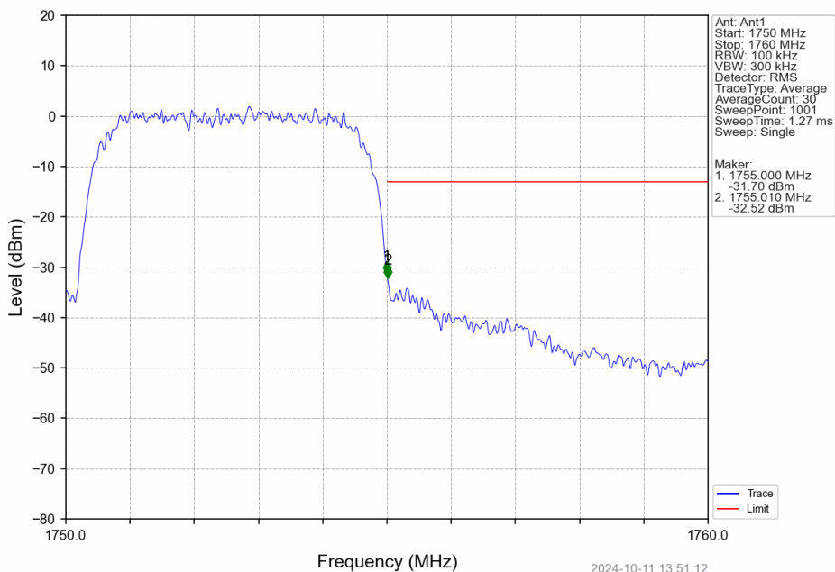
Band4 HSUPA HCH 1752.6MHz Subtest 1 NTN
