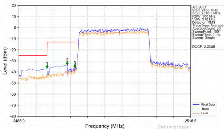
Band41_15MHz_16QAM_LCH_2503.5MHz_RB_75_0_NTNV
