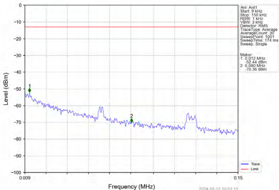
Band25 20MHz 16QAM LCH 1860MHz RB 1 0 NTV
