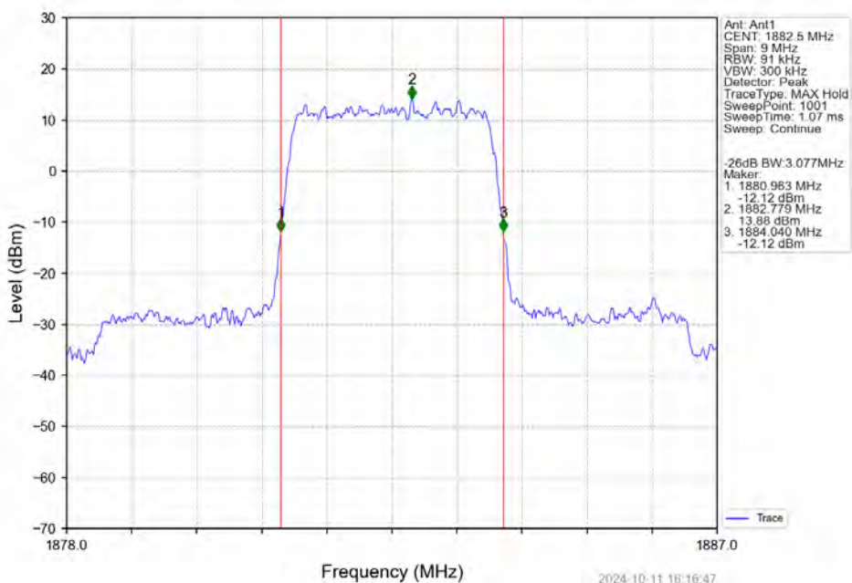
Band25_3MHz_QPSK_MCH_1882.5MHz_RB_15_0_NTNV
