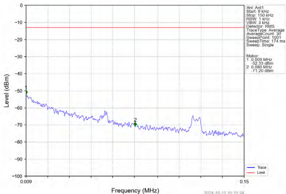
Band25_3MHz_QPSK_HCH_1913.5MHz_RB_1_0_NTV
