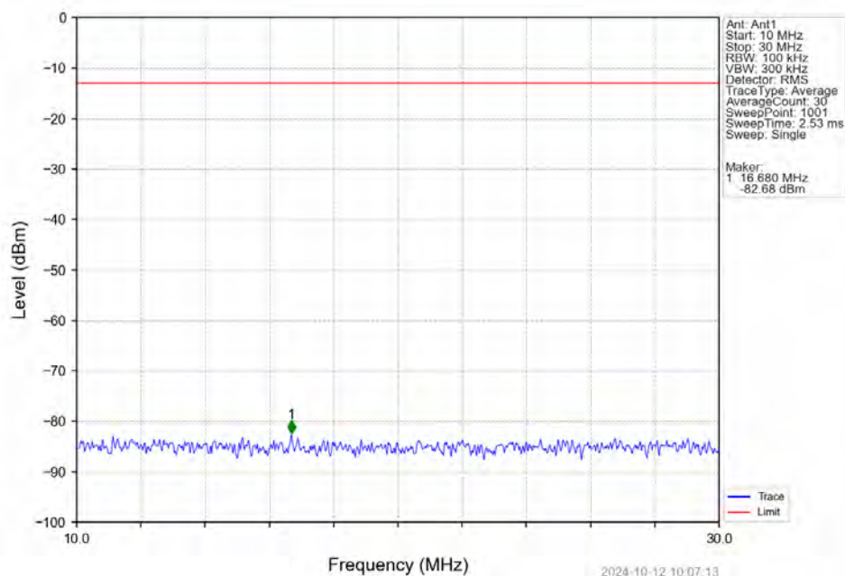
Band25_3MHz_QPSK_LCH_1851.5MHz_RB_1_0 NTN
