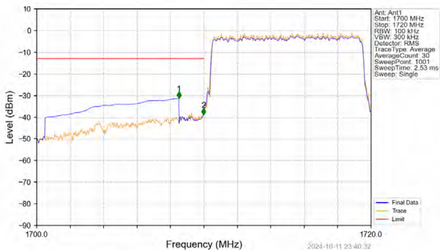
Band4_10MHz_16QAM_LCH_1715MHz_RB_50_0_NTN
