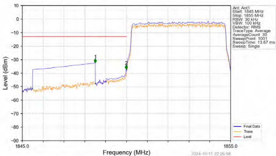
Band2_5MHz_16QAM_LCH_1852.5MHz_RB_25_0_NTV
