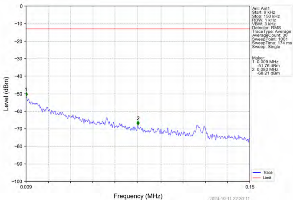
Band2_5MHz_16QAM_HCH_1907.5MHz_RB_1_0_NTN
