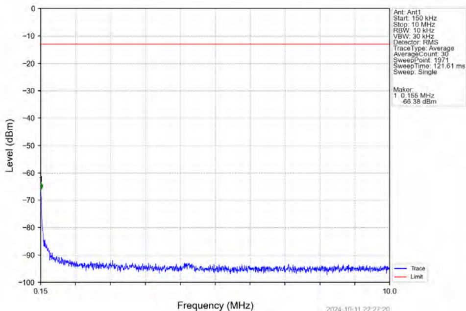
Band2_5MHz_QPSK_MCH_1880MHz_RB_1_0_NTN
