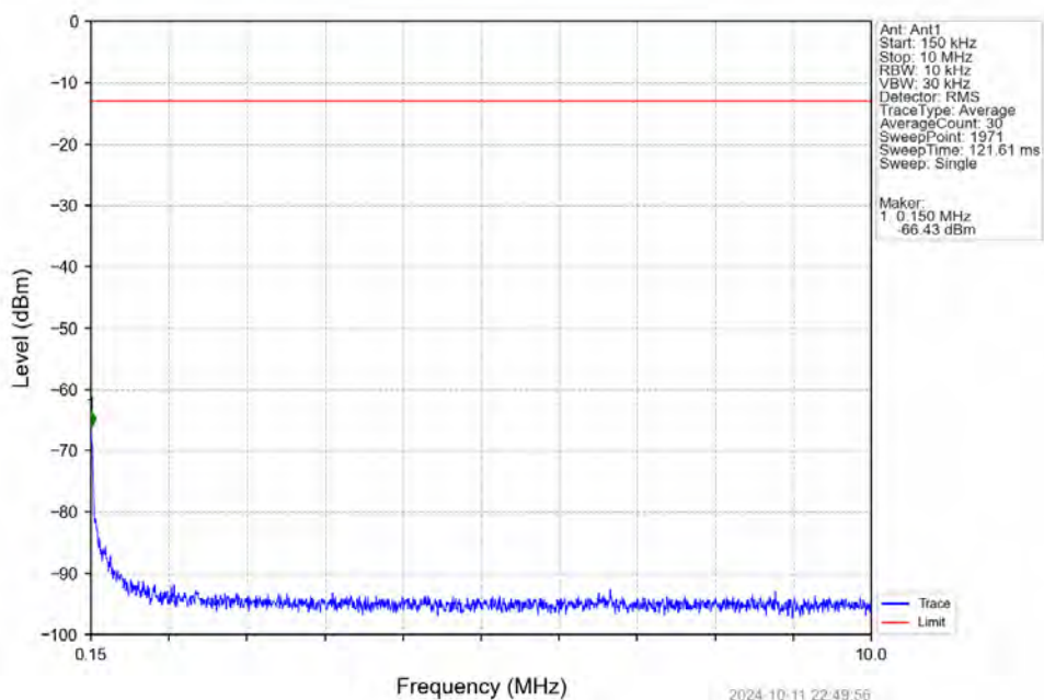
Band2_15MHz_16QAM_MCH_1880MHz_RB_1_0_NTNV
