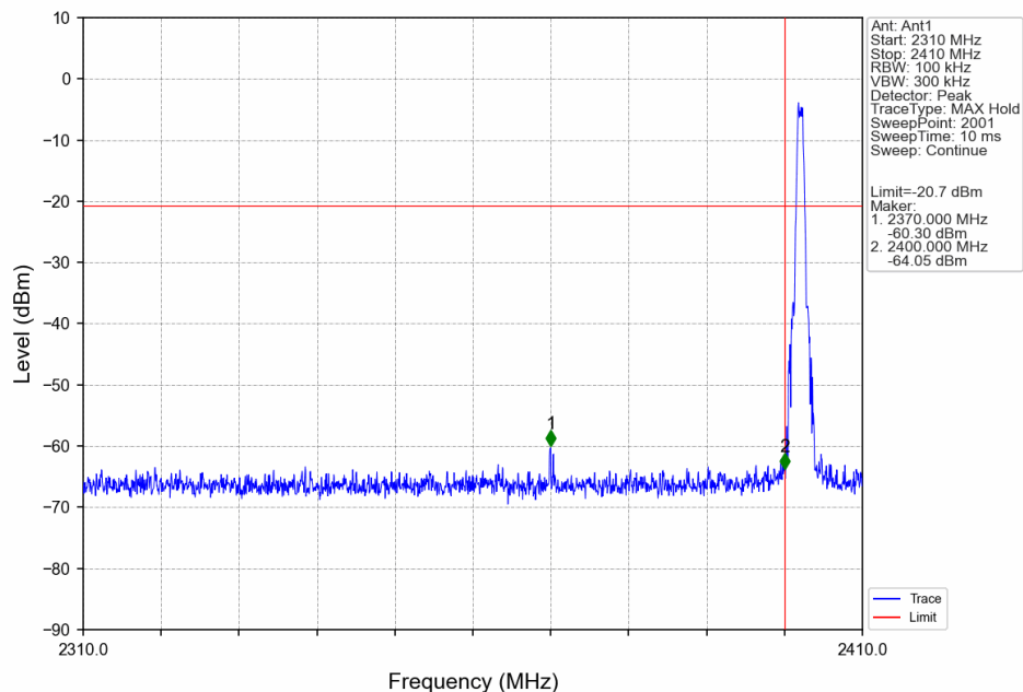
1M_LCH_2402MHz_Ant1_NTNV
