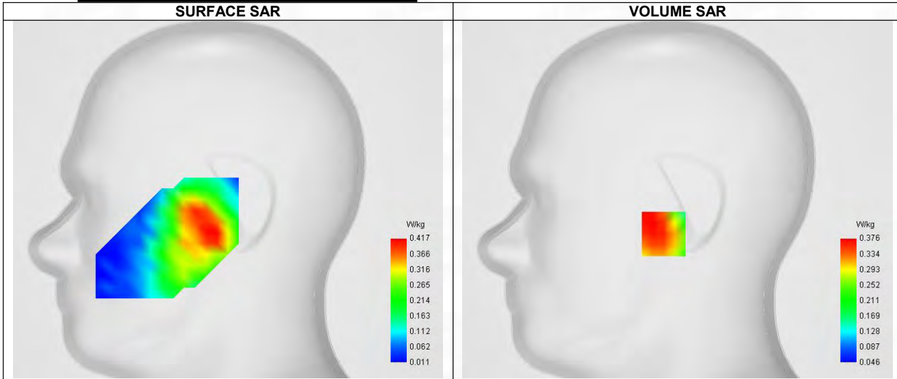
Maximum location: X=-10.00, Y=-25.00 ; SAR Peak: 0.55 W/kg
