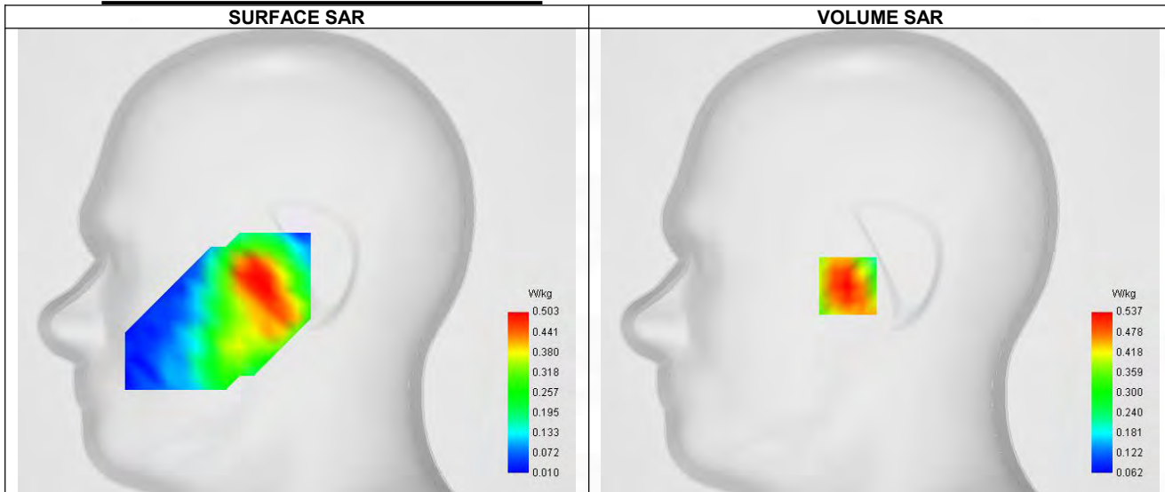
Maximum location: X=-18.00, Y=-14.00 ; SAR Peak: 0.71 W/kg
