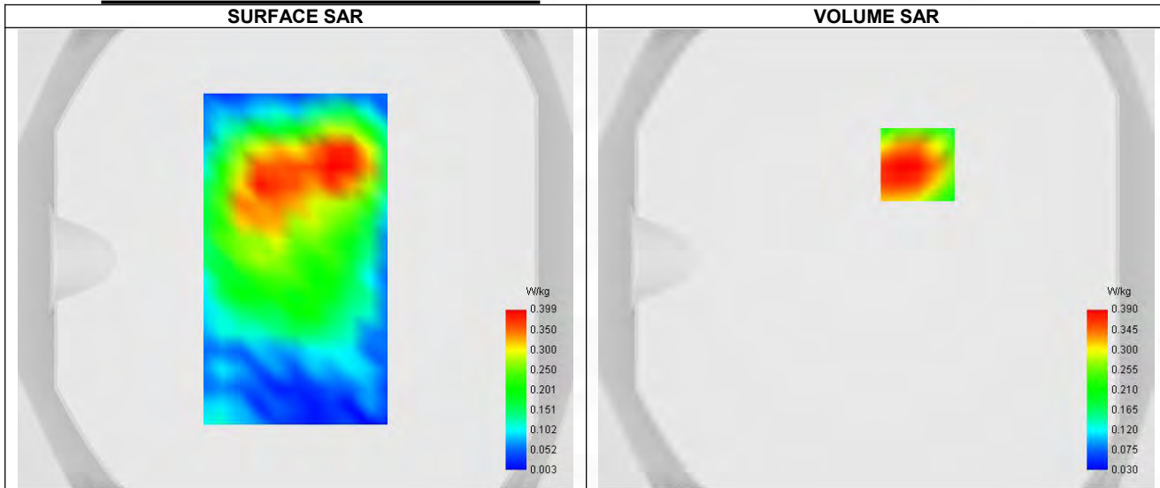
Maximum location: X=18.00, Y=41.00 ; SAR Peak: 0.57 W/kg
