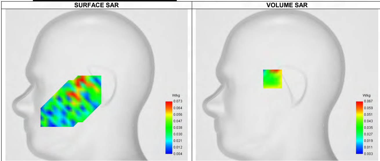
Maximum location: X=-25.00, Y=10.00 ; SAR Peak: 0.07 W/kg
