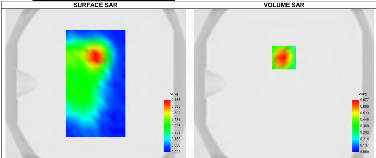
Maximum location: X=0.00, Y=35.00 ; SAR Peak: 1.06 W/kg
