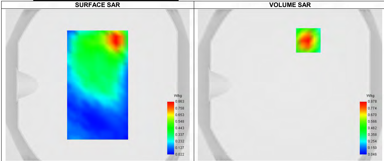
Maximum location: X=24.00, Y=59.00 ; SAR Peak: 1.37 W/kg
