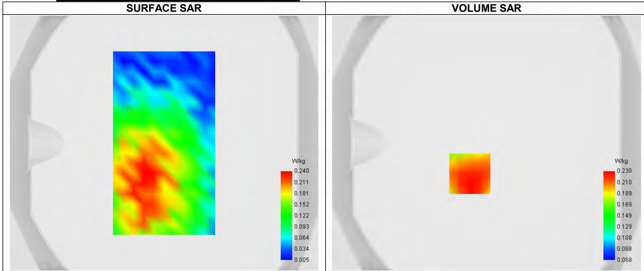
Maximum location: X=-13.00, Y=-24.00 ; SAR Peak: 0.29 W/kg
