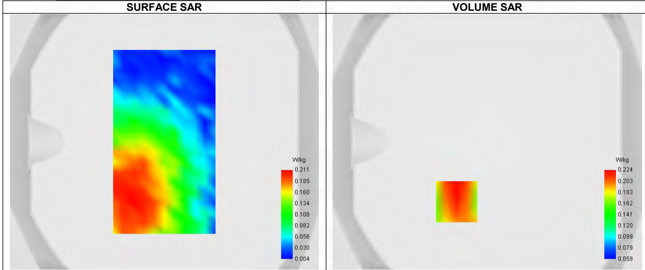
Maximum location: X=-24.00, Y=-47.00 ; SAR Peak: 0.32 W/kg
