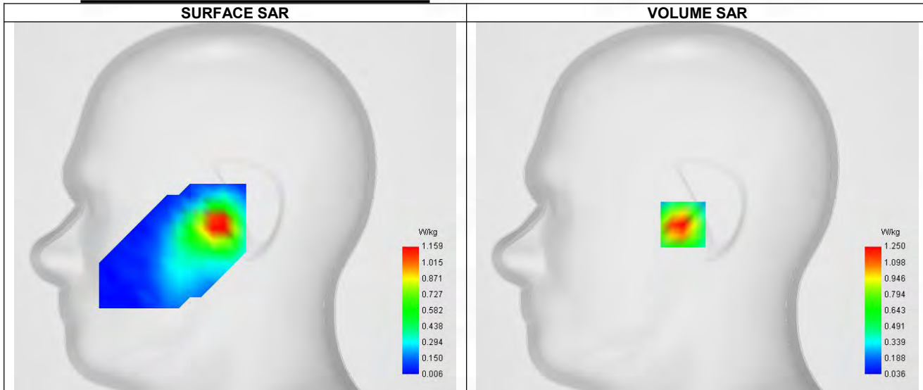
Maximum location: X=-10.00, Y=-13.00 ; SAR Peak: 1.93 W/kg
