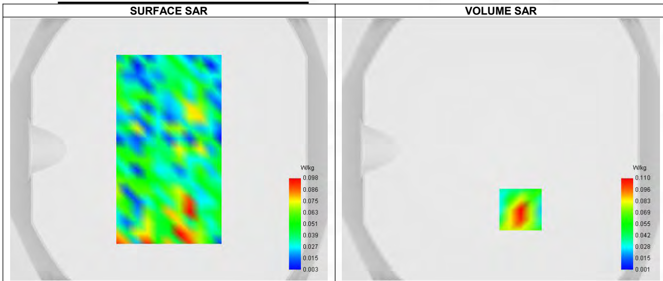
Maximum location: X=15.00, Y=-46.00 ; SAR Peak: 0.17 W/kg
