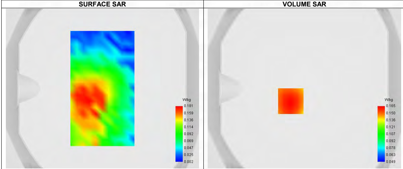
Maximum location: X=-17.00, Y=-16.00 ; SAR Peak: 0.20 W/kg
