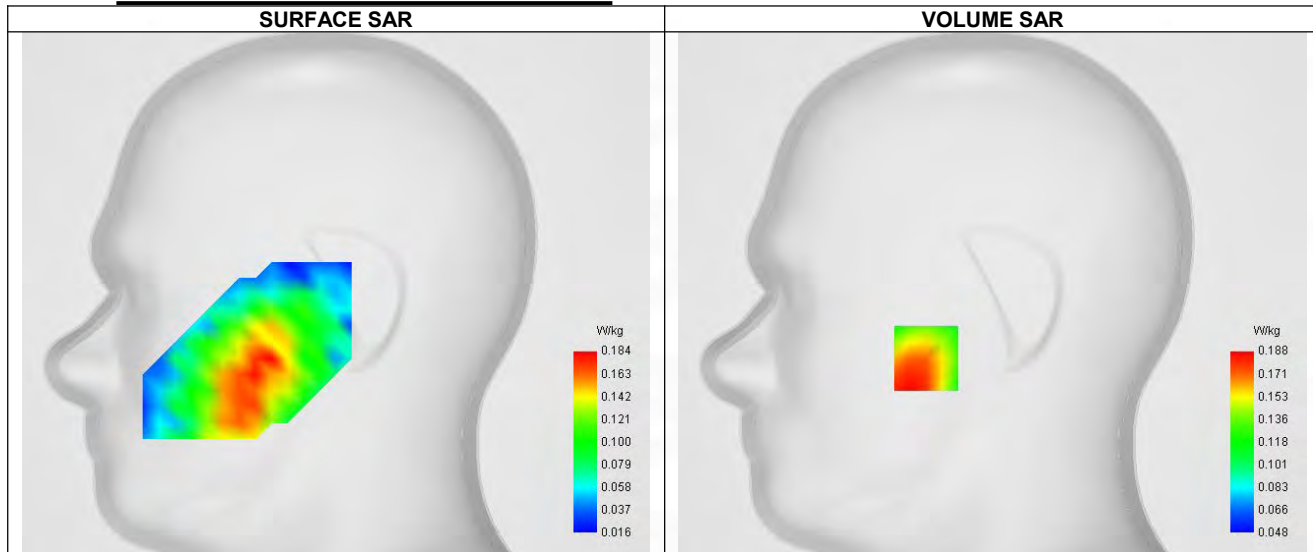
Maximum location: X=-33.00, Y=-32.00 ; SAR Peak: 0.24 W/kg
