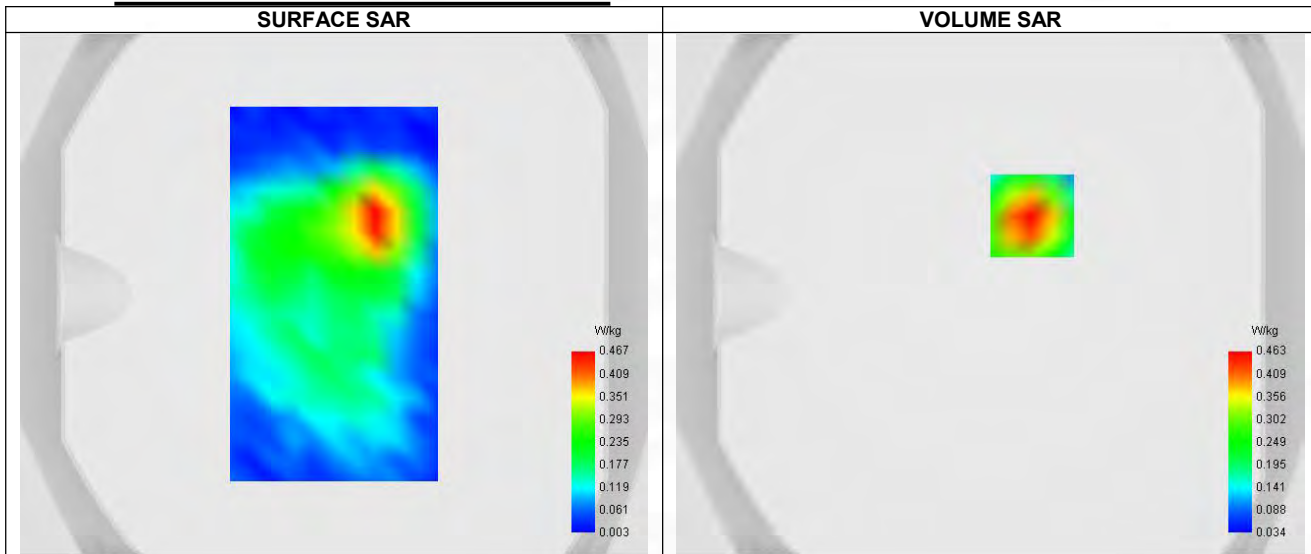
Maximum location: X=16.00, Y=30.00 ; SAR Peak: 0.69 W/kg
