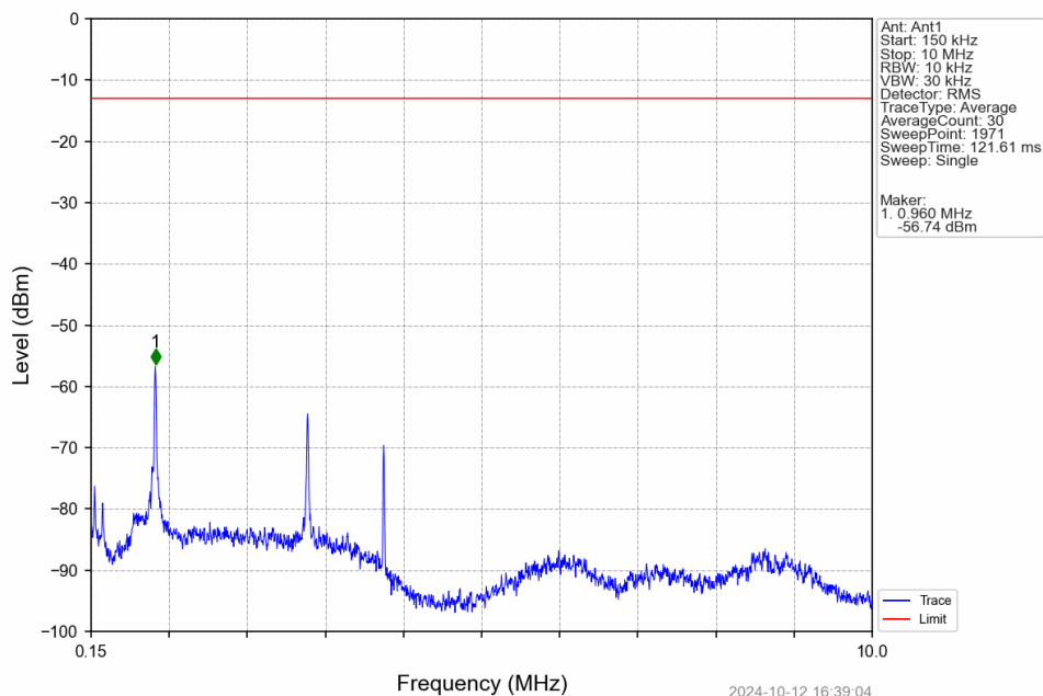
Band4_HSDPA_LCH_1712.4MHz_Subtest 1 NTN
