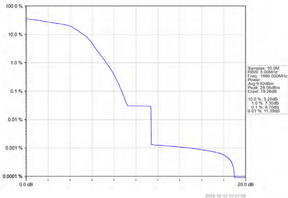
PCS1900 EGPRS MCH 1880MHz 4 TX Slots NTN
