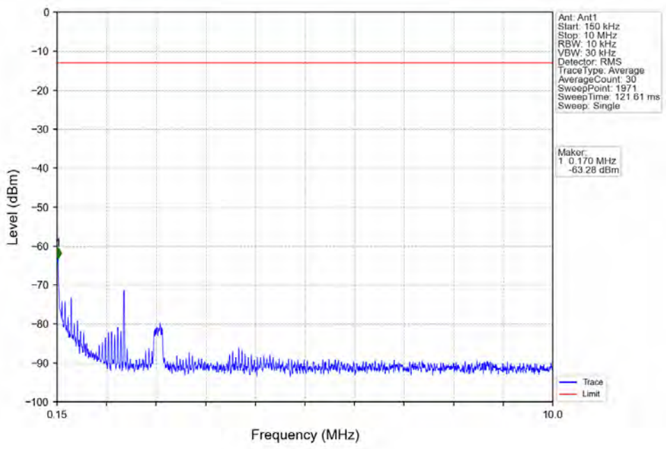
Band66_5MHz_16QAM_MCH_1745MHz_RB_1_0_NTNV
