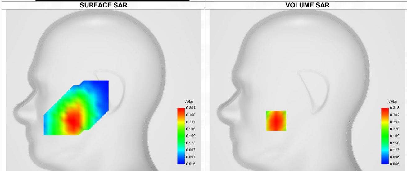
Maximum location: X=-50.00, Y=-49.00 ; SAR Peak: 0.38 W/kg
