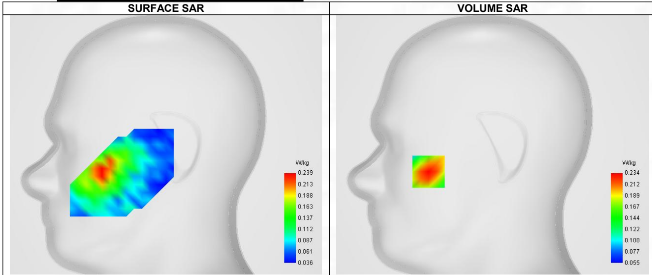
Maximum location: X=-64.00, Y=-27.00 ; SAR Peak: 0.32 W/kg
