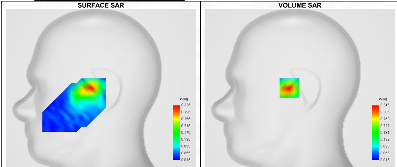
Maximum location: X=-17.00, Y=0.00 ; SAR Peak: 0.55 W/kg
