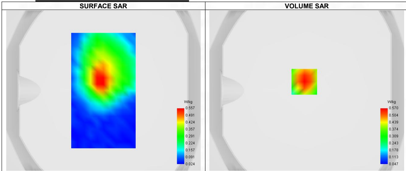
Maximum location: X=-3.00, Y=11.00 ; SAR Peak: 0.80 W/kg
