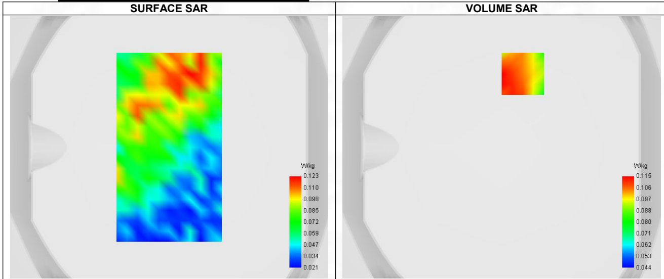
Maximum location: X=16.00, Y=56.00 ; SAR Peak: 0.17 W/kg
