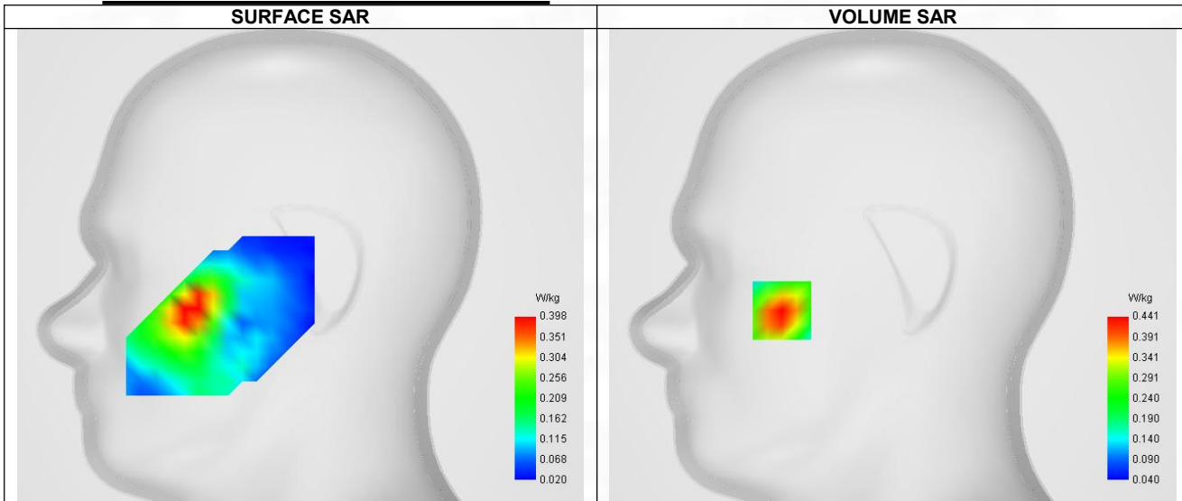
Maximum location: X=-61.00, Y=-25.00 ; SAR Peak: 0.64 W/kg
