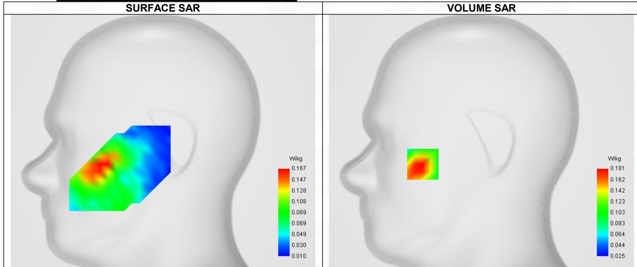
Maximum location: X=-60.00, Y=-24.00 ; SAR Peak: 0.27 W/kg
