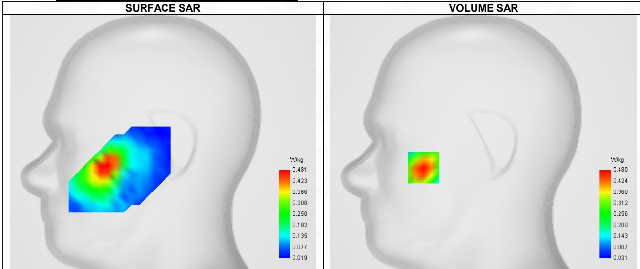
Maximum location: X=-61.00, Y=-26.00 ; SAR Peak: 0.74 W/kg
