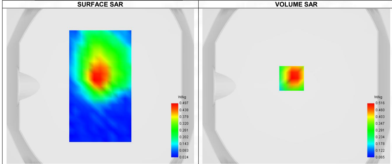
Maximum location: X=-6.00, Y=10.00 ; SAR Peak: 0.74 W/kg
