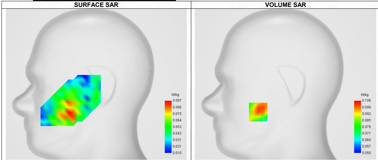
Maximum location: X=-47.00, Y=-48.00 ; SAR Peak: 0.13 W/kg
