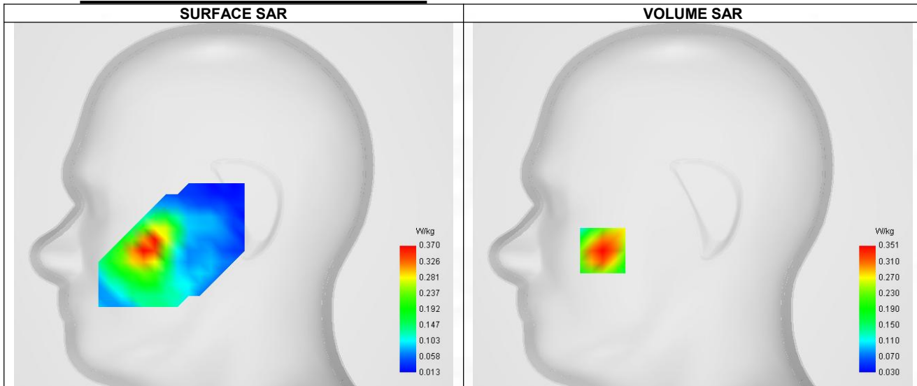
Maximum location: X=-64.00, Y=-32.00 ; SAR Peak: 0.45 W/kg
