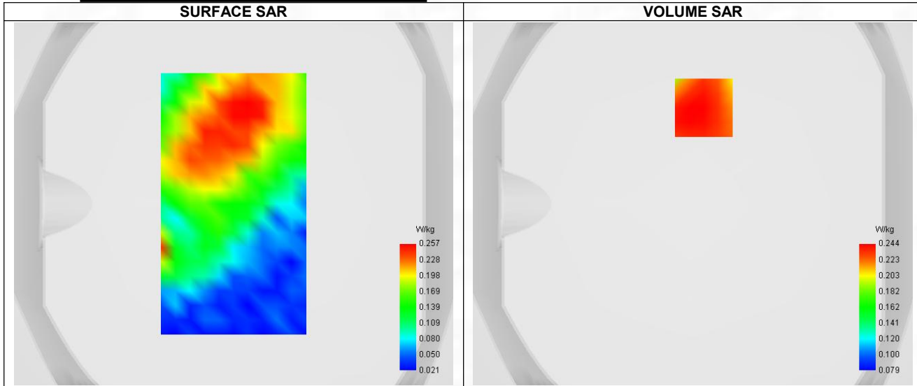
Maximum location: X=6.00, Y=53.00 ; SAR Peak: 0.32 W/kg
