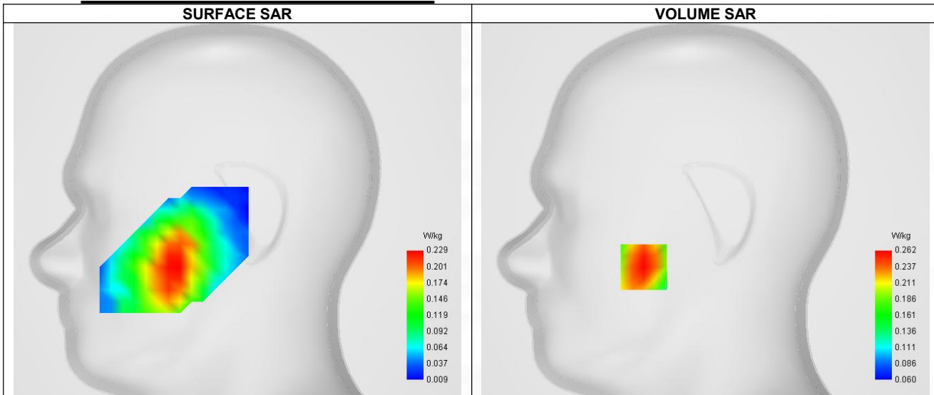
Maximum location: X=-43.00, Y=-40.00 ; SAR Peak: 0.32 W/kg
