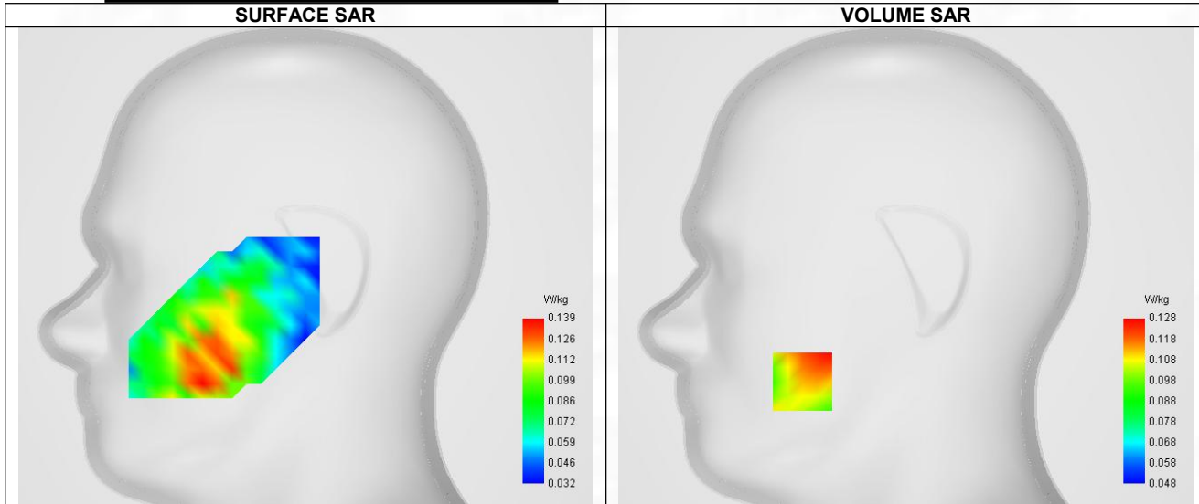
Maximum location: X=-56.00, Y=-63.00 ; SAR Peak: 0.16 W/kg
