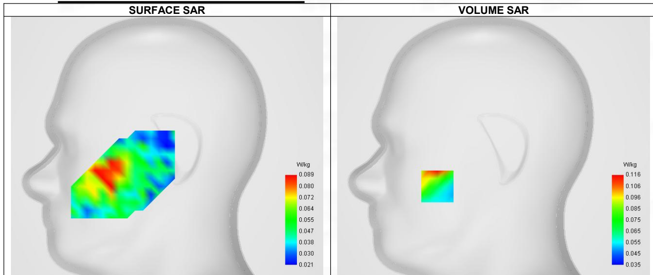
Maximum location: X=-56.00, Y=-40.00 ; SAR Peak: 0.17 W/kg
