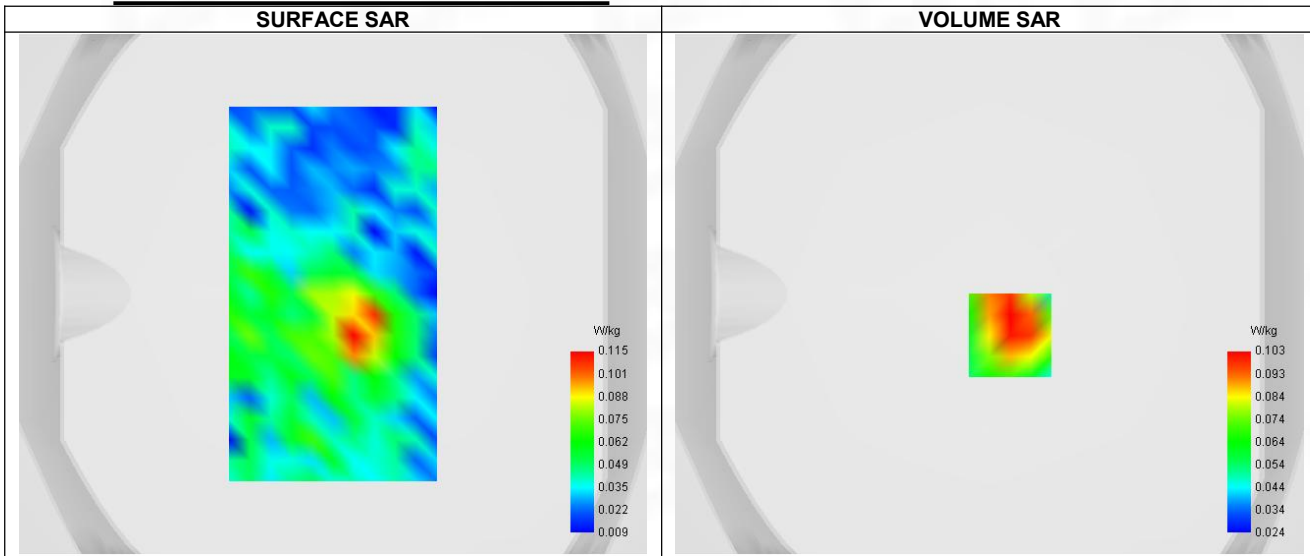
Maximum location: X=8.00, Y=-16.00 ; SAR Peak: 0.17 W/kg
