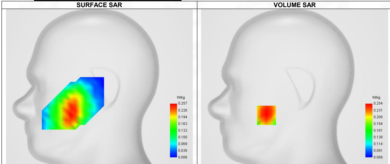
Maximum location: X=-47.00, Y=-48.00 ; SAR Peak: 0.30 W/kg
