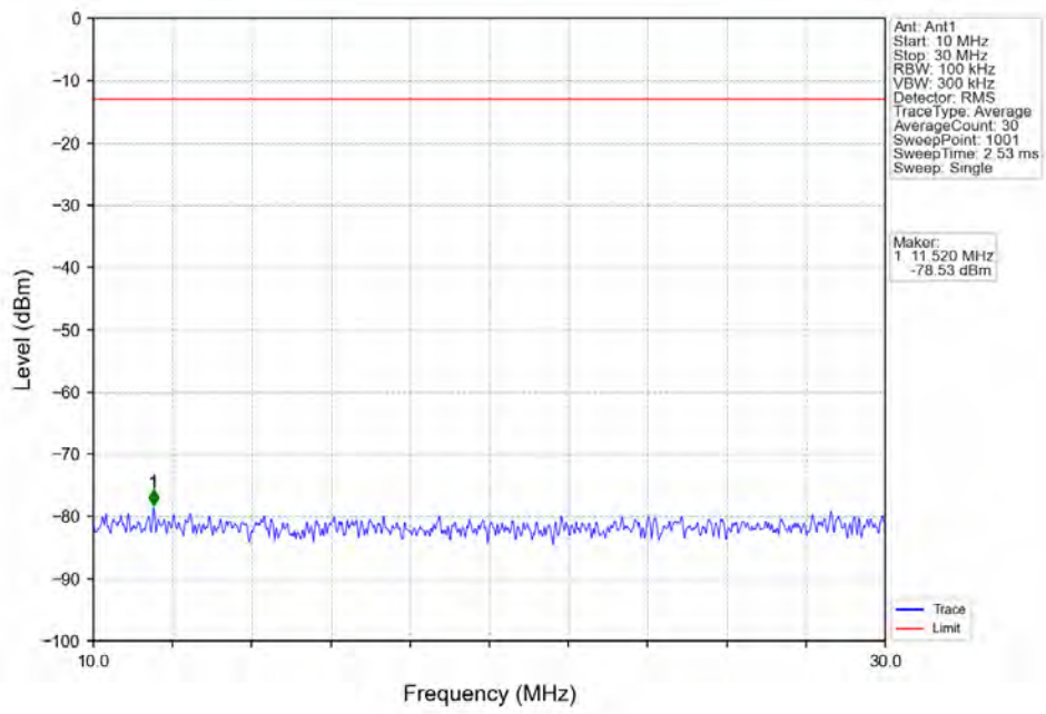
Band2_15MHz_16QAM_MCH_1880MHz_RB_1_0_NTNV
