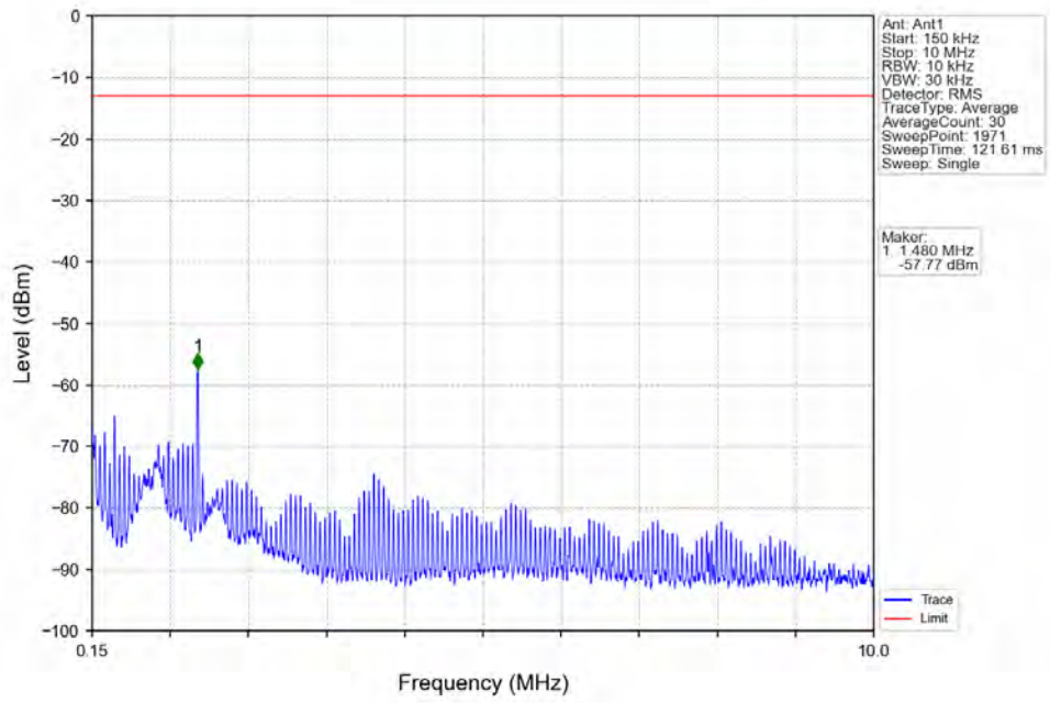
Band2_3MHz_16QAM_HCH_1908.5MHz_RB_1_0_NTNV
