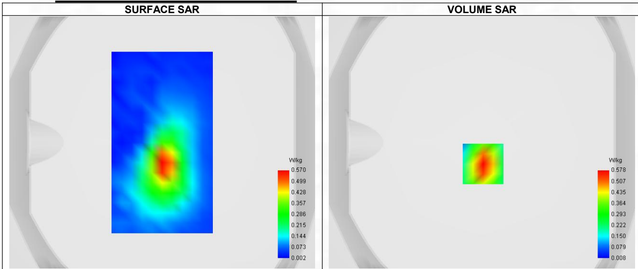
Maximum location: X=1.00, Y=-17.00 ; SAR Peak: 0.88 W/kg
