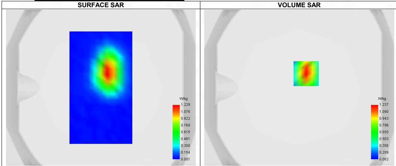
Maximum location: X=9.00, Y=18.00 ; SAR Peak: 1.86 W/kg
