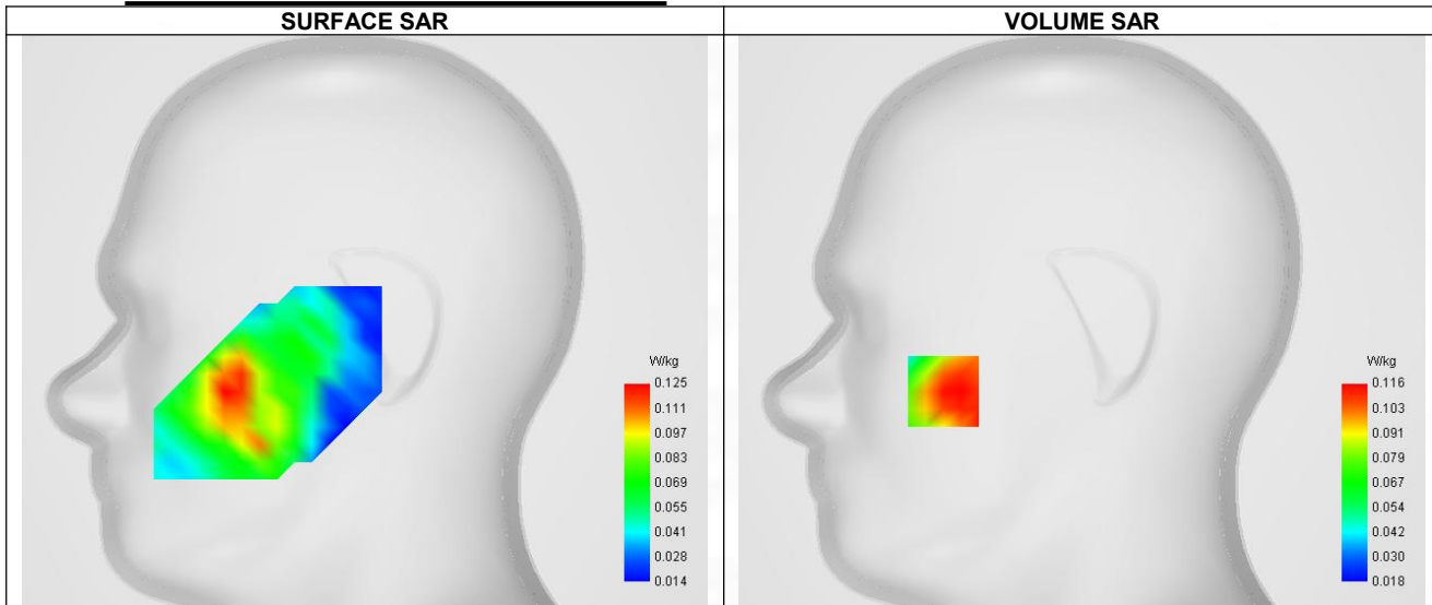
Maximum location: X=-63.00, Y=-32.00 ; SAR Peak: 0.15 W/kg
