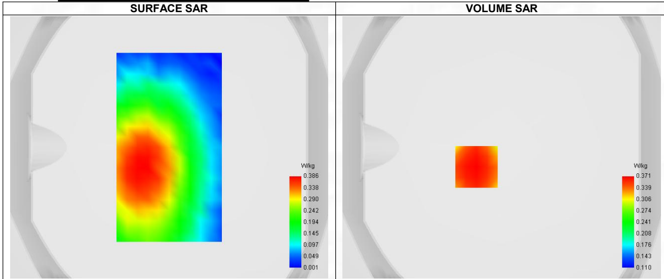
Maximum location: X=-19.00, Y=-15.00 ; SAR Peak: 0.45 W/kg
