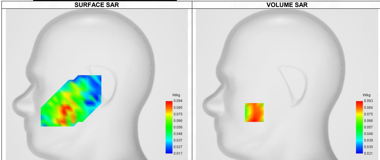
Maximum location: X=-56.00, Y=-48.00 ; SAR Peak: 0.13 W/kg
