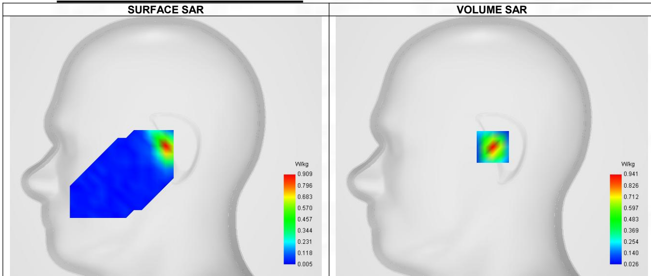
Maximum location: X=1.00, Y=-1.00 ; SAR Peak: 1.68 W/kg
