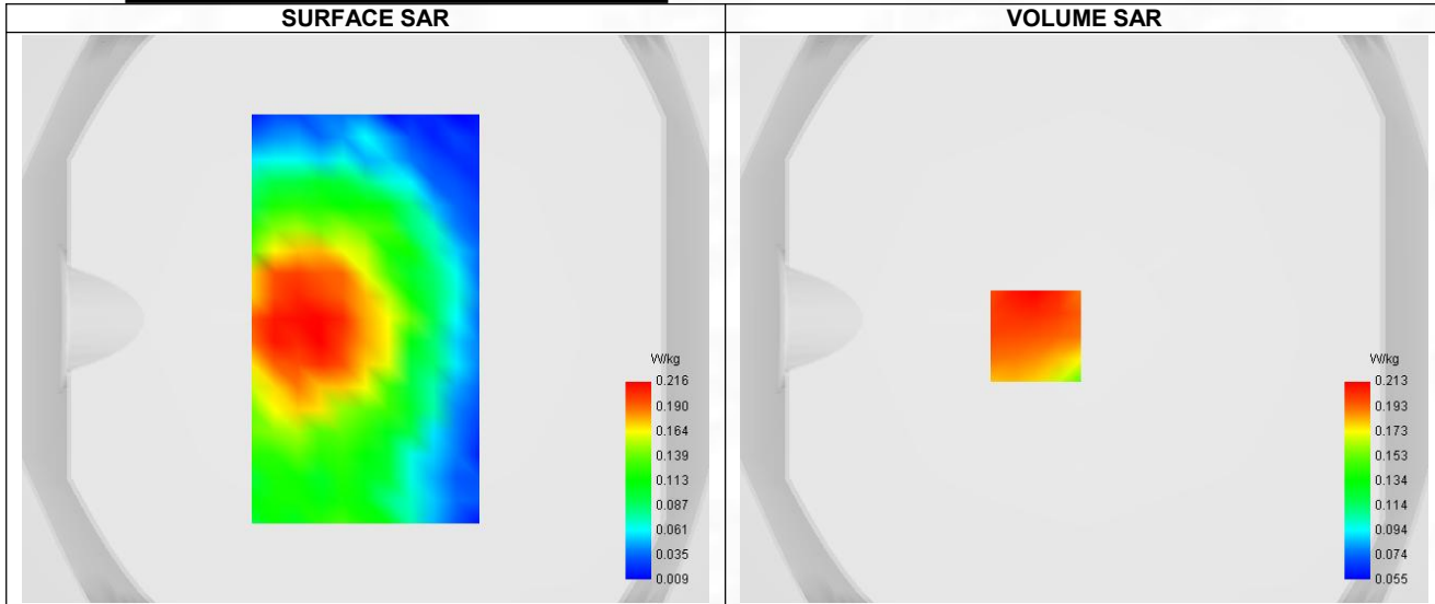
Maximum location: X=-17.00, Y=-6.00 ; SAR Peak: 0.25 W/kg
