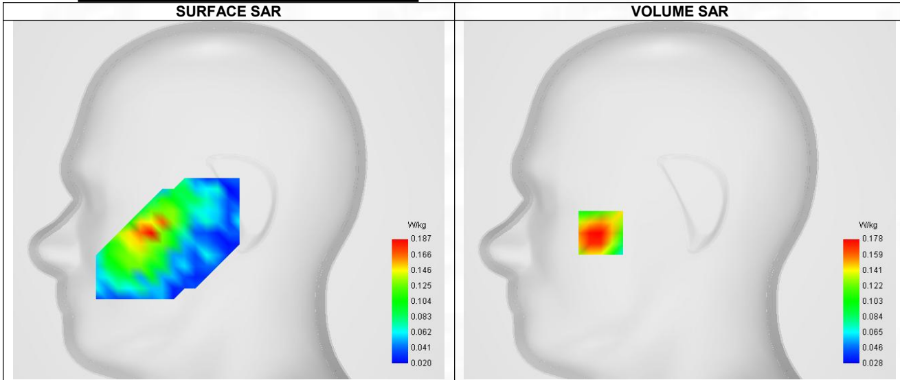
Maximum location: X=-57.00, Y=-24.00 ; SAR Peak: 0.20 W/kg
