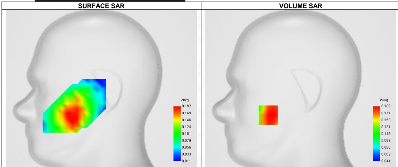
Maximum location: X=-53.00, Y=-43.00 ; SAR Peak: 0.25 W/kg
