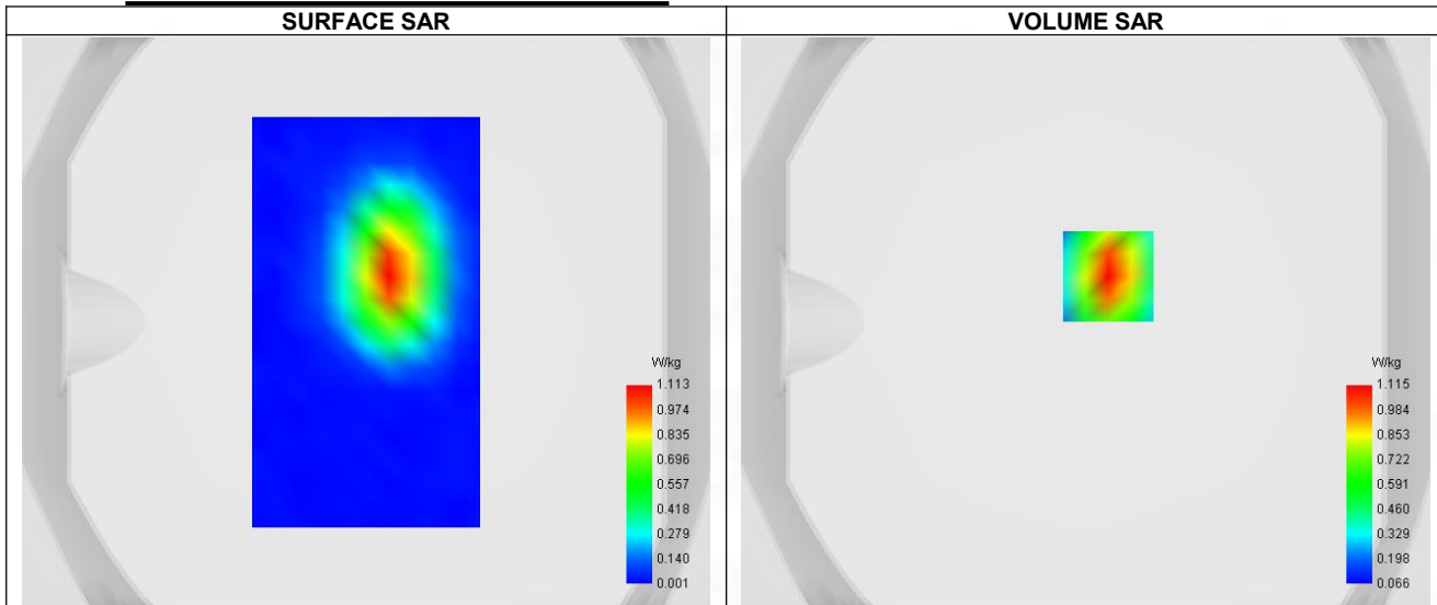
Maximum location: X=8.00, Y=16.00 ; SAR Peak: 1.68 W/kg
