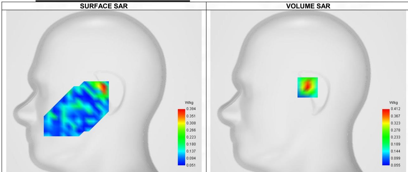
Maximum location: X=-1.00, Y=6.00 ; SAR Peak: 0.88 W/kg
