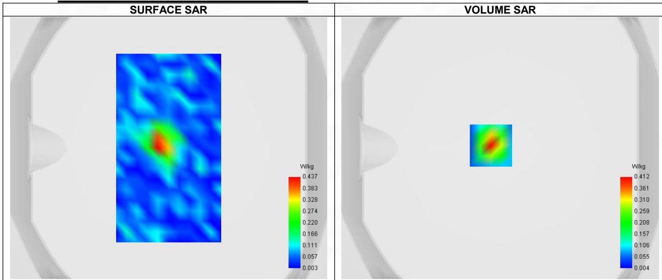
Maximum location: X=-7.00, Y=2.00 ; SAR Peak: 0.74 W/kg
