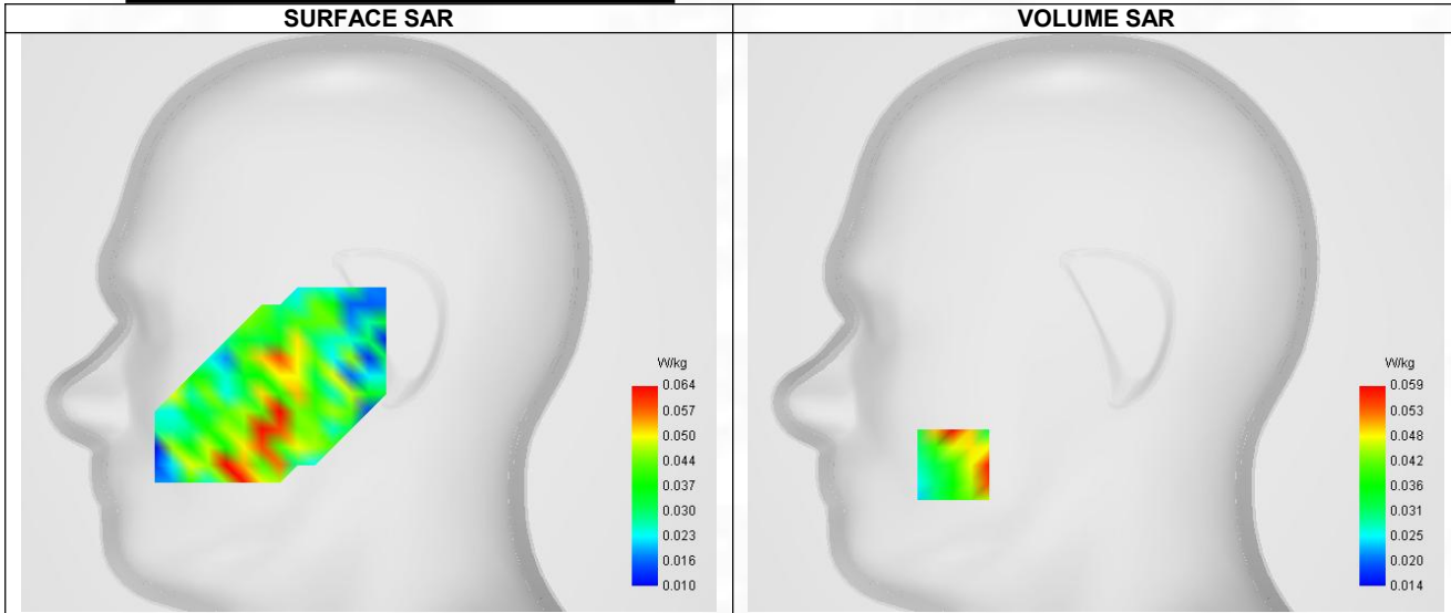
Maximum location: X=-64.00, Y=-64.00 ; SAR Peak: 0.09 W/kg
