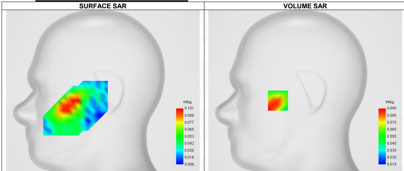
Maximum location: X=-44.00, Y=-16.00 ; SAR Peak: 0.13 W/kg
