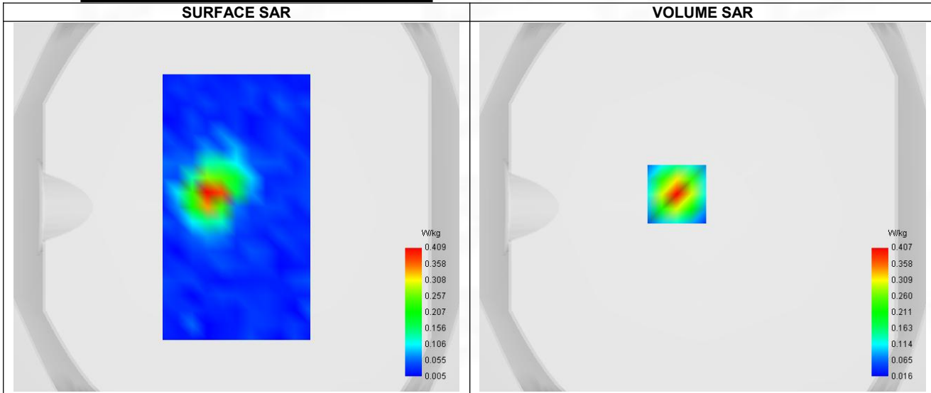
Maximum location: X=-14.00, Y=7.00 ; SAR Peak: 0.64 W/kg
