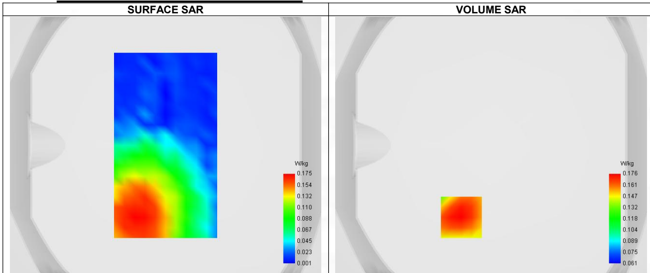
Maximum location: X=-23.00, Y=-56.00 ; SAR Peak: 0.20 W/kg
