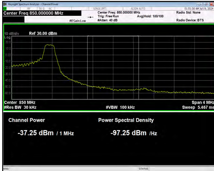
Band26(824-849) 16QAM BW=1.4MHz Channel=27033 RB Size=1 Position=#Max Extended
