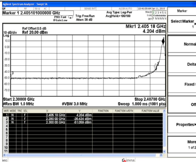
2405 MHz – Peak
