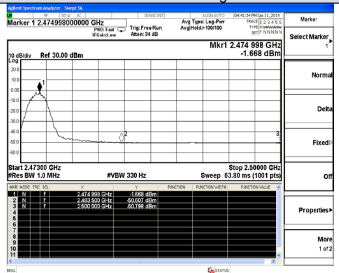
2475 MHz – Average
