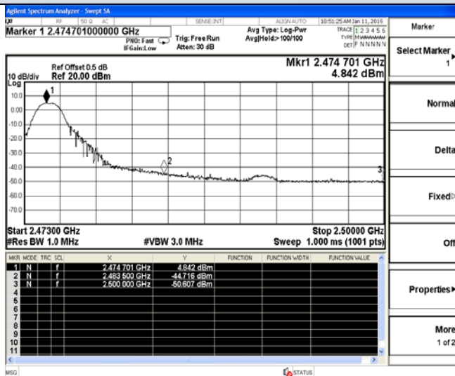
2475 MHz – Peak
