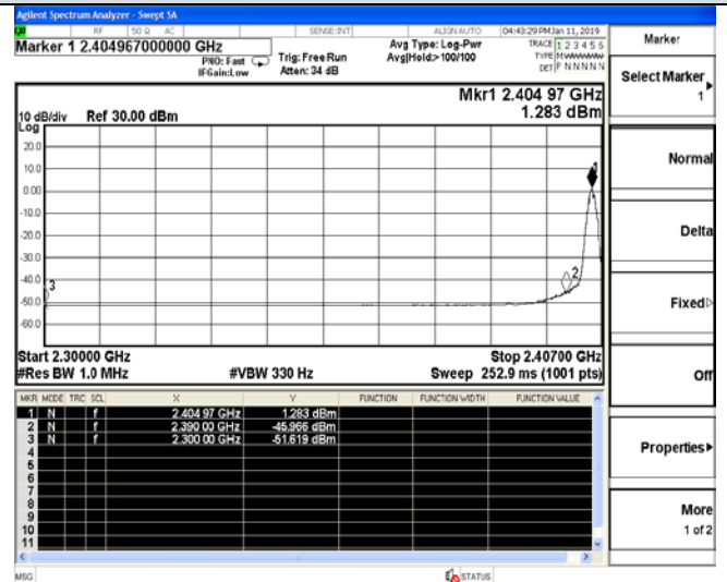
2405 MHz – Average
