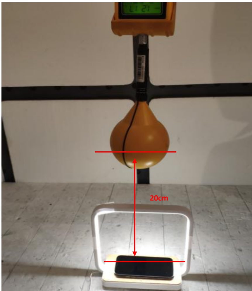
TestPosition E-Exposure photo from top surface (20cm) (TM1)
