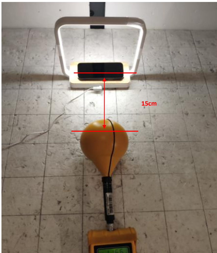
TestPosition A-Exposure photo from side edge surface-Rear (TM1)
