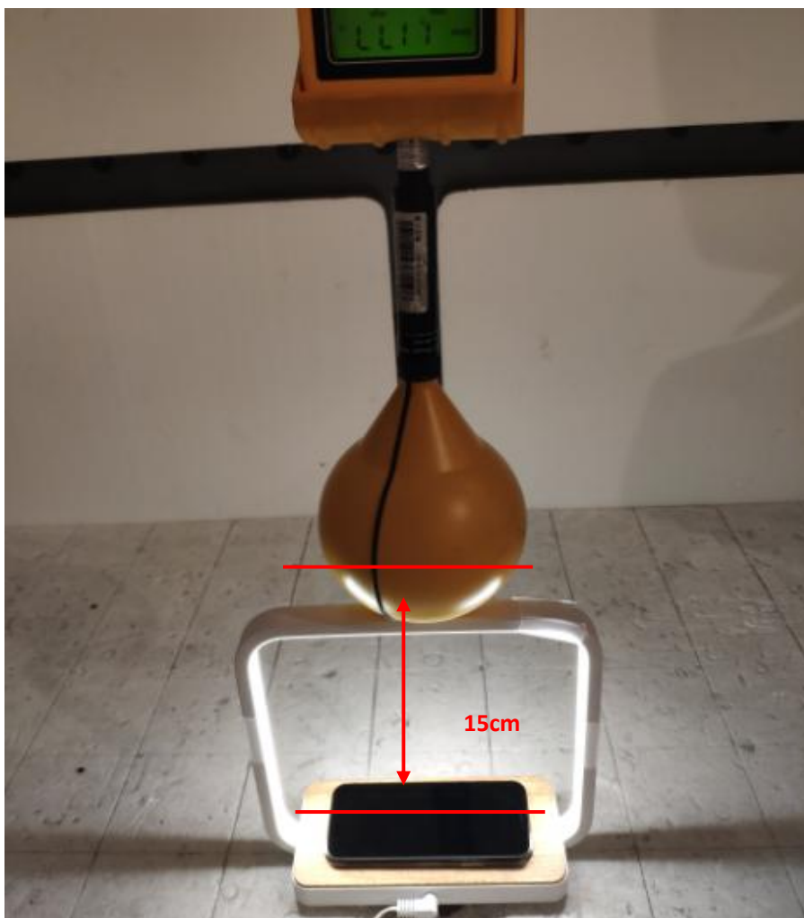
TestPosition E-Exposure photo from top surface (15cm) (TM1)
