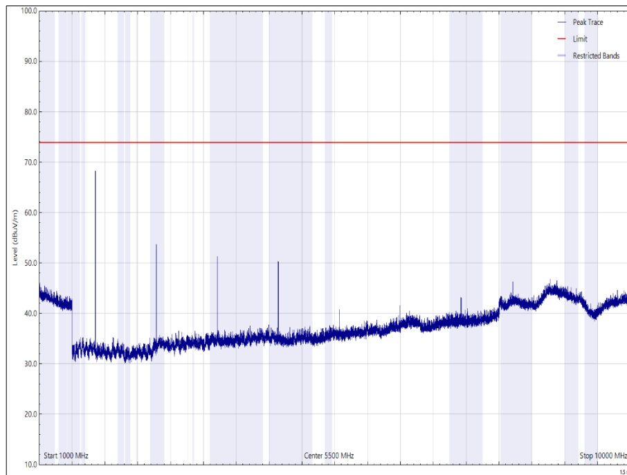
Figure 52 - 927.25 MHz - 1 GHz to 10 GHz, Vertical, N/A Orientation - Peak
