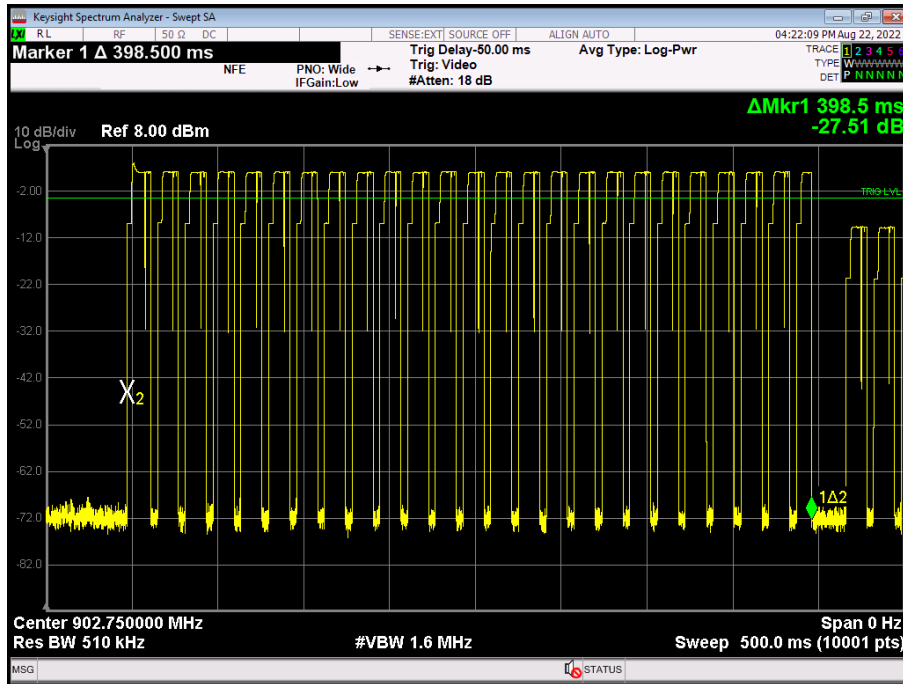
Figure 3 - Dwell Time
