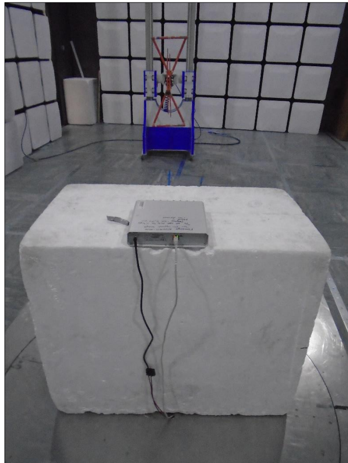
Figure 62 - Test Setup - 30 MHz to 1 GHz
