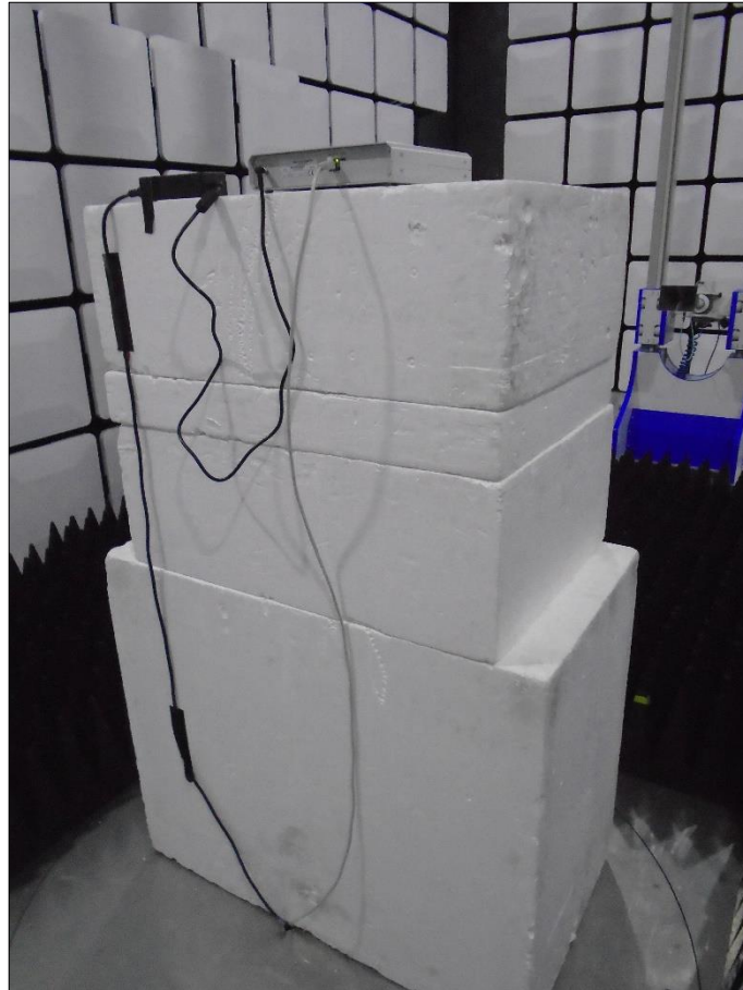
Figure 63 - Test Setup - 1 GHz to 10 GHz
