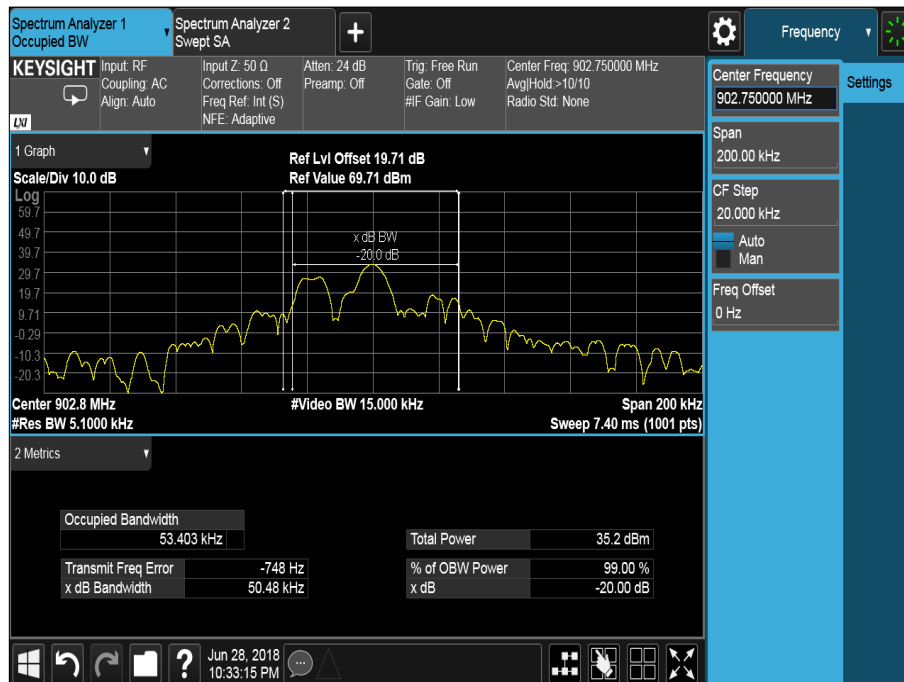
Figure 67 - 902.75 MHz
