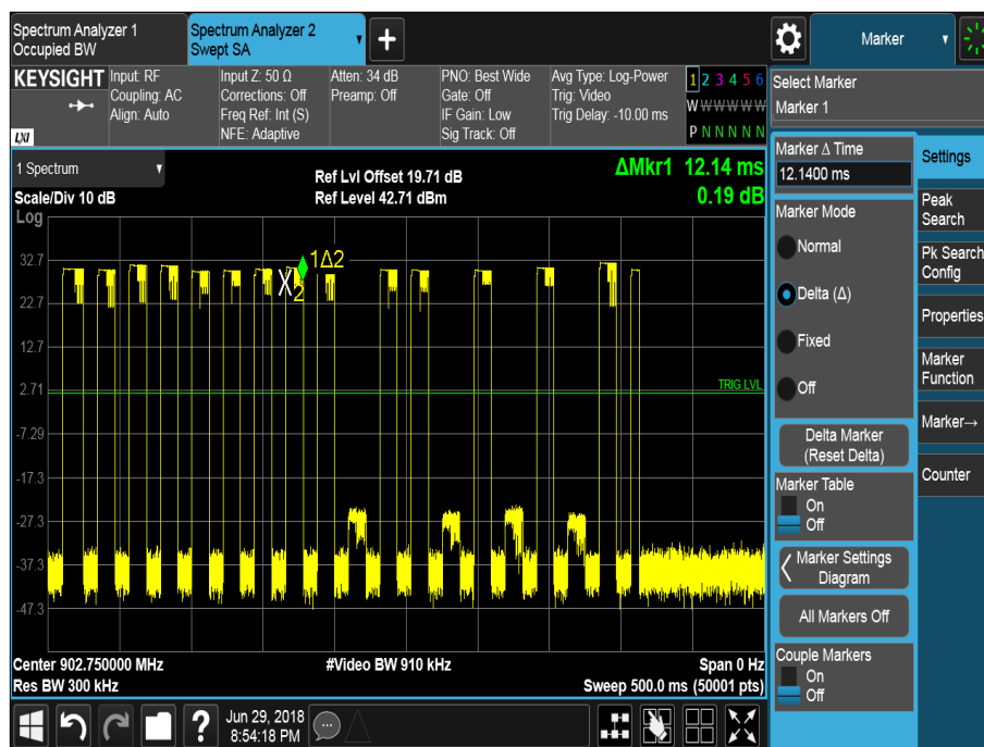
Figure 63 - Dwell Time
