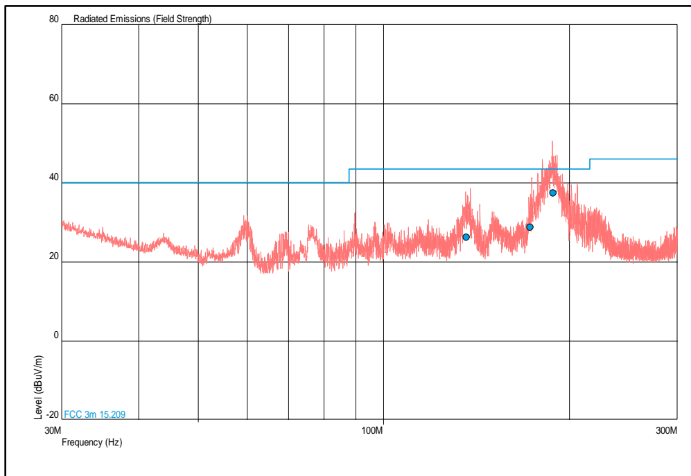
Figure 33 - 927.25 MHz - 30 MHz to 300 MHz Polarity: Combined, EUT Orientation: Y
