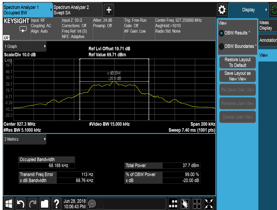
Figure 69 - 927.25 MHz
