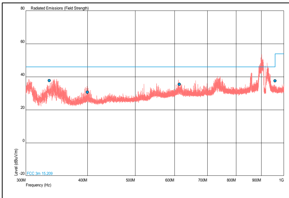
Figure 22 - 915.25 MHz - 300 MHz to 1 GHz Polarity: Combined, EUT Orientation: Y
