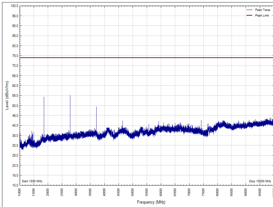
Figure 35 - 927.25 MHz - 1 GHz to 10 GHz Polarity: Vertical, EUT Orientation: X, Peak
