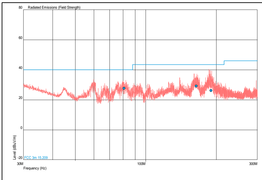
Figure 9 - 902.75 MHz - 30 MHz to 300 MHz Polarity: Combined, EUT Orientation: Y
