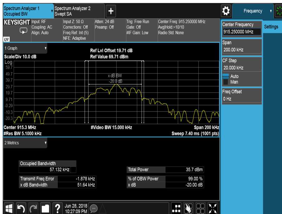
Figure 68 - 915.25 MHz
