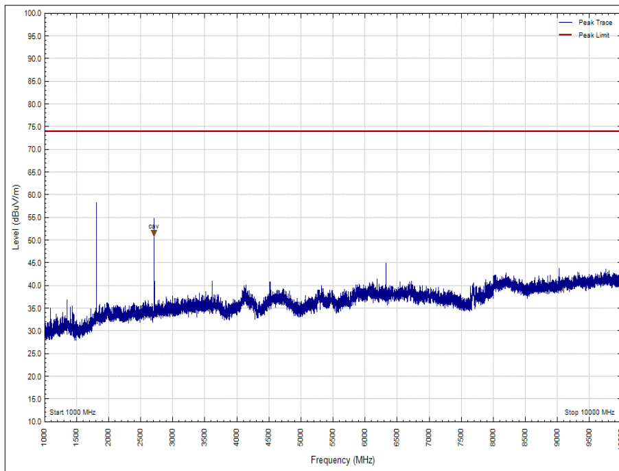
Figure 15 - 902.75 MHz - 1 GHz to 10 GHz Polarity: Vertical, EUT Orientation: Y, Peak
