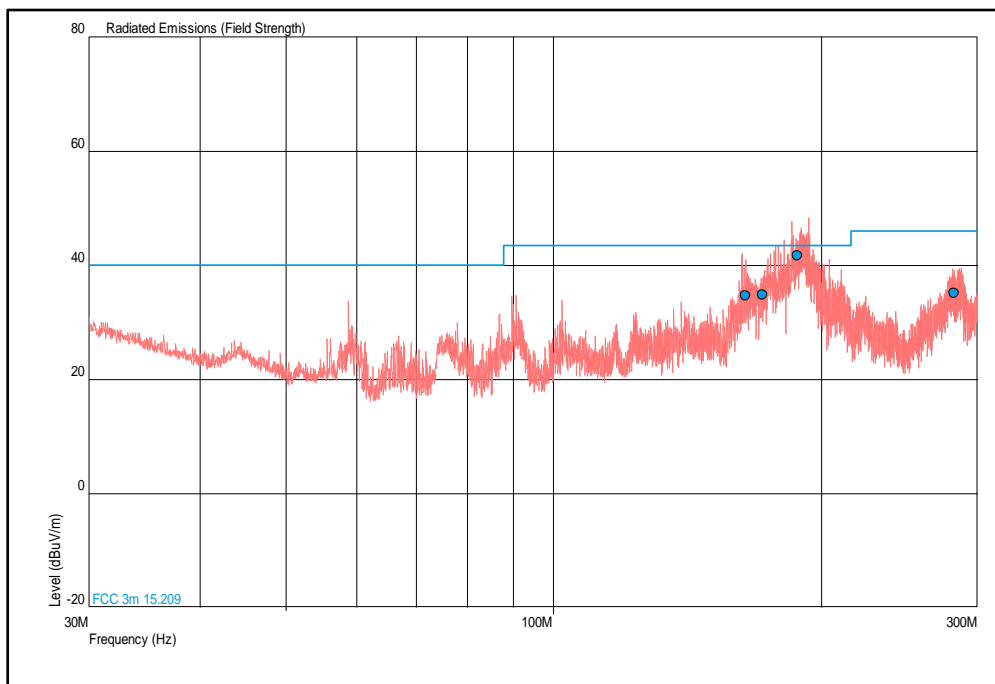
Figure 21 - 915.25 MHz - 30 MHz to 300 MHz Polarity: Combined, EUT Orientation: Y
