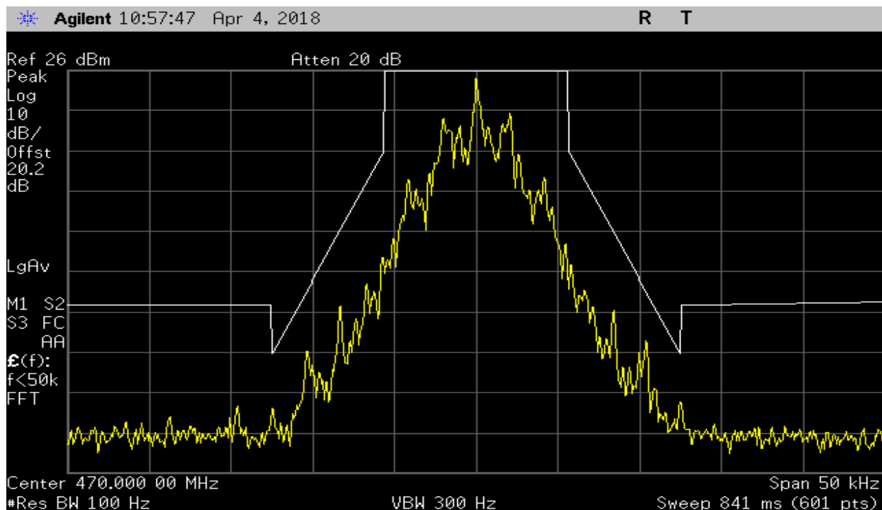
Plot 6 – Mid Chanel 12.5 kHz Spacing – Mask D
