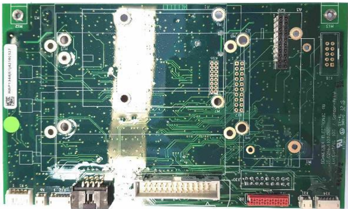
HAP1344 BOTTOM
