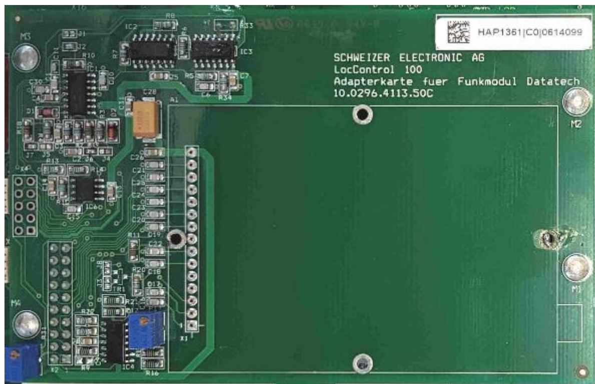
HAP1361 BOTTOM
