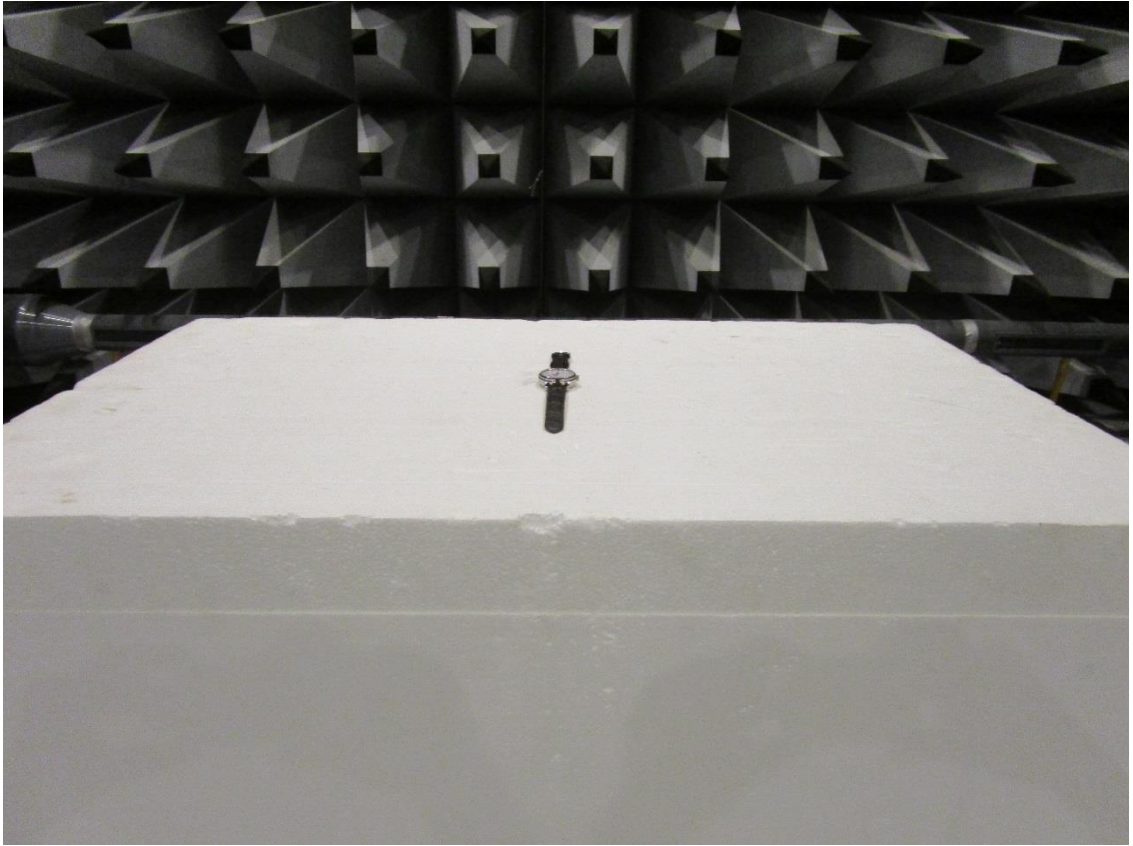
Photo Error! No text of specified style in document..6 measurement of radiated emission (above 1 GHz)
