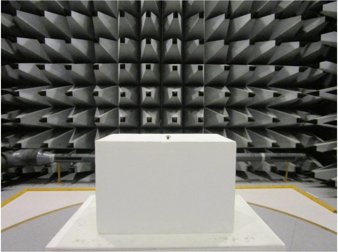
Photo Error! No text of specified style in document..5 Test setup regarding measurement of radiated emission (above 1 GHz)
