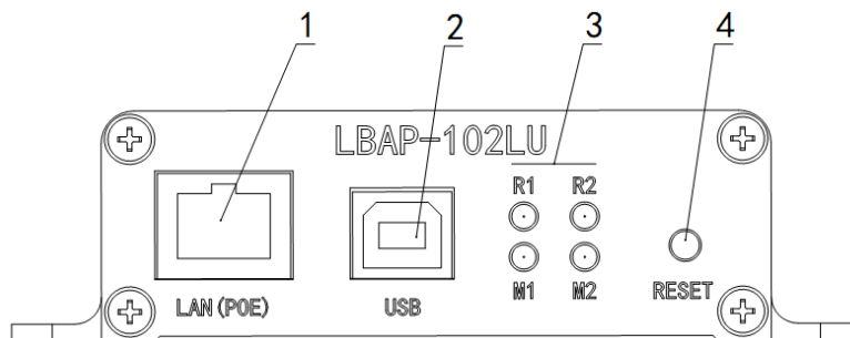
Piture 2 Panel Wiring Instructions
