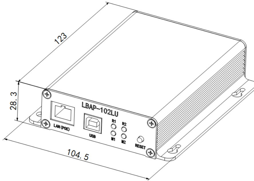
Picture 1 Appearance structure of wireless communication device
