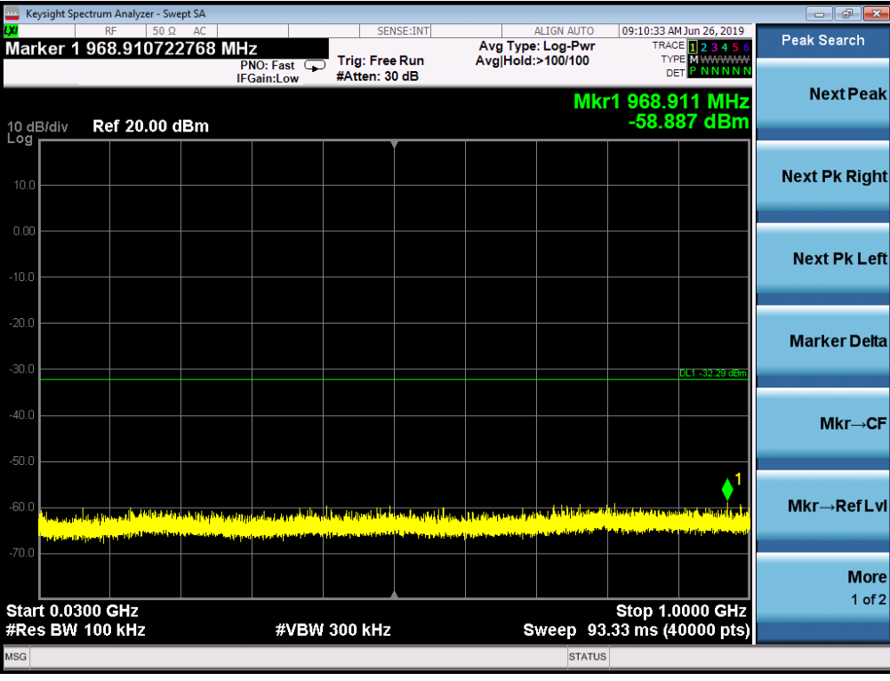
TEST PLOT OF OUT OF BAND EMISSIONS WITH THE WORST CASE OF (802.11n40 with data rate 13.5) FOR MODULATION IN LOW CHANNEL
