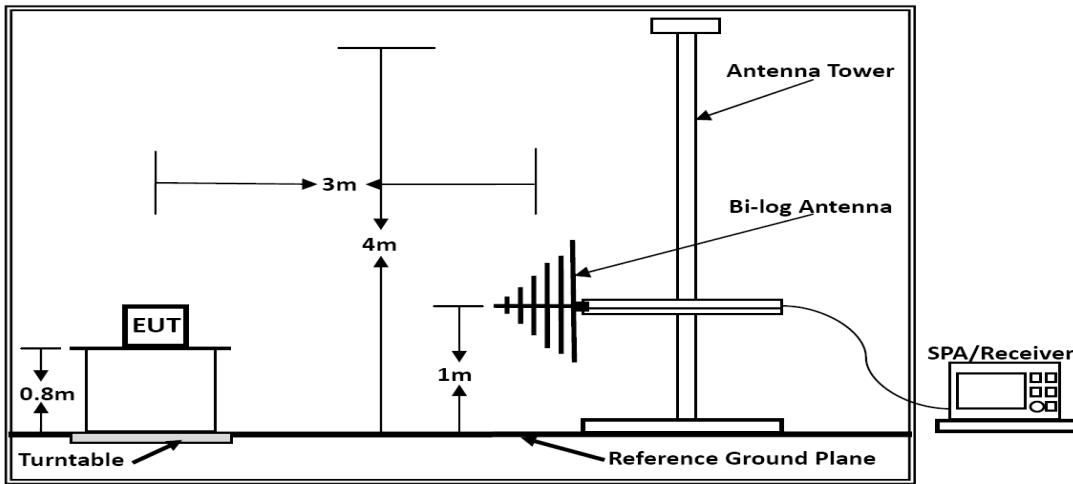
Below 1GHz
