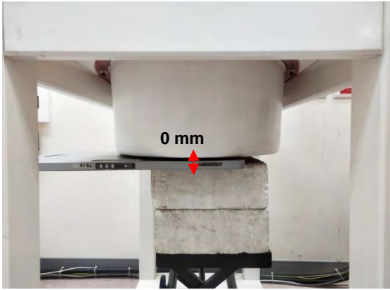
Fig.6 EUT Back side (Aux) to flat phantom
