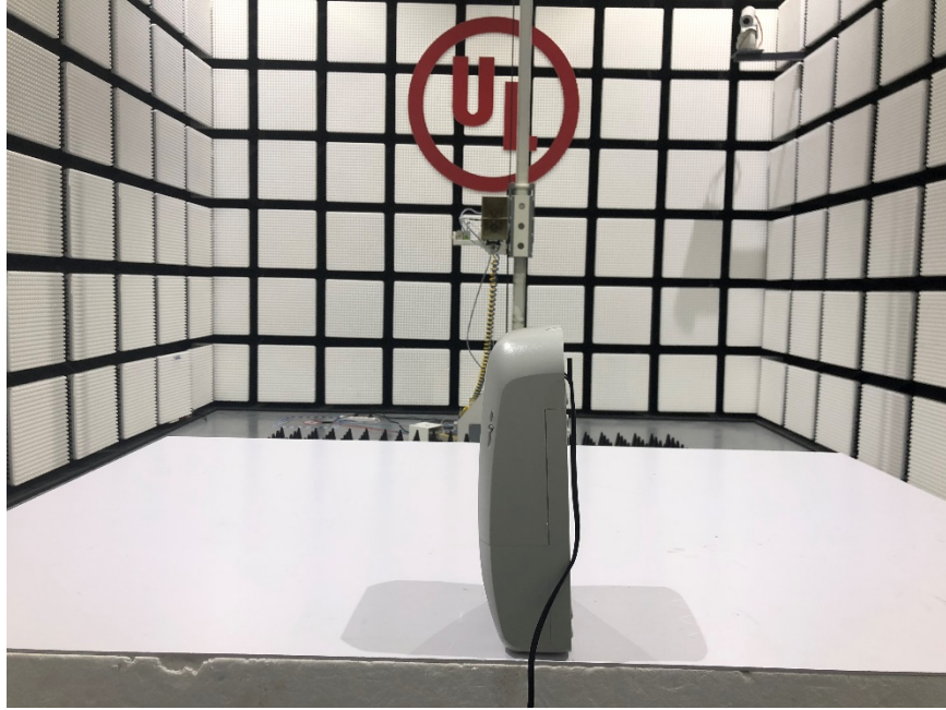
MEASUREMENT POSITION OF WCDMA Band 5 (Y axis)
